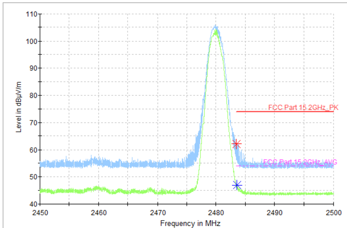
Fig.63. Frequency Band Edges: 8DPSK, Channel 78, 2.45 GHz - 2.50GHz
