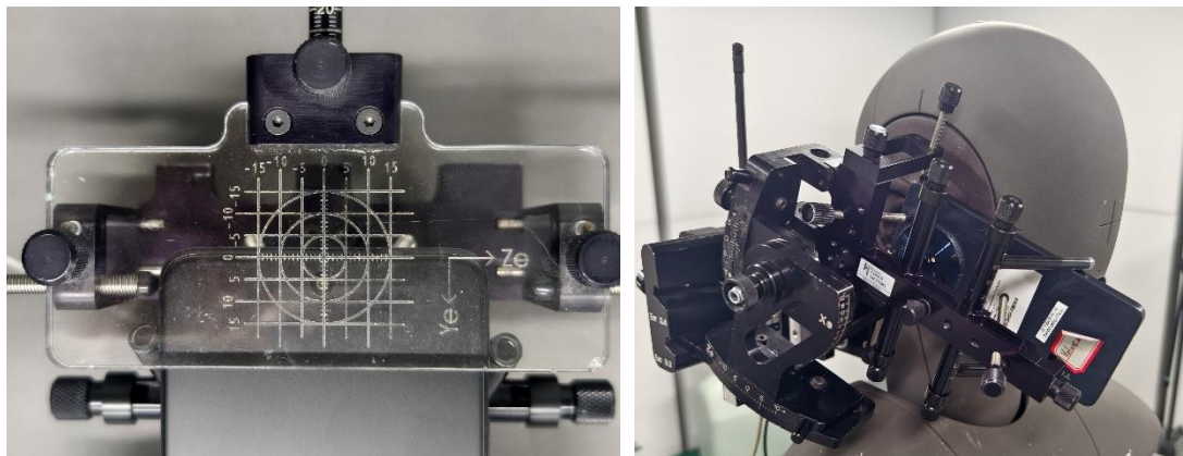
Pic 3: Handset Positioner (HHPIII) with mounted EUT mobile phone
