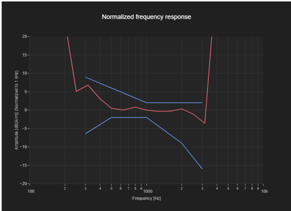
Figure C.1 Frequency Response of NR B7-N77
