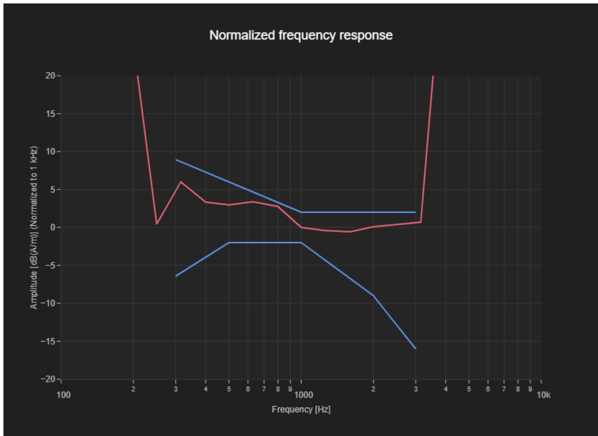
Figure C.2 Frequency Response of NR B26-N77-OTT
