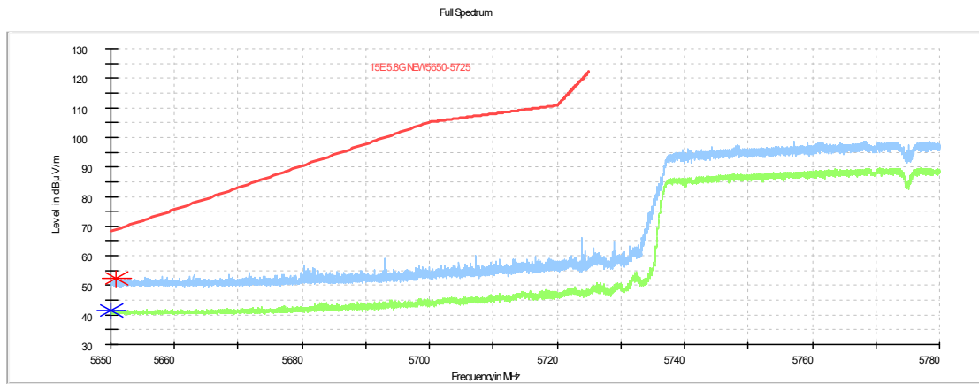
Fig. 11 Band Edges (802.11ac-HT80 Ch155, 5775MHz)
