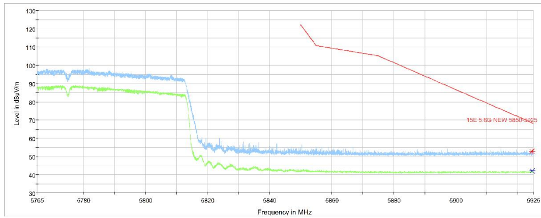
Fig. 11 Band Edges (802.11ac-HT80 Ch155, 5775MHz)
