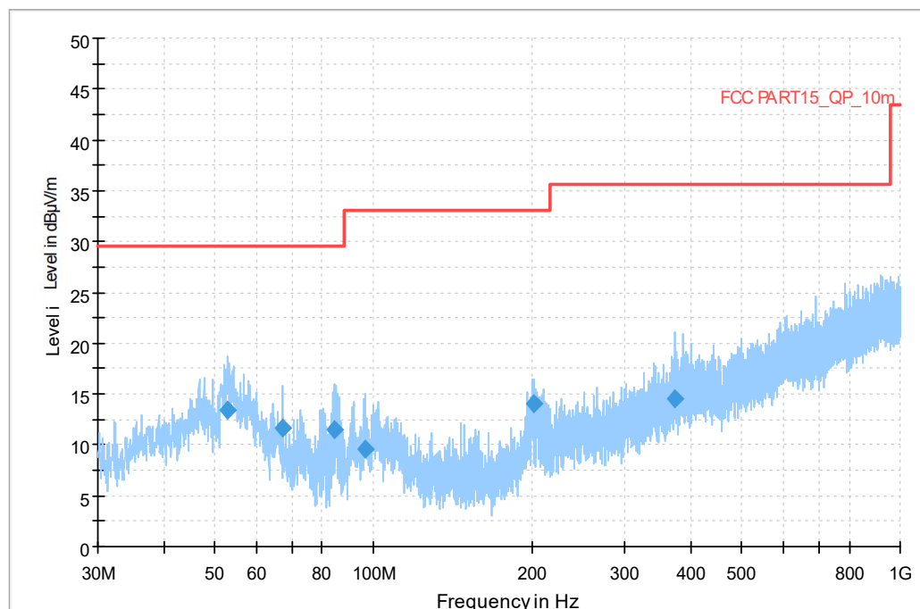
Figure B.11 Radiated Emission from 30MHz to 1GHz
