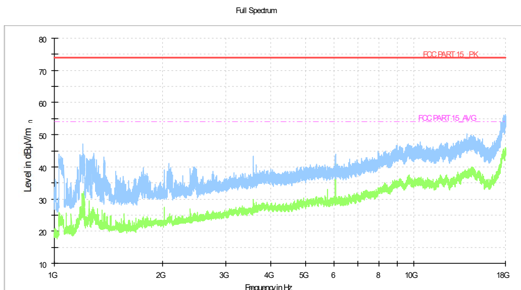
Figure B.6 Radiated Emission from 1GHz to 18GHz
