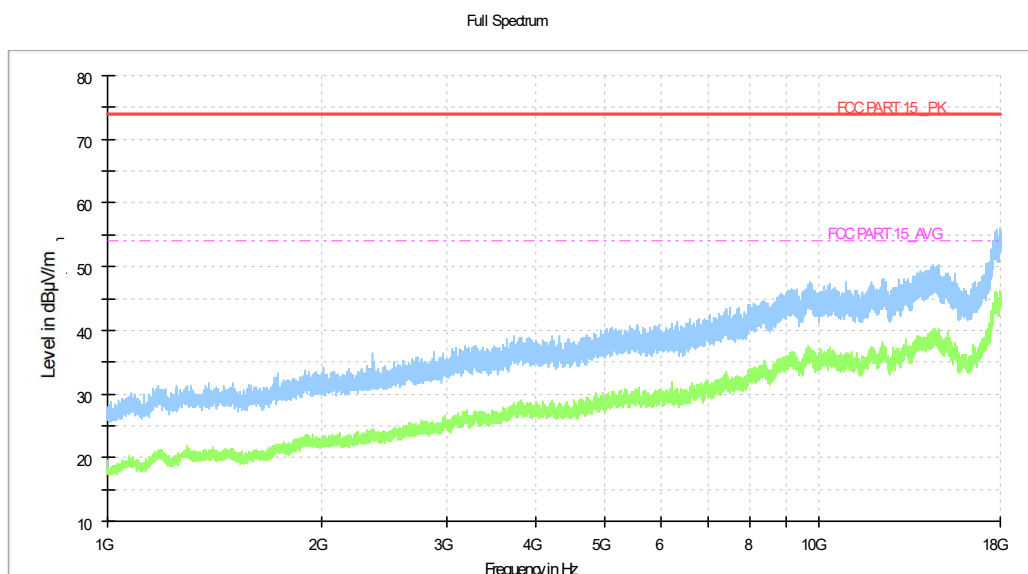
Figure B.2 Radiated Emission from 1GHz to 18GHz
