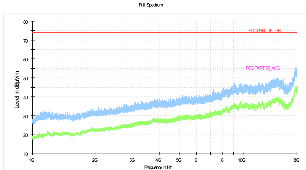
Figure B.4 Radiated Emission from 1GHz to 18GHz
