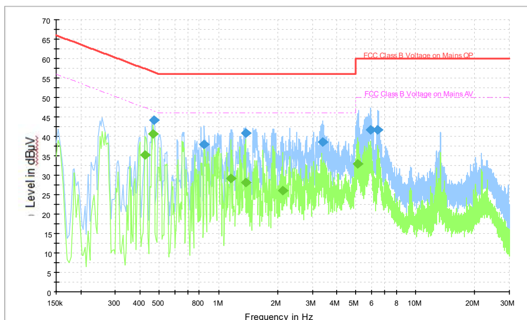
Figure B.15 Conducted Emission
