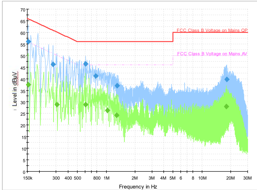
Figure B.17 Conducted Emission
