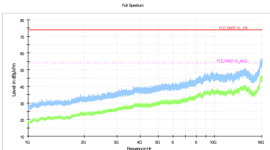
Figure B.10 Radiated Emission from 1GHz to 18GHz
