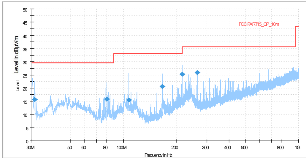
Figure B.7 Radiated Emission from 30MHz to 1GHz
