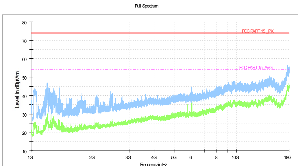
Figure B.8 Radiated Emission from 1GHz to 18GHz
