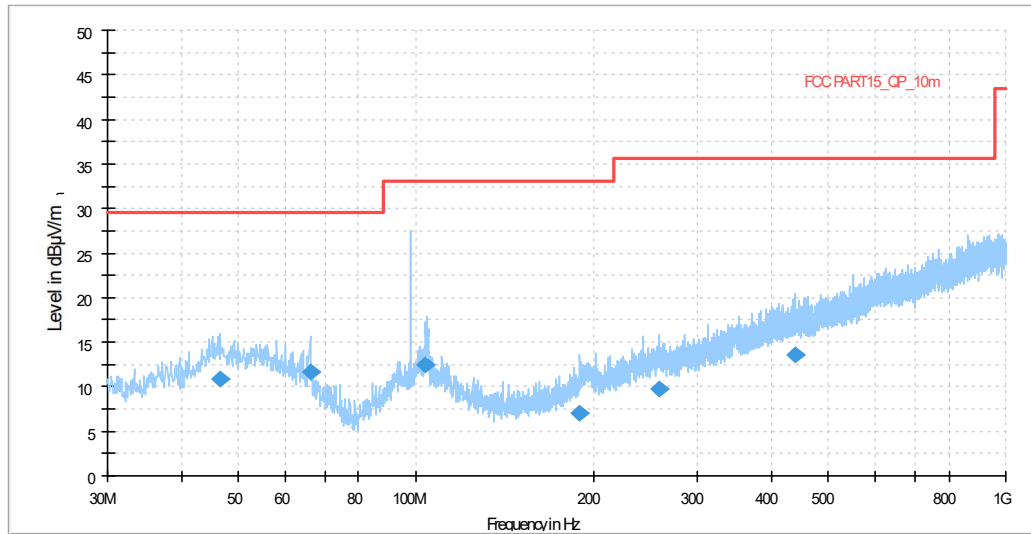
Figure B.9 Radiated Emission from 30MHz to 1GHz
