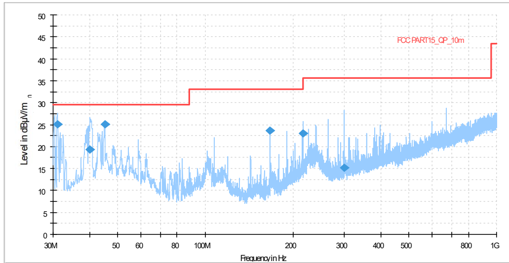
Figure B.5 Radiated Emission from 30MHz to 1GHz
