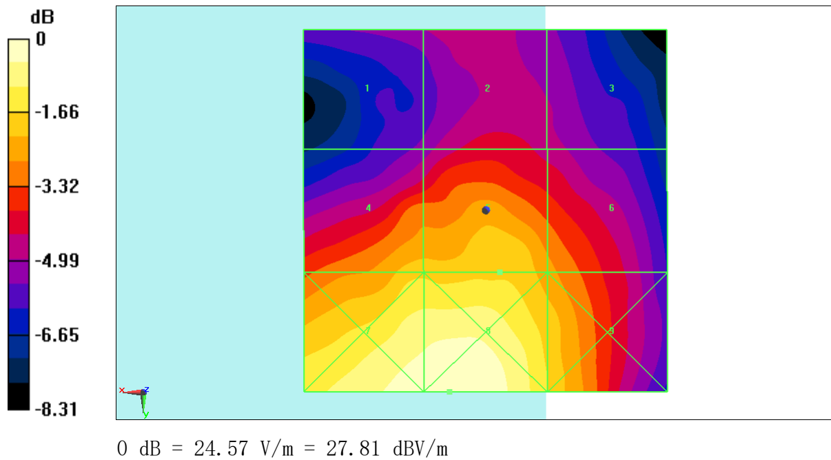
Fig B.3 HAC RF E-Field WiFi2.4G
