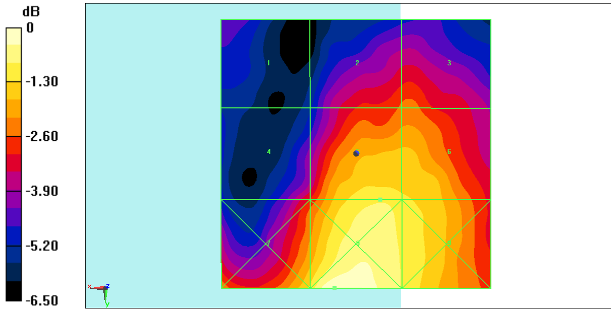
Fig B.1 HAC RF E-Field LTE Band41 PC2
