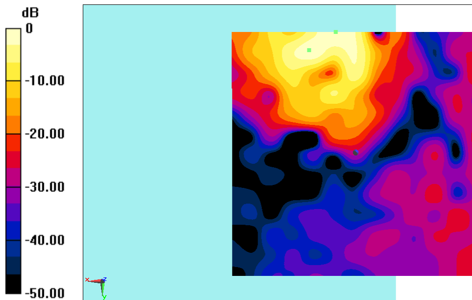
Fig B.1 T-Coil LTE Band41 PC2
