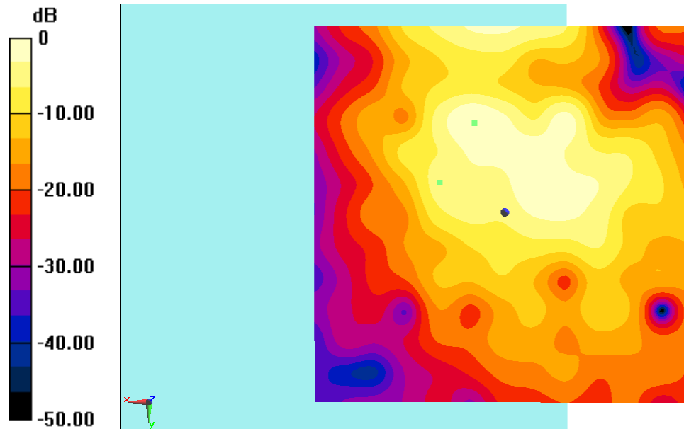
Fig B.2 T-Coil LTE Band41 PC2
