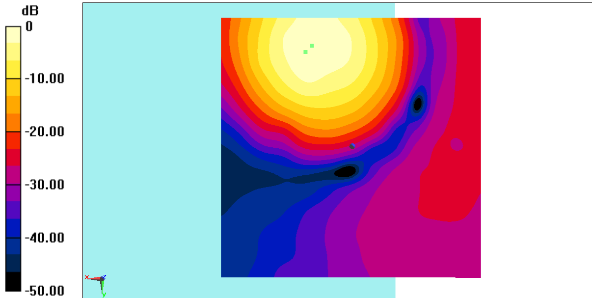
Fig B.3 T-Coil LTEB41 PC2-OTT
