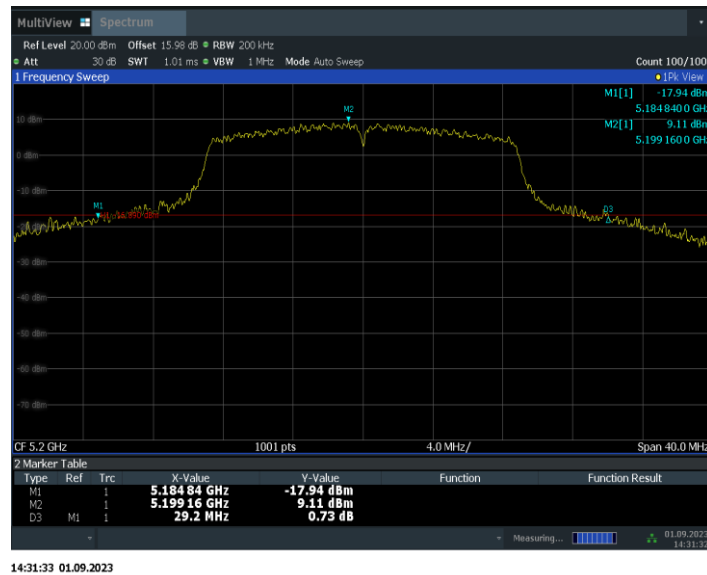
Fig.12 26dB Emission Bandwidth (802.11ac-VHT20, 5200MHz)
