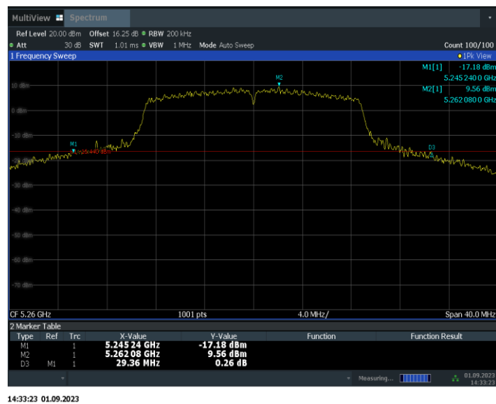
Fig.14 26dB Emission Bandwidth (802.11ac-VHT20, 5260MHz)
