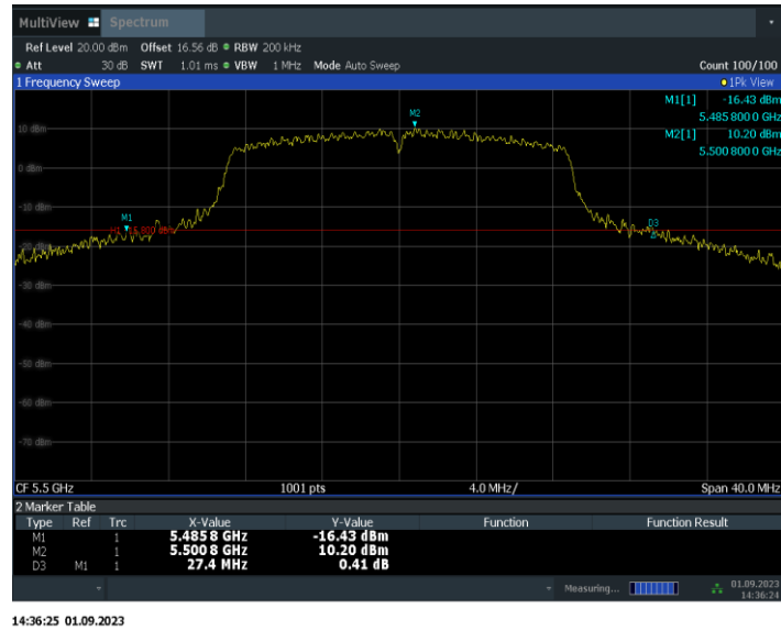
Fig.17 26dB Emission Bandwidth (802. 11ac-VHT20, 5500MHz)
