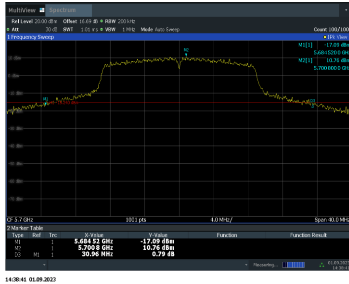
Fig.19 26dB Emission Bandwidth (802. 11ac-VHT20, 5700MHz)
