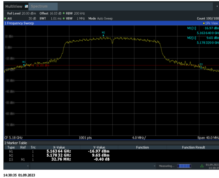
Fig.11 26dB Emission Bandwidth (802.11ac-VHT20, 5180MHz)
