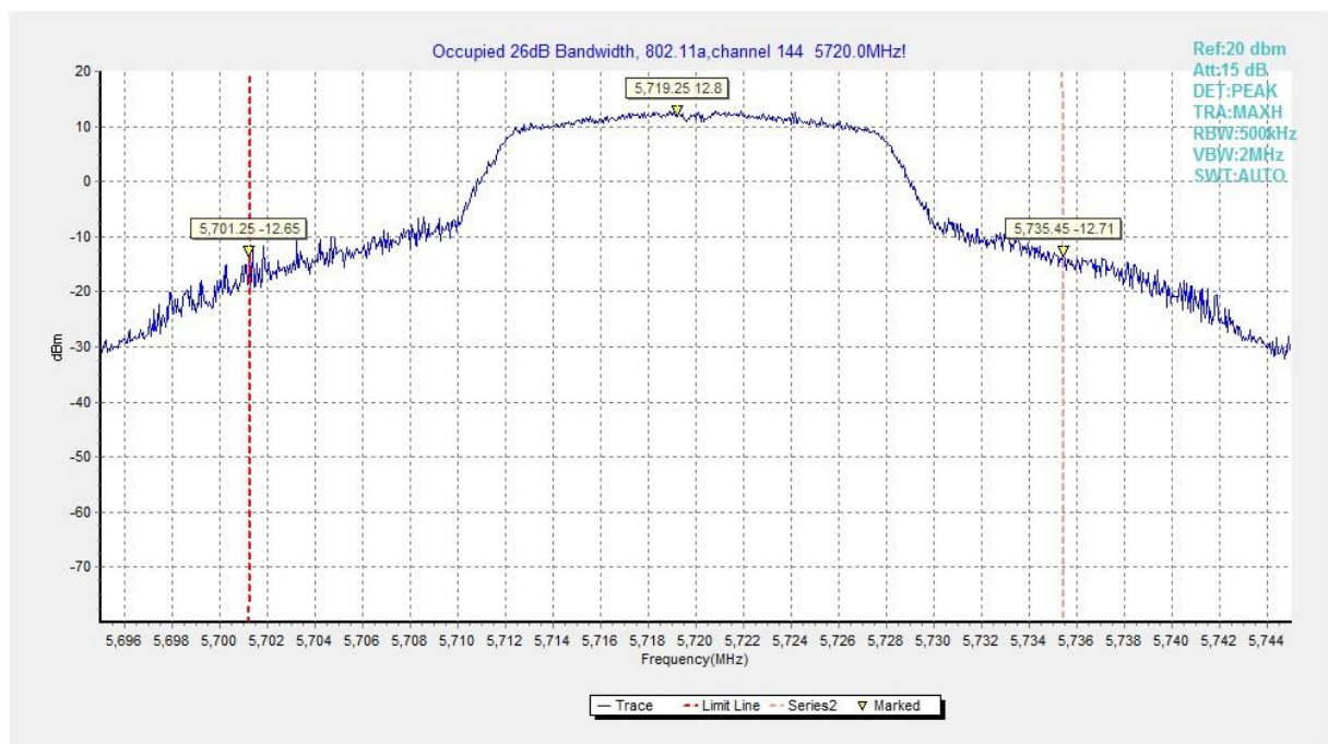
Fig.10 26dB Emission Bandwidth (802.11a, 5720MHz)
