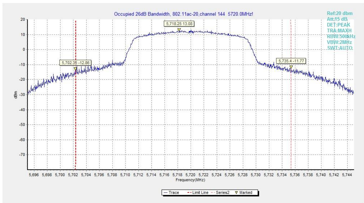
Fig.20 26dB Emission Bandwidth (802. 11ac-VHT20, 5720MHz)
