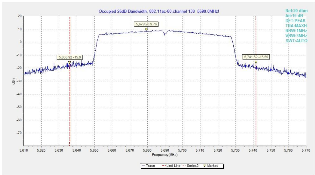
Fig.33 26dB Emission Bandwidth (802.11ac-VHT80, 5690MHz)
