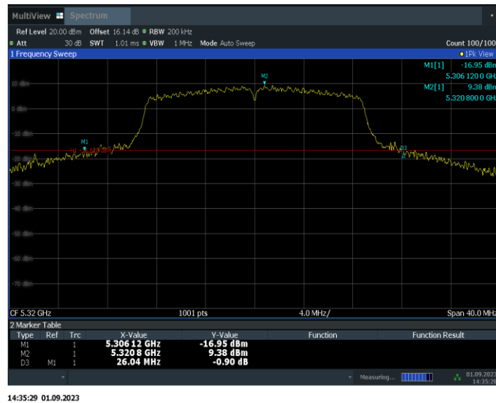
Fig.16 26dB Emission Bandwidth (802.11ac-VHT20, 5320MHz)
