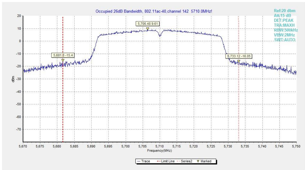
Fig.28 26dB Emission Bandwidth (802. 11ac-VHT40, 5710MHz)
