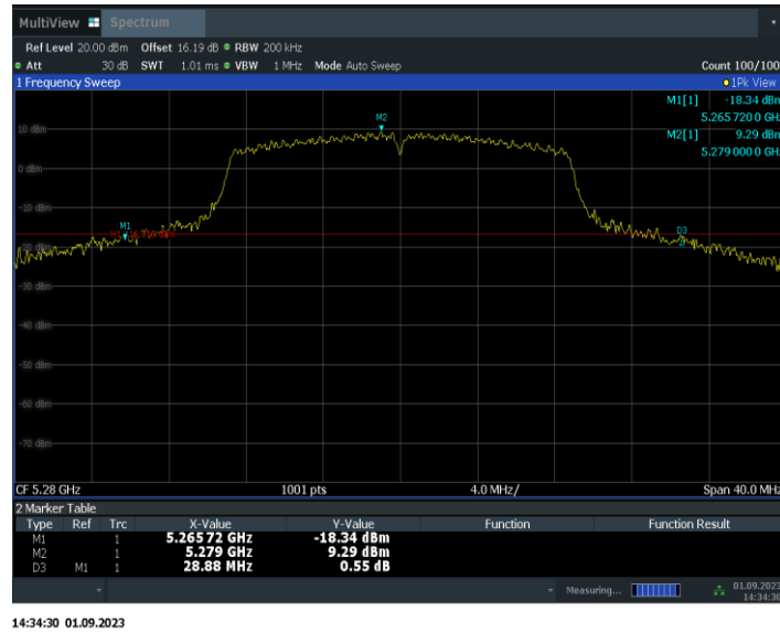
Fig.15 26dB Emission Bandwidth (802.11ac-VHT20, 5280MHz)
