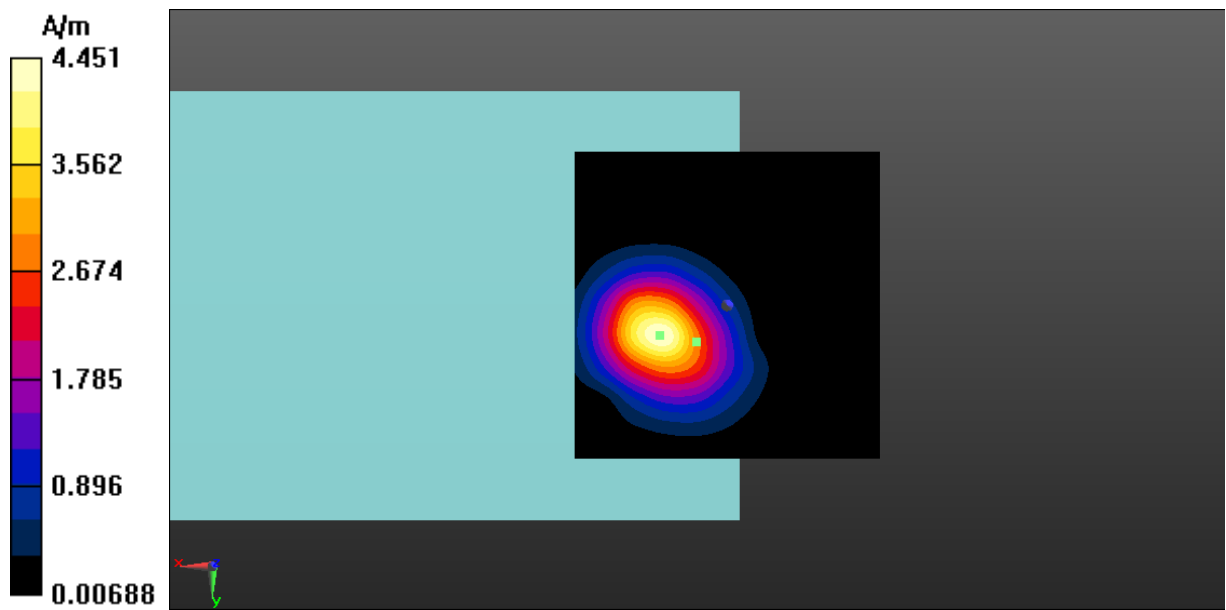
Fig A.19 T-Coil LTE-Band 25-Z
