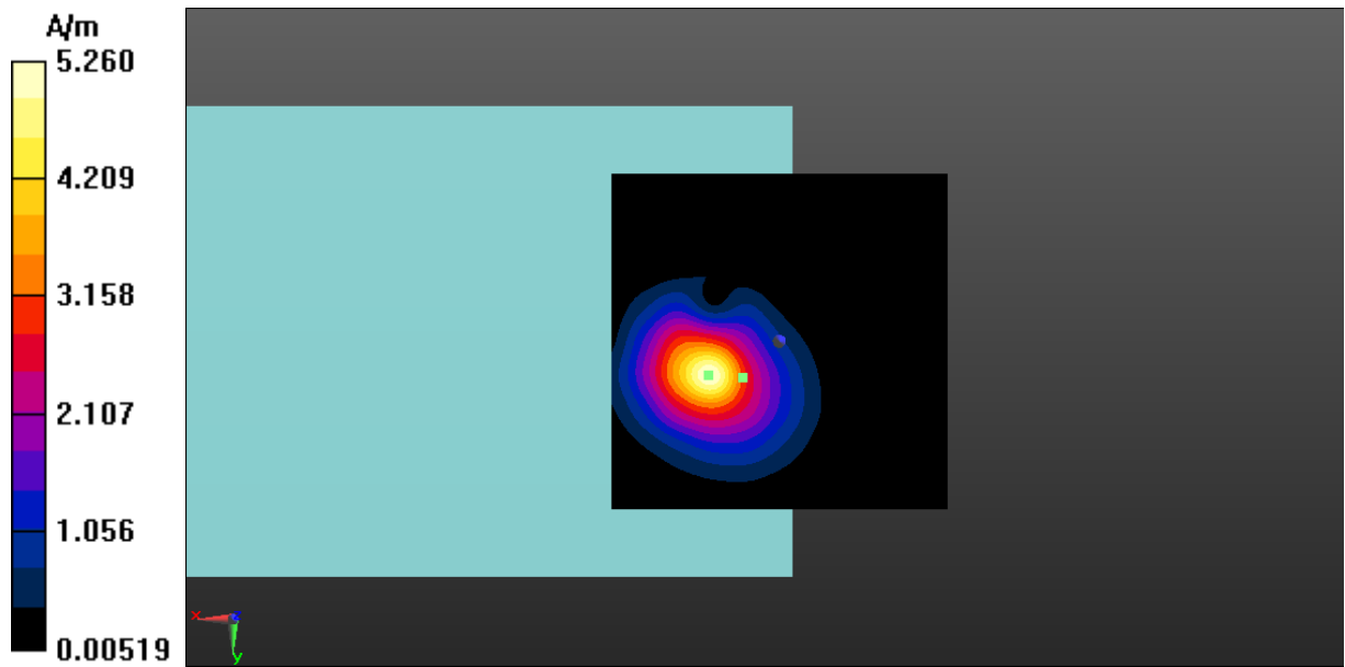
Fig A.22 T-Coil LTE-Band 66-Z
