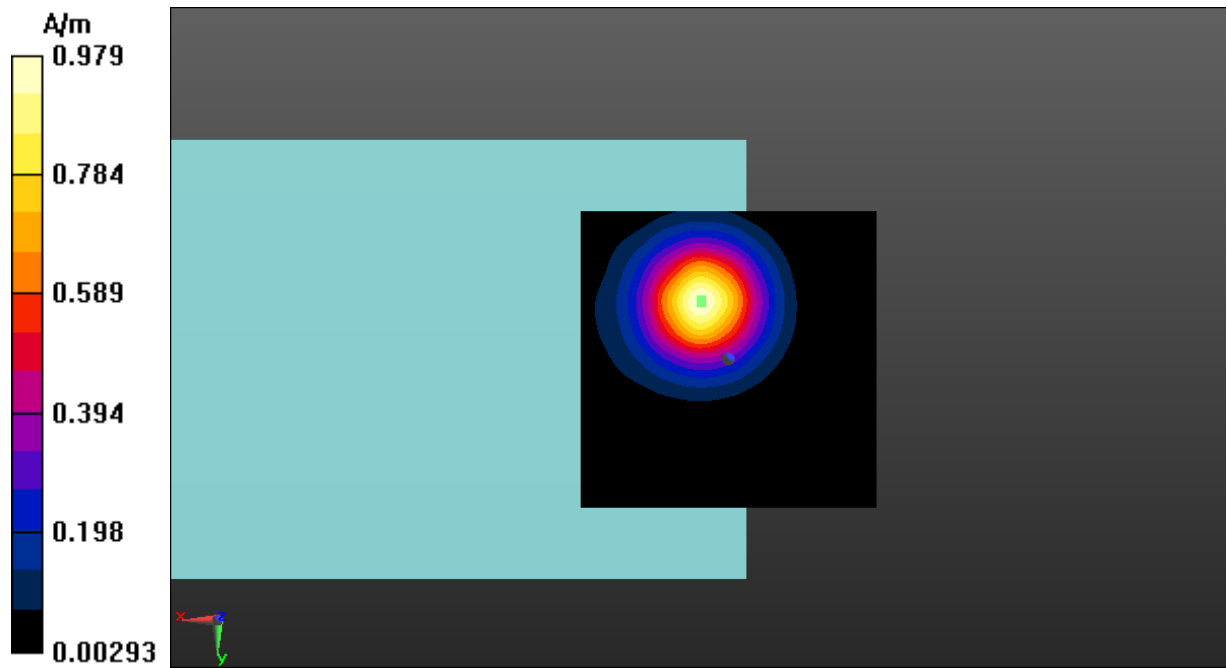
Fig A.7 T-Coil LTE-Band 25-Z
