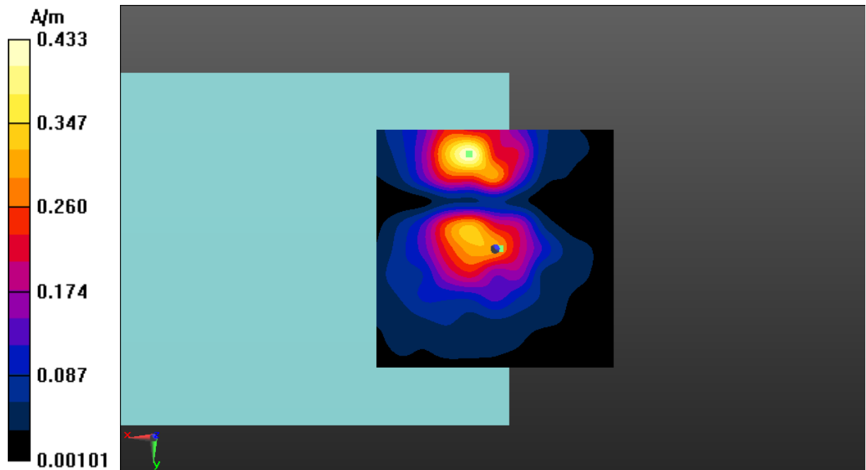
Fig A.5 T-Coil LTE-Band 12-Y
