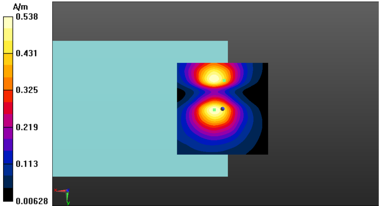
Fig A.21 T-Coil LTE-Band 41-Y
