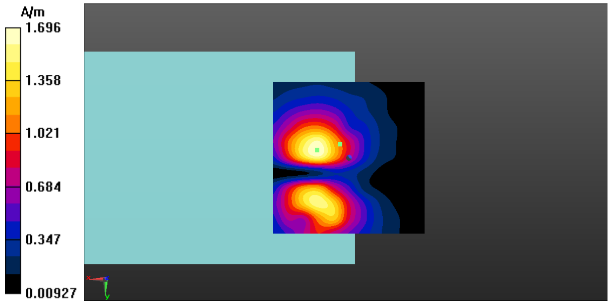
Fig A.23 T-Coil LTE-Band 71-Y
