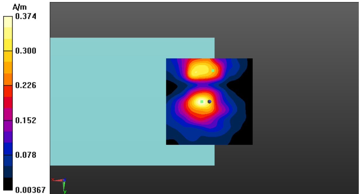
Fig A.14 T-Coil WLAN 5.3GHz-Y
