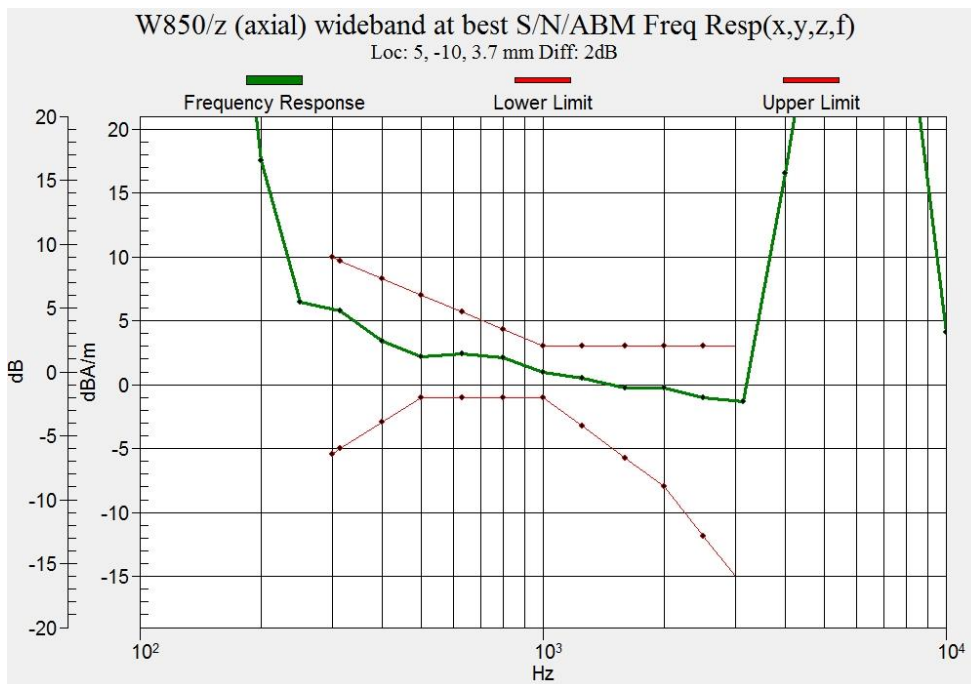
Figure B.17 Frequency Response of WCDMA Band 5 (Google Duo)
