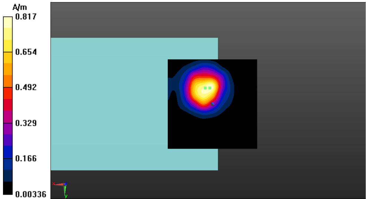
Fig A.6 T-Coil LTE-Band 13-Z
