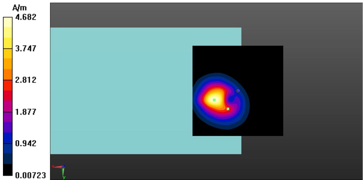
Fig A.23 T-Coil LTE-Band 71-Z
