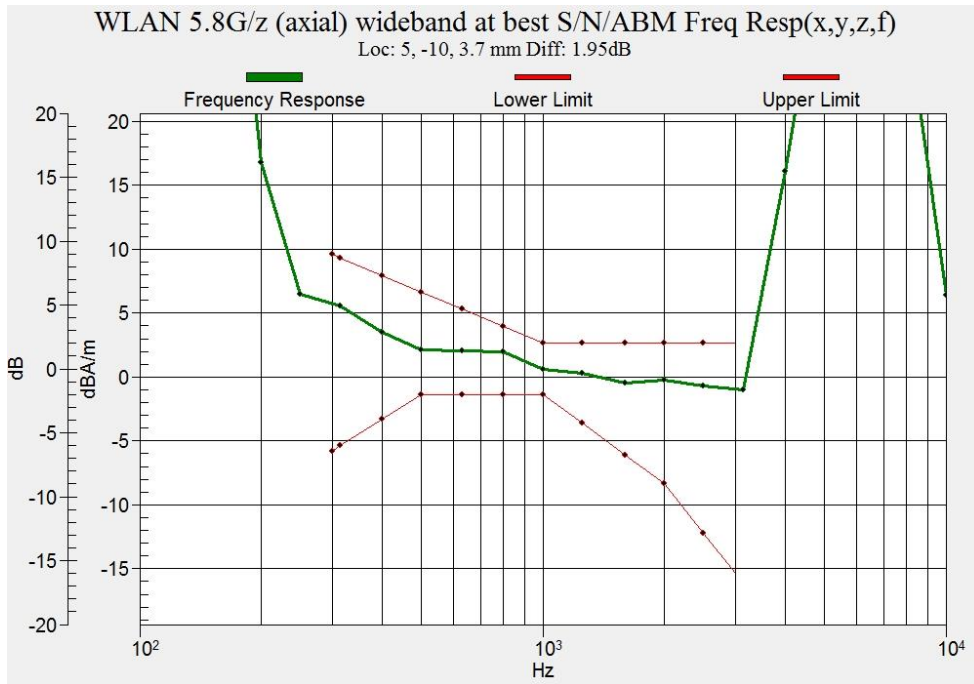
Figure B.25 Frequency Response of WLAN 5.8GHz (Google Duo)
