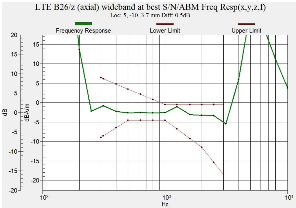
Figure B.8 Frequency Response of LTE Band 26
