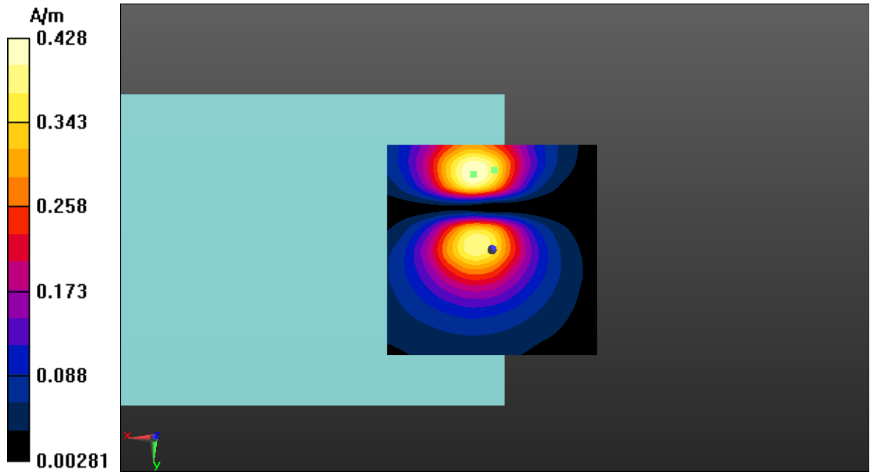
Fig A.10 T-Coil LTE-Band 71-Y
