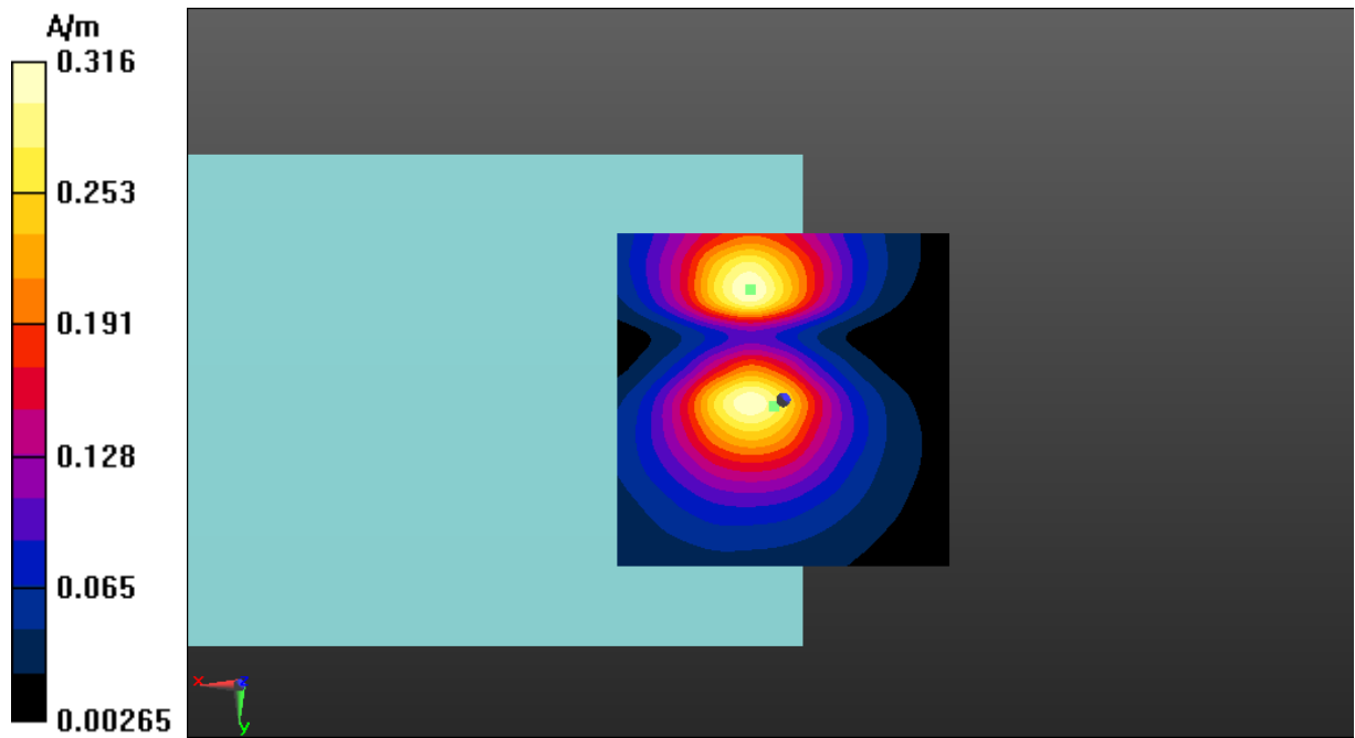
Fig A.2 T-Coil WCDMA Band 4-Y
