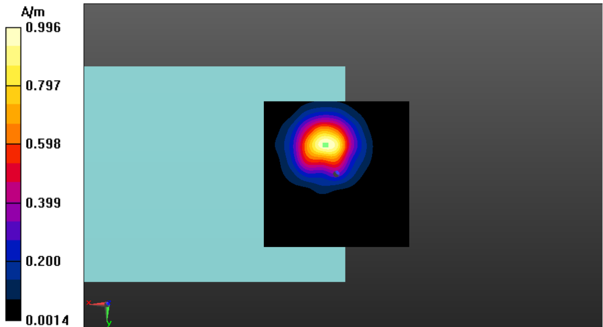
Fig A.16 T-Coil WLAN 5.8GHz-Z
