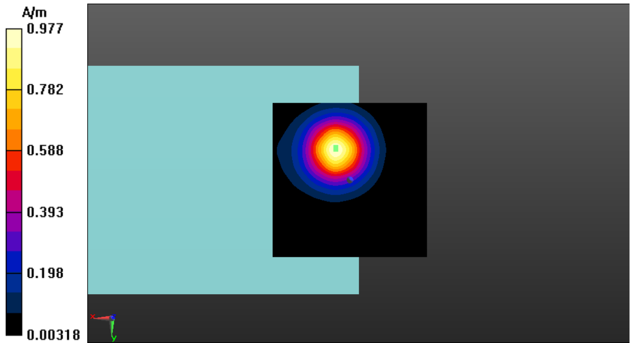
Fig A.10 T-Coil LTE-Band 71-Z
