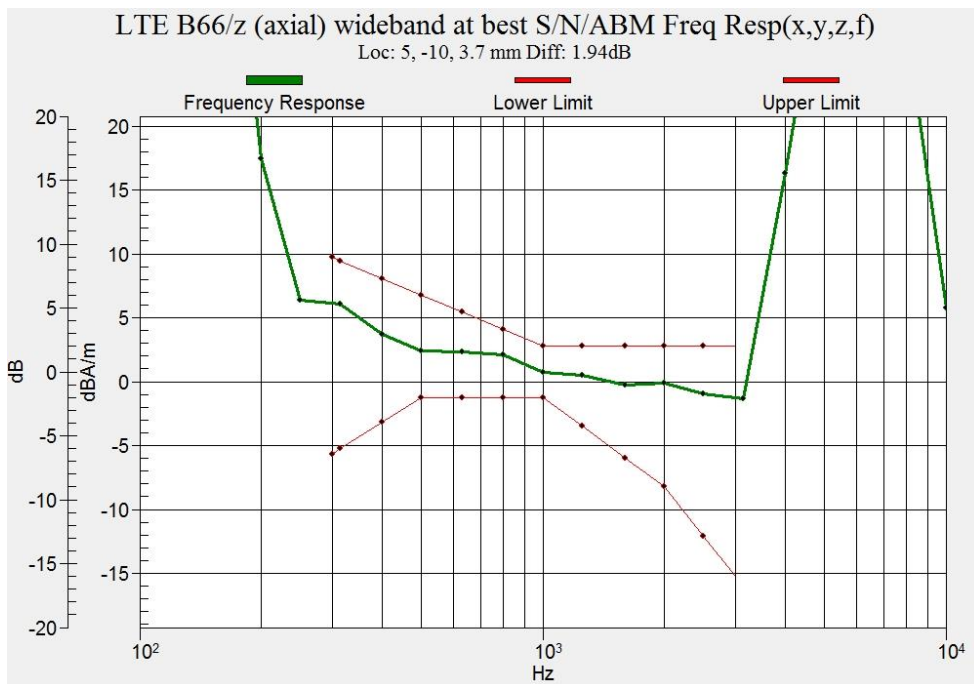
Figure B.22 Frequency Response of LTE Band 66 (Google Duo)
