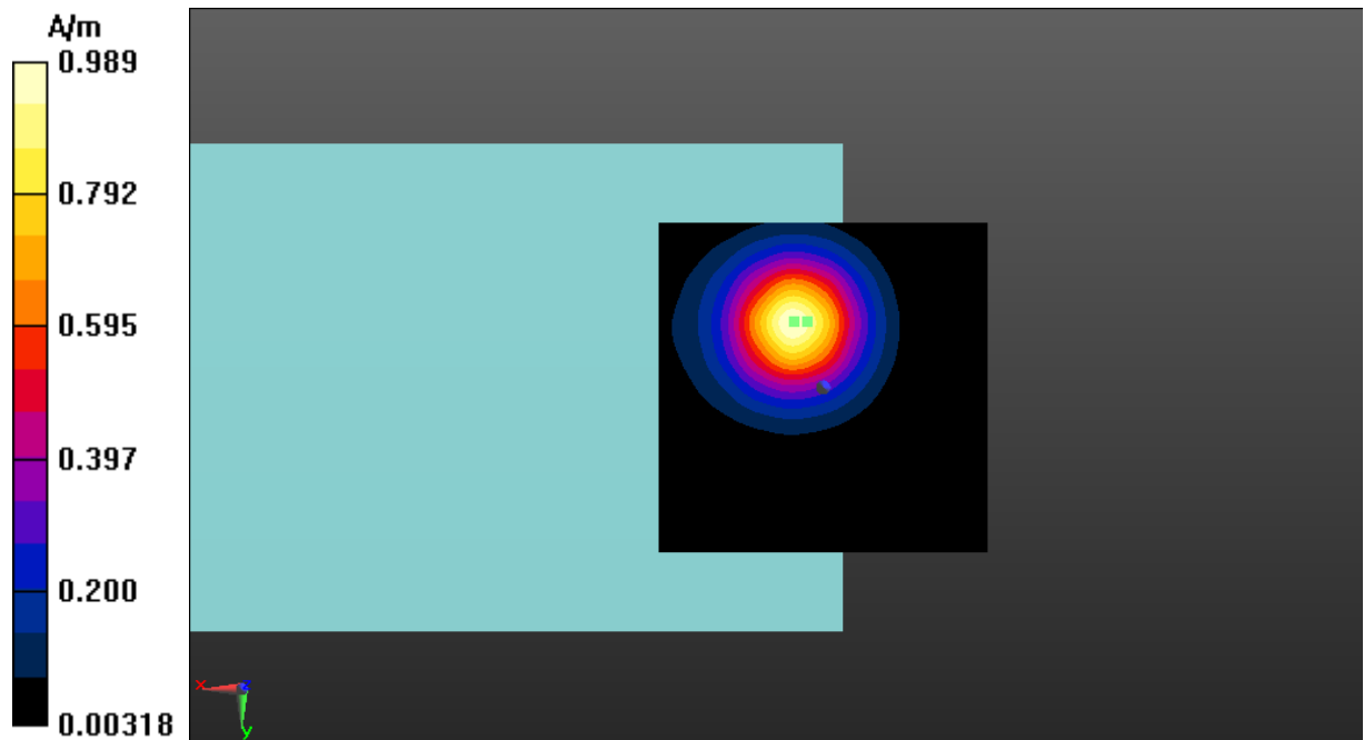
Fig A.9 T-Coil LTE-Band 66-Z
