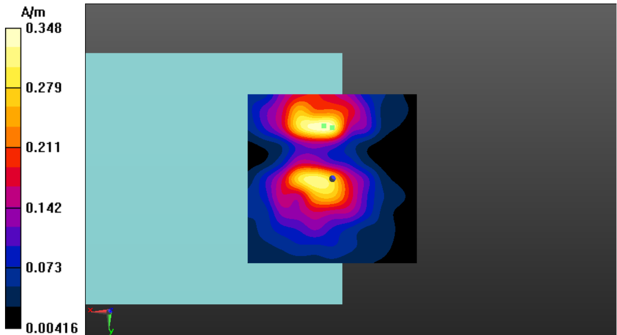
Fig A.6 T-Coil LTE-Band 13-Y
