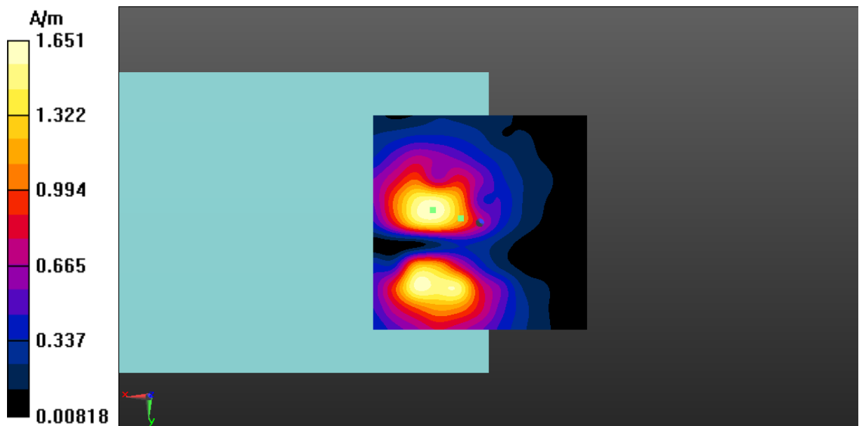
Fig A.22 T-Coil LTE-Band 66-Y
