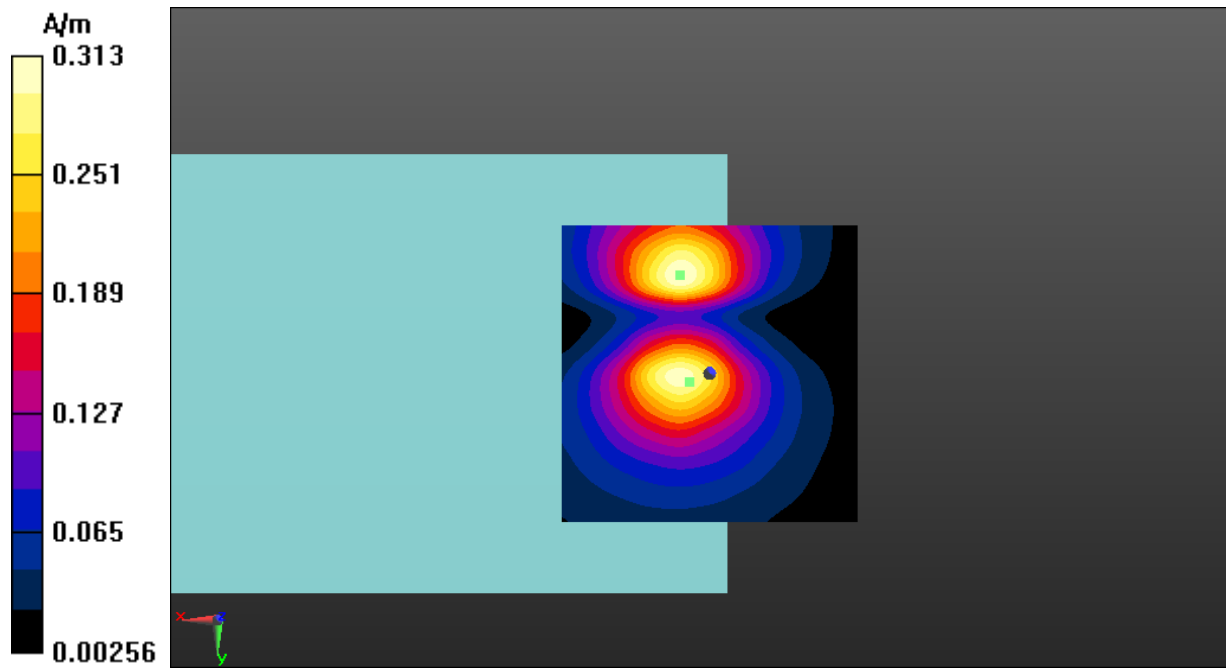
Fig A.3 T-Coil WCDMA Band 5-Y
