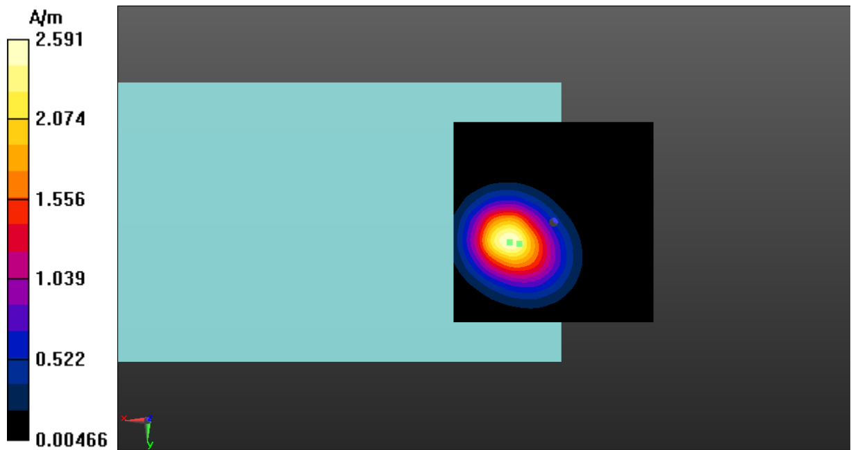
Fig A.18 T-Coil LTE-Band 7-Z
