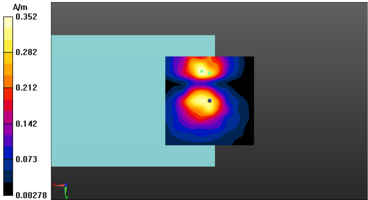
Fig A.16 T-Coil WLAN 5.8GHz-Y
