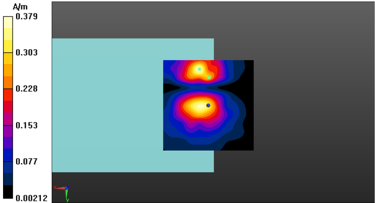
Fig A.12 T-Coil WLAN 2.4GHz-Y
