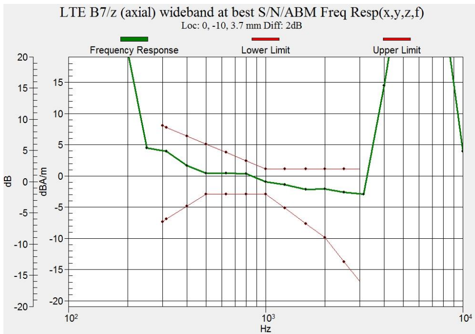
Figure B.18 Frequency Response of LTE Band 7 (Google Duo)
