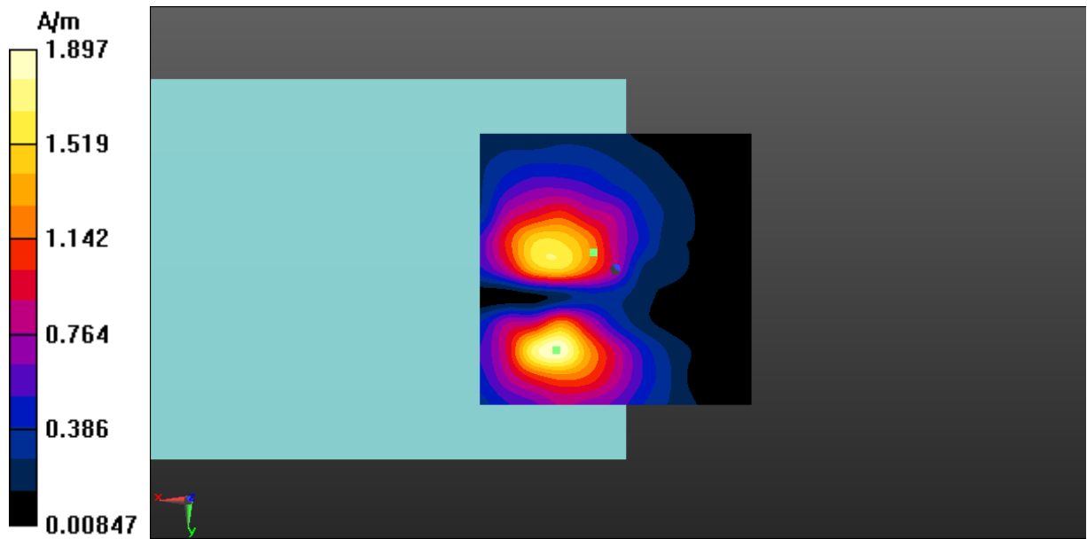
Fig A.19 T-Coil LTE-Band 25-Y
