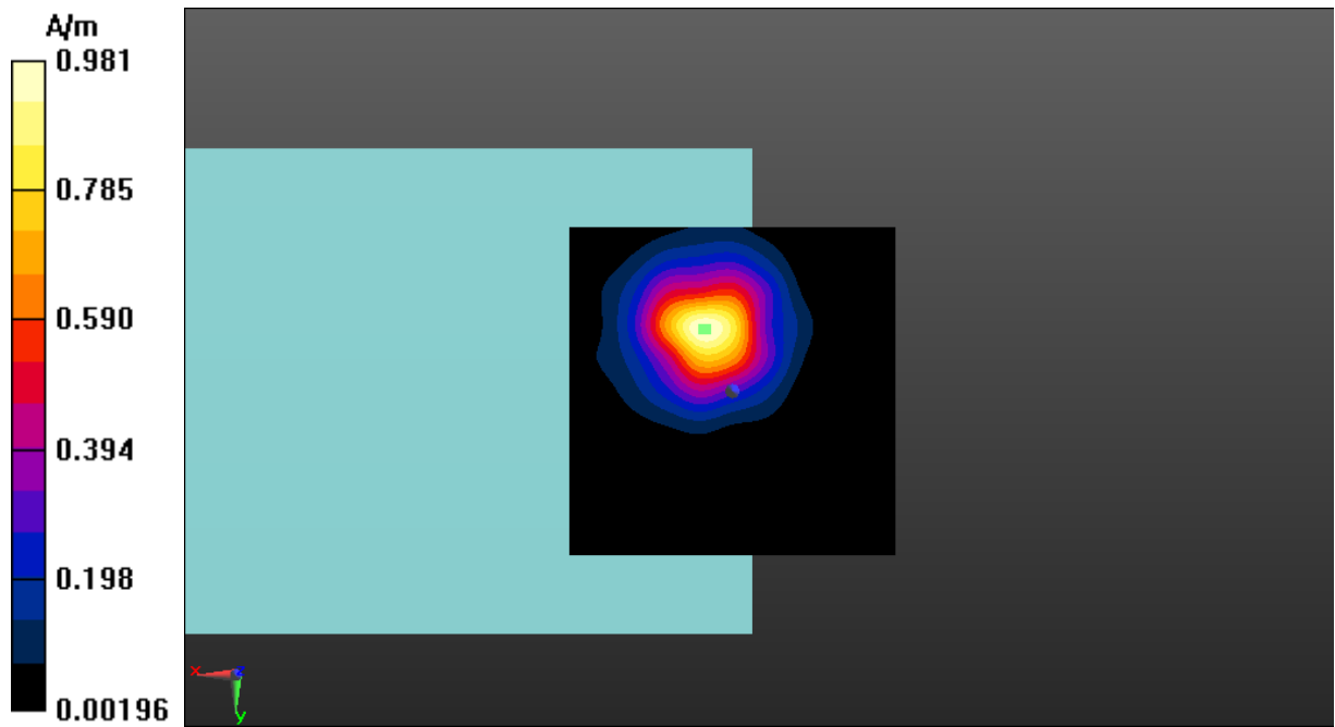
Fig A.15 T-Coil WLAN 5.5GHz-Z
