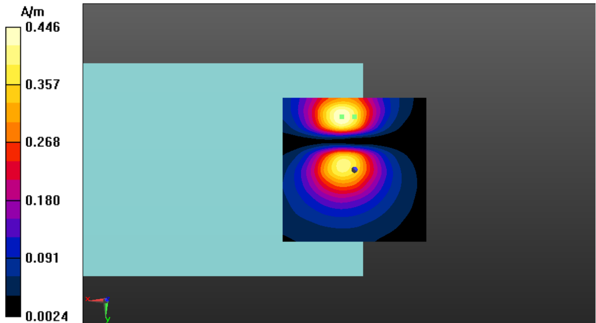
Fig A.11 T-Coil LTE-Band 41-Y
