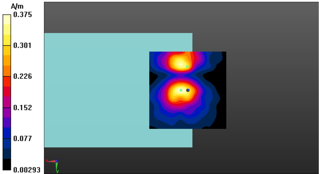
Fig A.15 T-Coil WLAN 5.5GHz-Y
