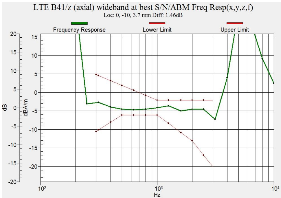
Figure B.9 Frequency Response of LTE Band 41
