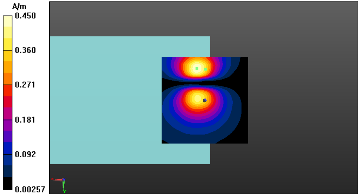
Fig A.8 T-Coil LTE-Band 26-Y
