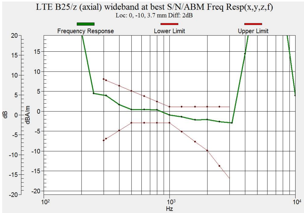
Figure B.18 Frequency Response of LTE Band 25 (Google Duo)
