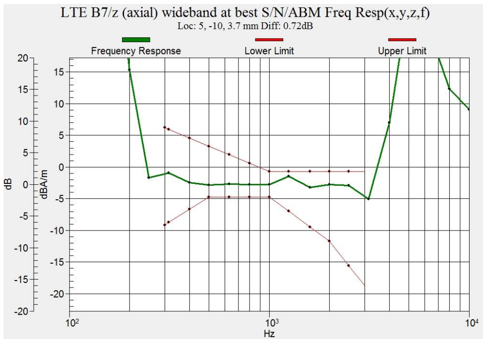
Figure B.4 Frequency Response of LTE Band 7
