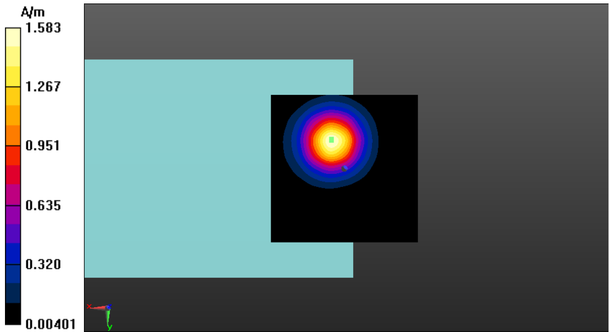
Fig A.25 T-Coil WLAN 5.8GHz-Z
