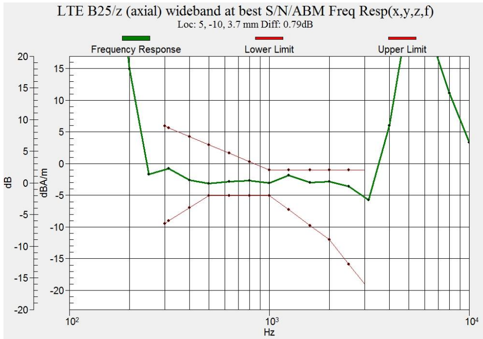
Figure B.7 Frequency Response of LTE Band 25
