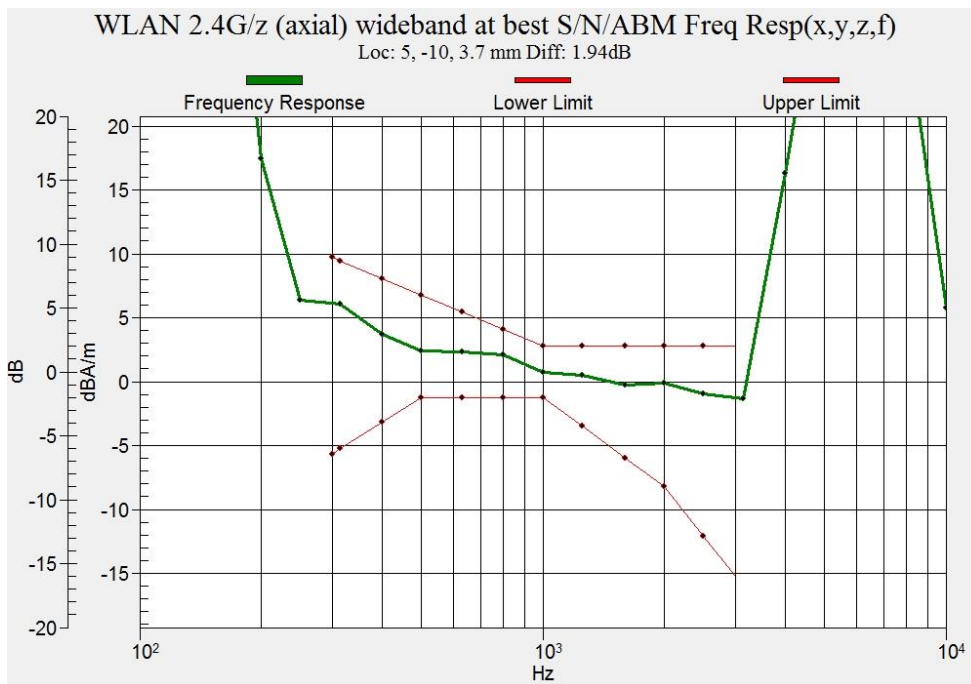
Figure B.24 Frequency Response of WLAN 2.4GHz (Google Duo)
