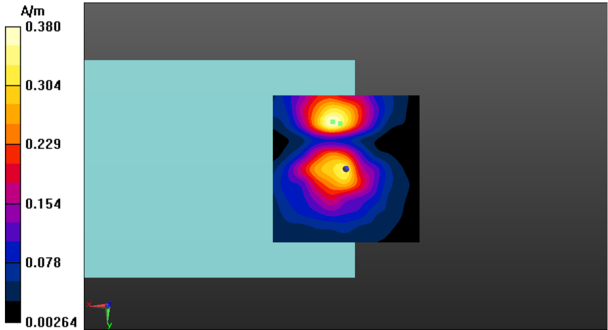
Fig A.13 T-Coil WLAN 5.2GHz-Y
