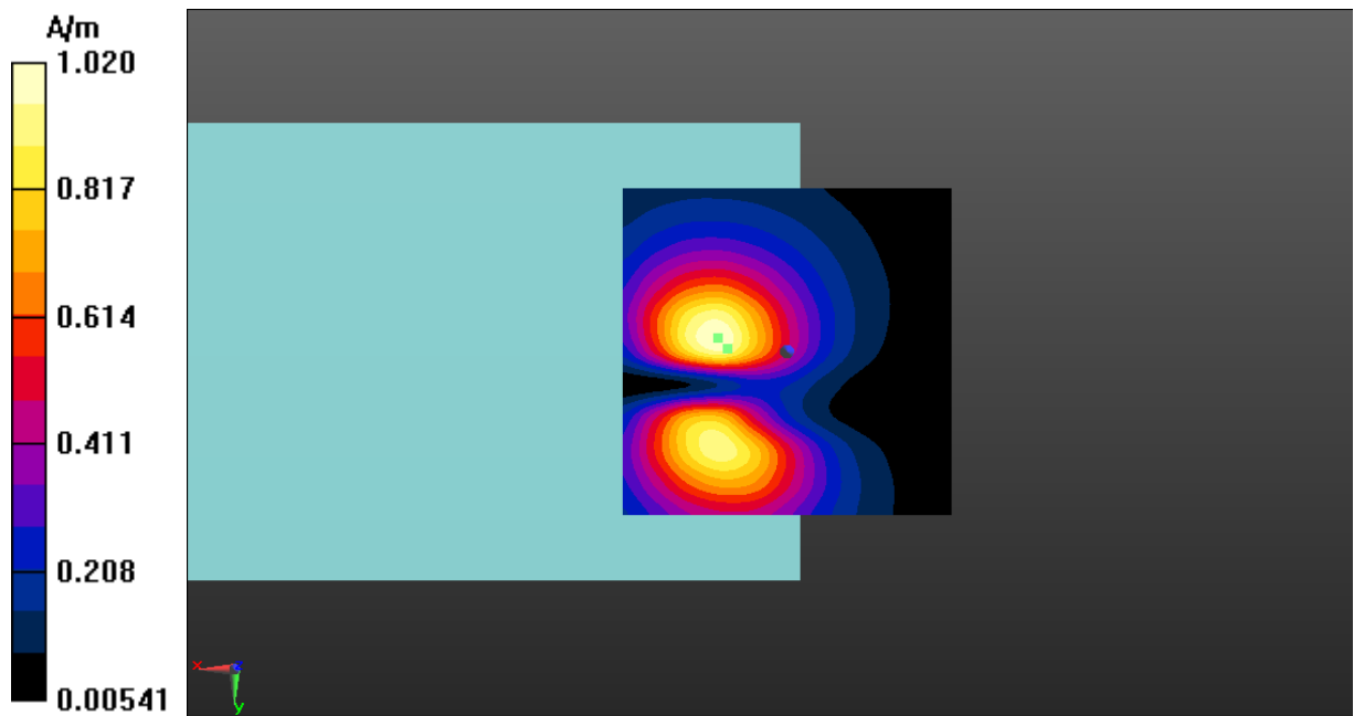
Fig A.18 T-Coil LTE-Band 7-Y
