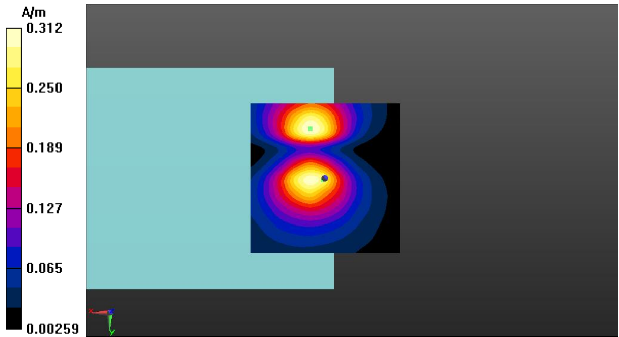
Fig A.1 T-Coil WCDMA Band 2-Y
