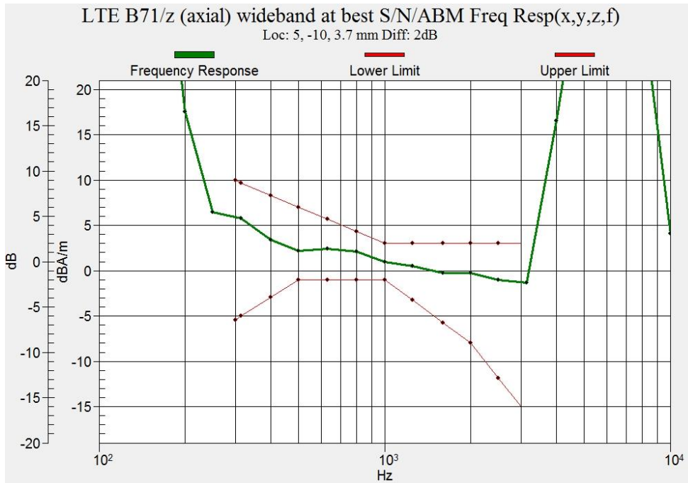
Figure B.23 Frequency Response of LTE Band 71 (Google Duo)
