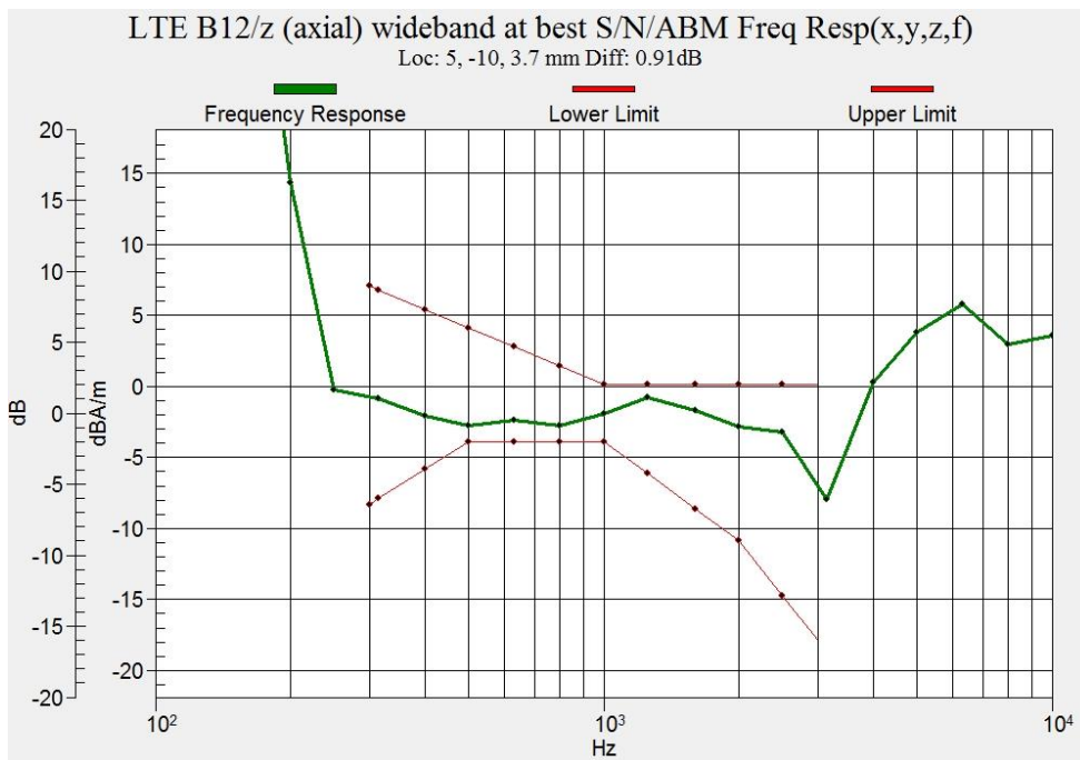
Figure B.5 Frequency Response of LTE Band 12
