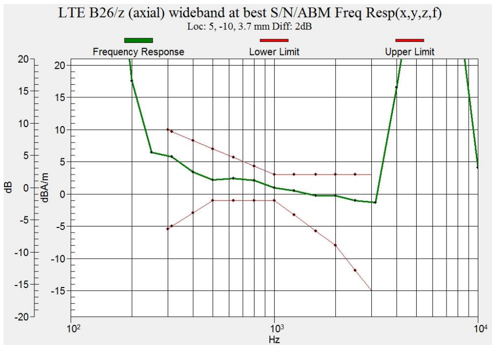
Figure B.18 Frequency Response of LTE Band 26 (Google Duo)
