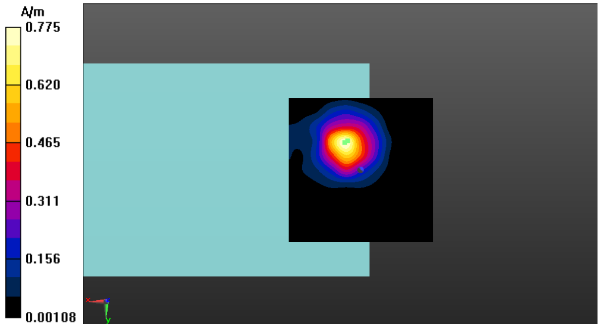
Fig A.5 T-Coil LTE-Band 12-Z
