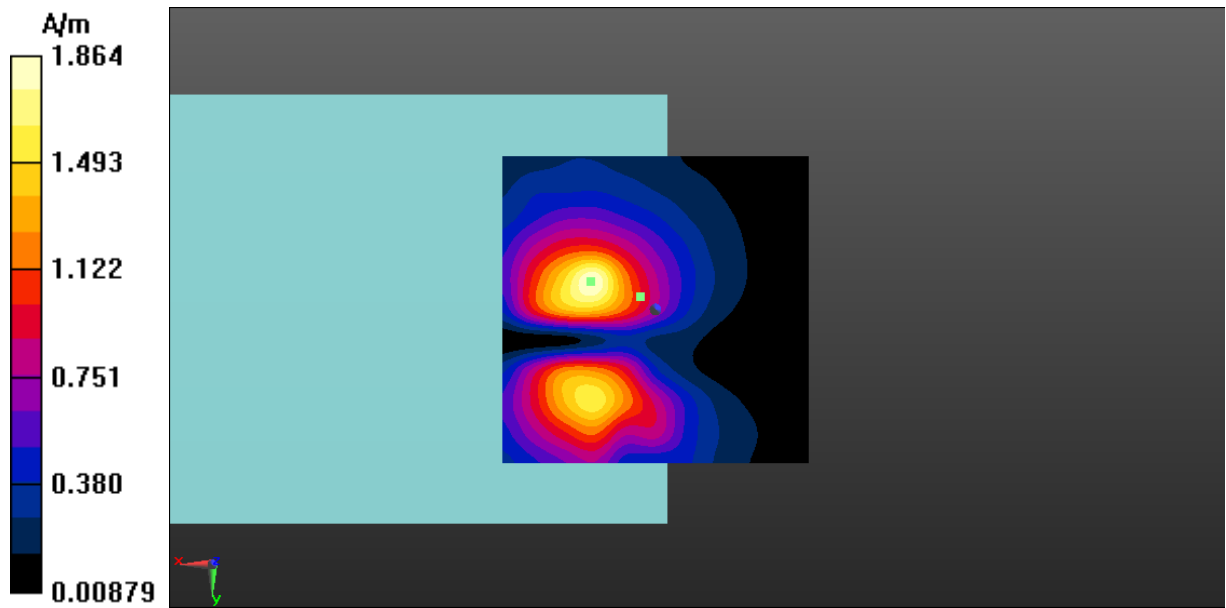
Fig A.20 T-Coil LTE-Band 26-Y
