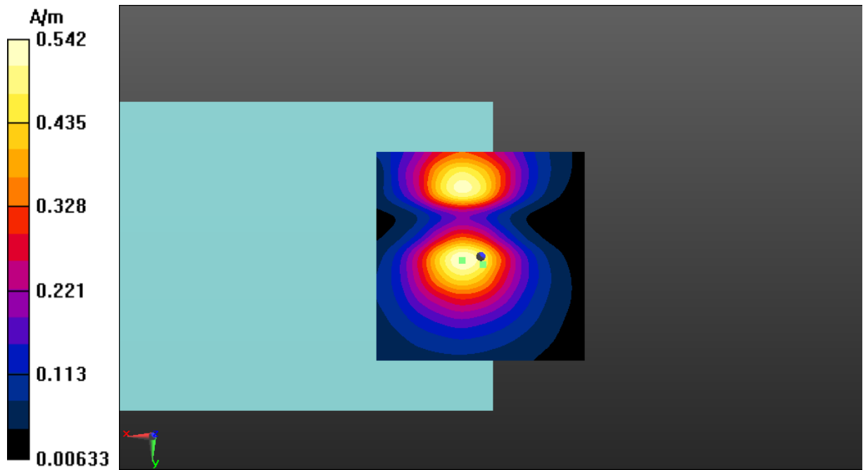
Fig A.17 T-Coil WCDMA Band 5-Y
