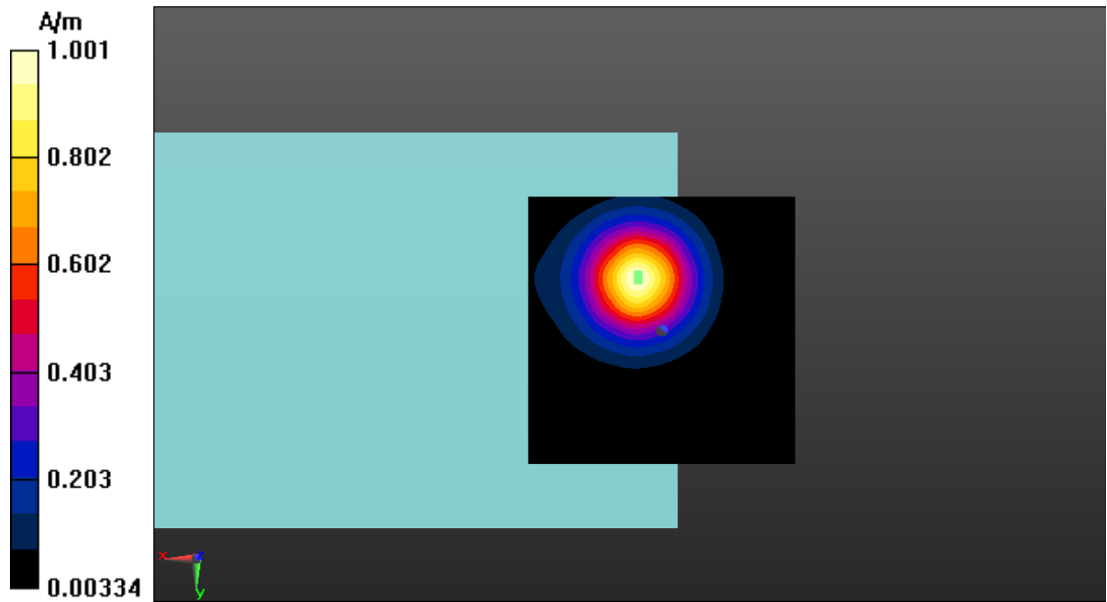
Fig A.8 T-Coil LTE-Band 26-Z
