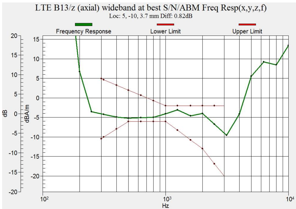
Figure B.6 Frequency Response of LTE Band 13
