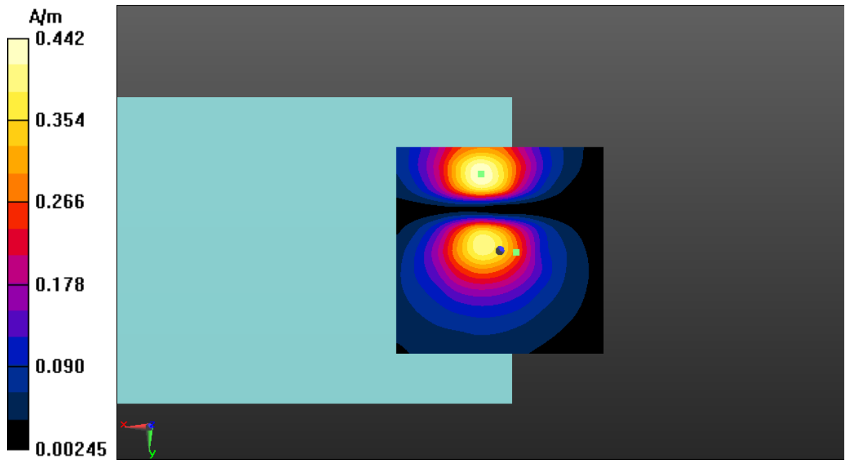
Fig A.4 T-Coil LTE-Band 7-Y
