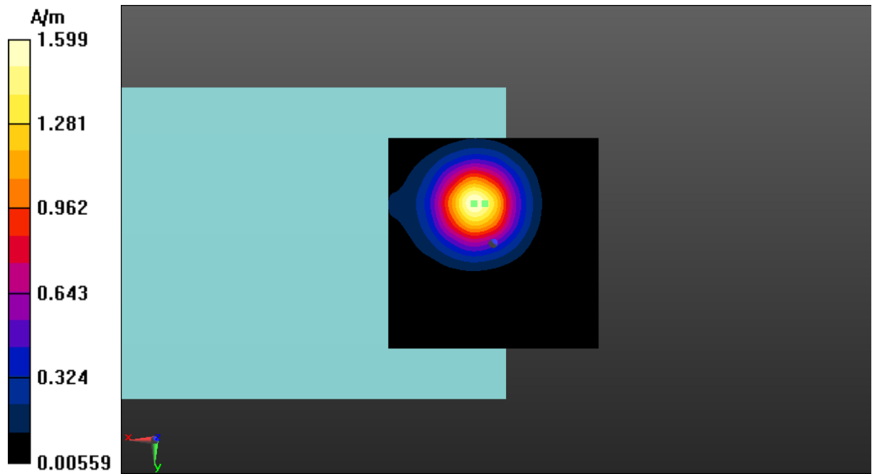
Fig A.21 T-Coil LTE-Band 41-Z
