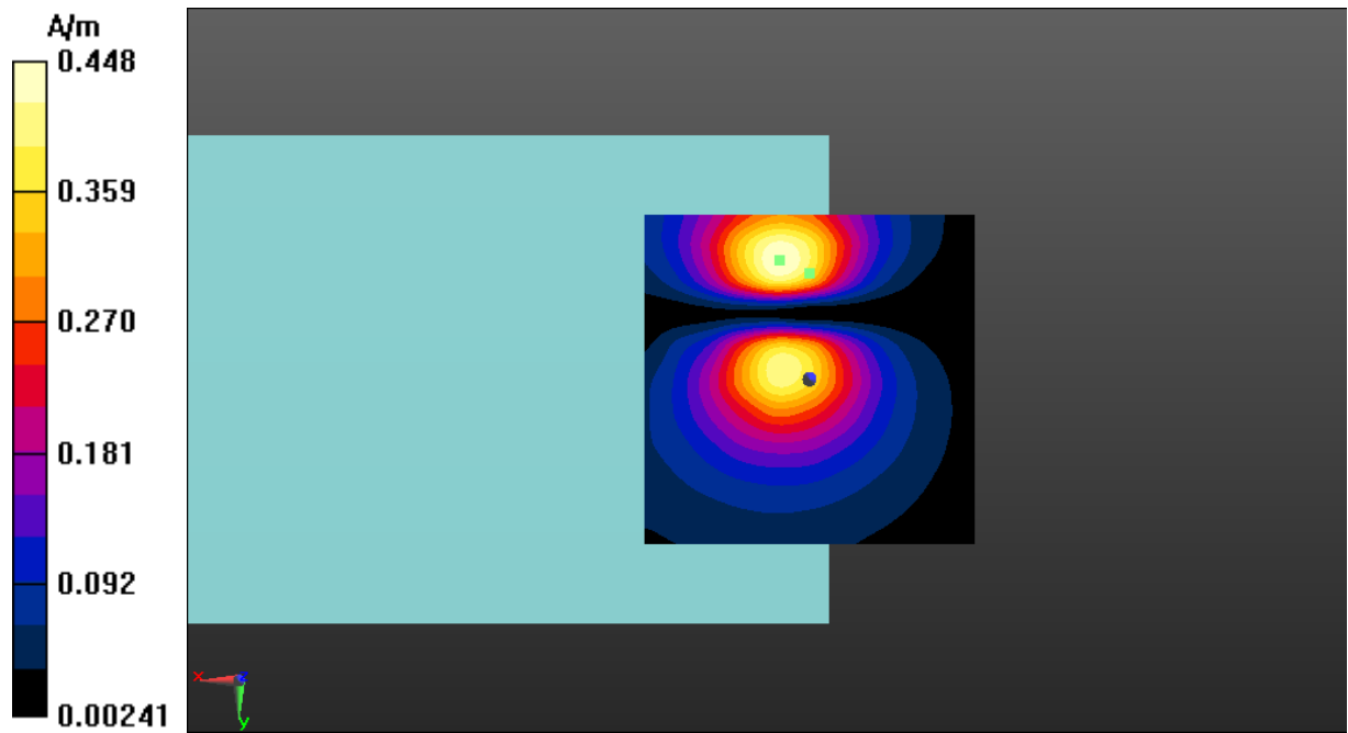
Fig A.9 T-Coil LTE-Band 66-Y
