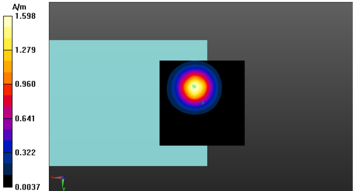
Fig A.17 T-Coil WCDMA Band 5-Z
