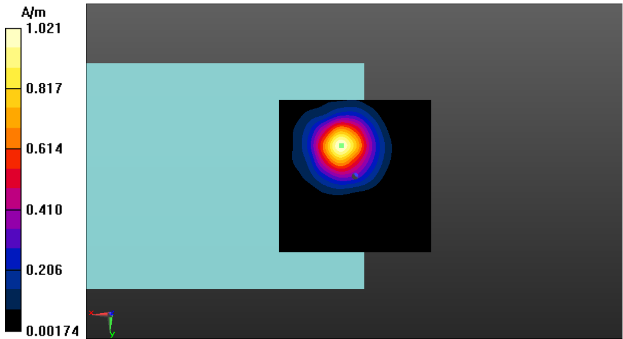
Fig A.13 T-Coil WLAN 5.2GHz-Z
