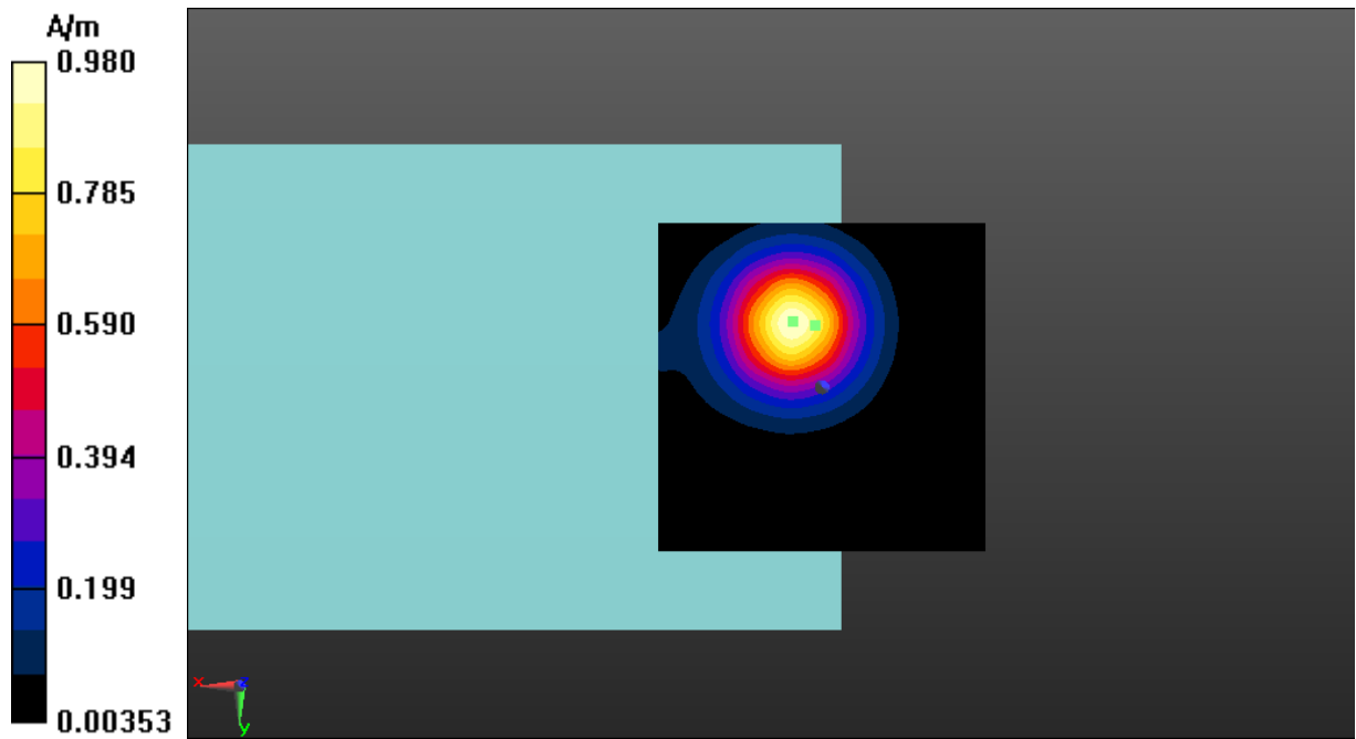
Fig A.11 T-Coil LTE-Band 41-Z
