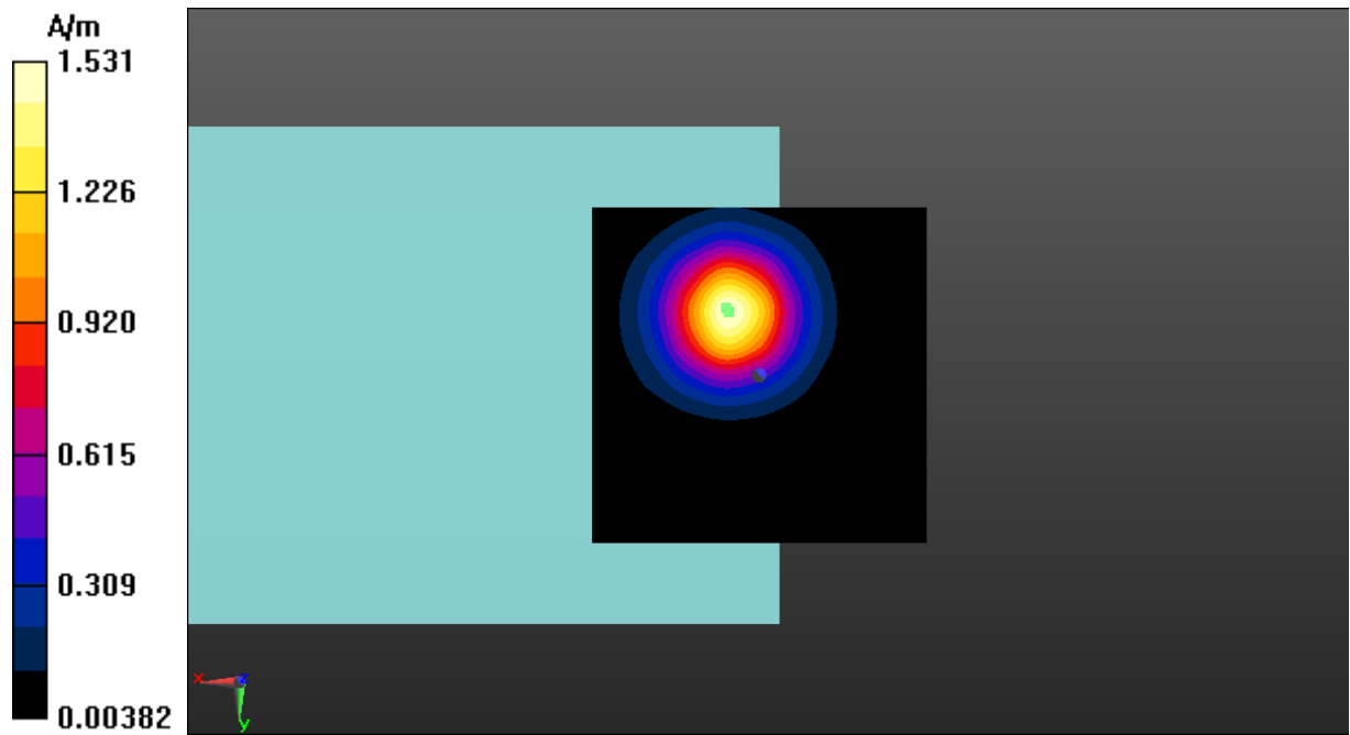
Fig A.24 T-Coil WLAN 2.4GHz-Z
