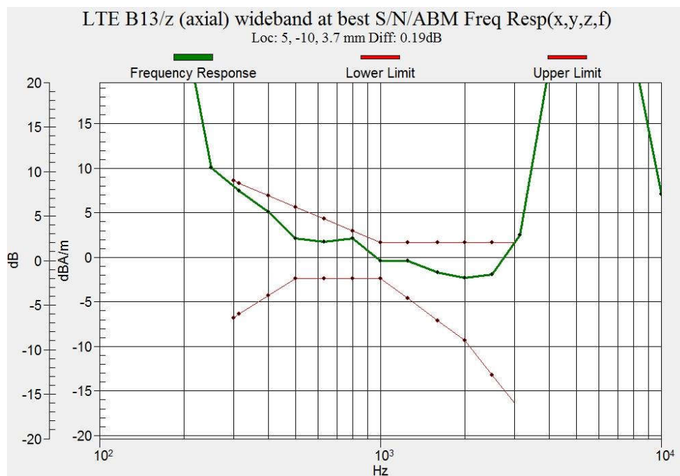
Figure B.25 Frequency Response of LTE Band 13 (Google Duo)
