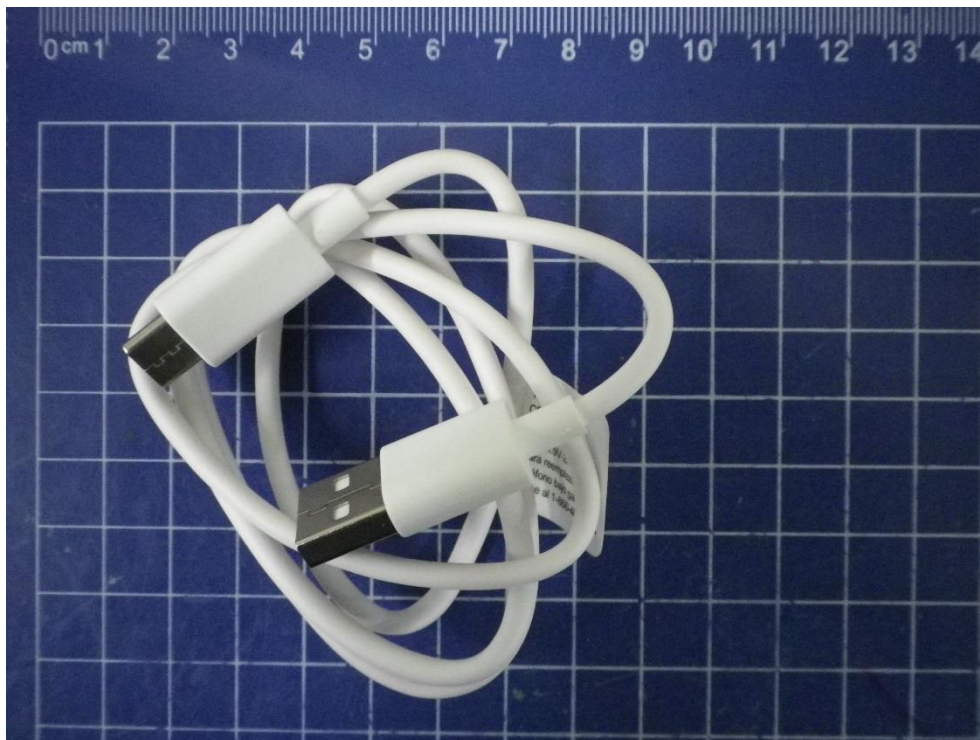
CDA0000202C1 Type C Data Cable, USB A to Type C,0.8 m,JUWEI
