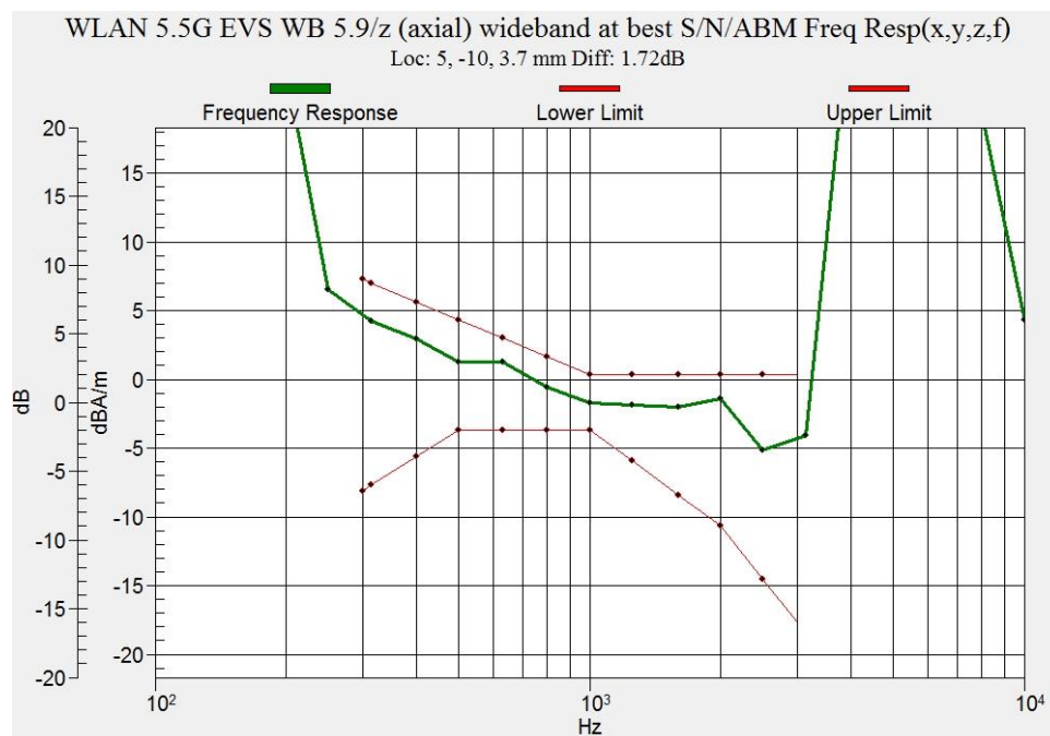
Figure B.16 Frequency Response of WLAN 5.5GHz
