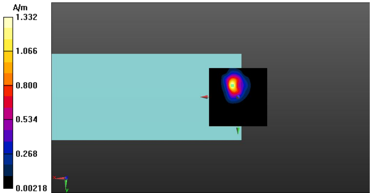
Fig A.15 T-Coil WLAN 5.3GHz-Z
