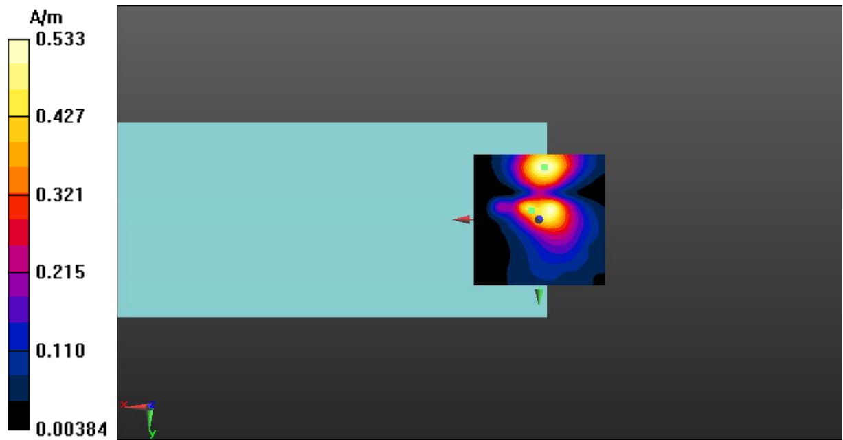
Fig A.16 T-Coil WLAN 5.5GHz-Y
