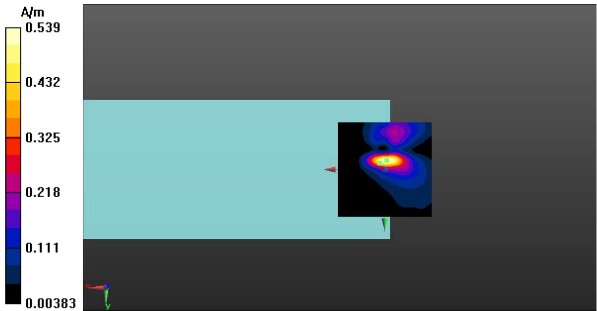
Fig A.13 T-Coil WLAN 2.4GHz-Y
