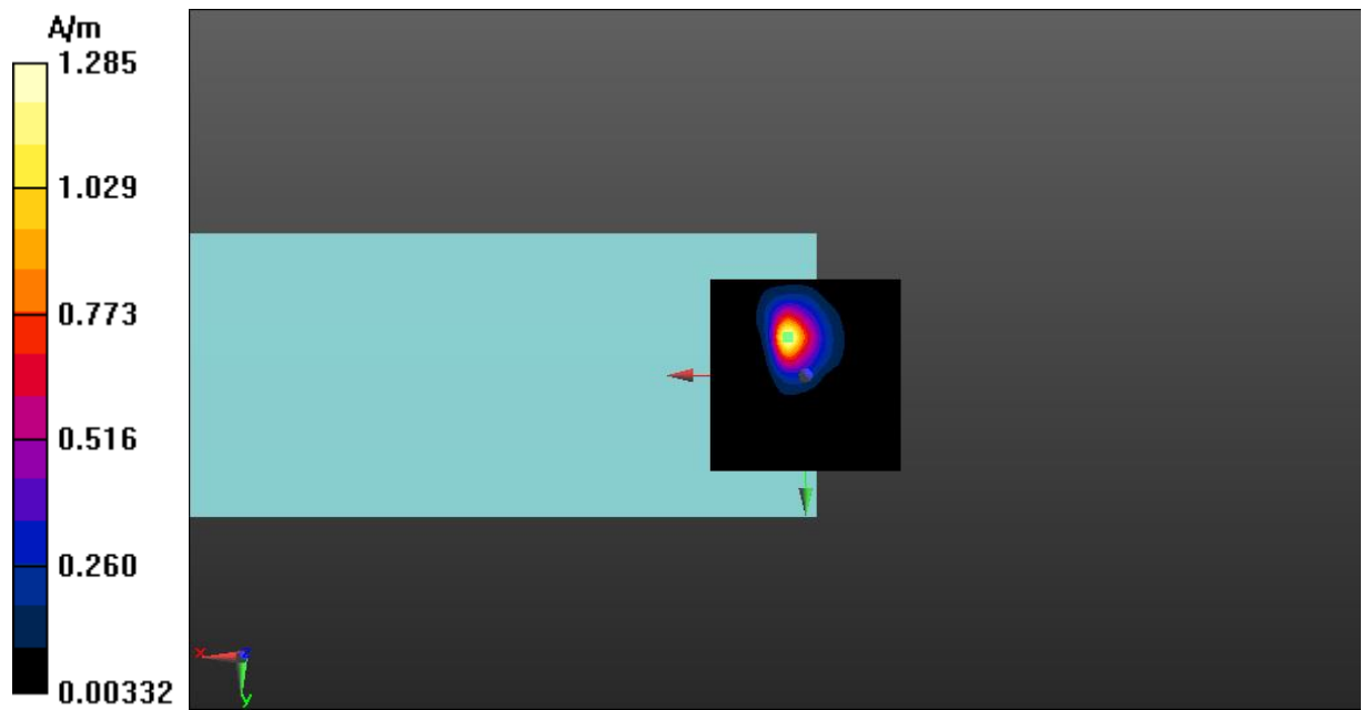
Fig A.13 T-Coil WLAN 2.4GHz-Z
