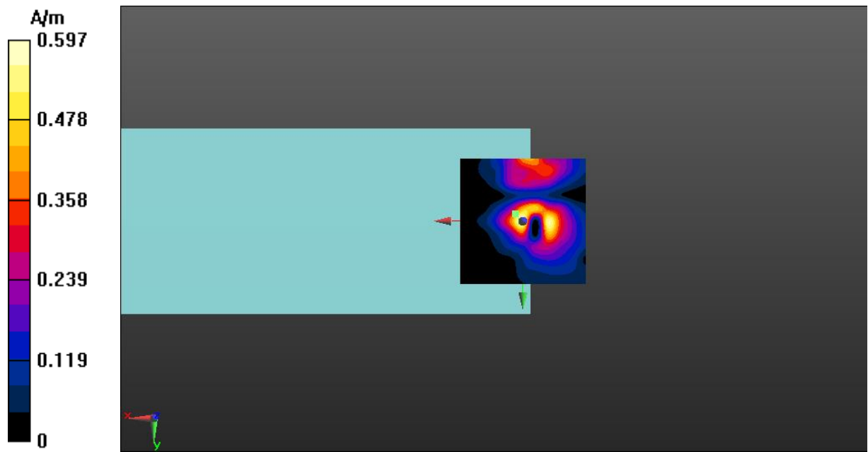
Fig A.19 T-Coil LTE-Band 13-Y
