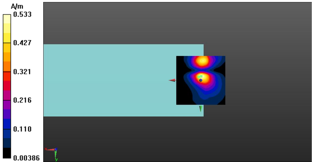
Fig A.17 T-Coil WLAN 5.8GHz-Y
