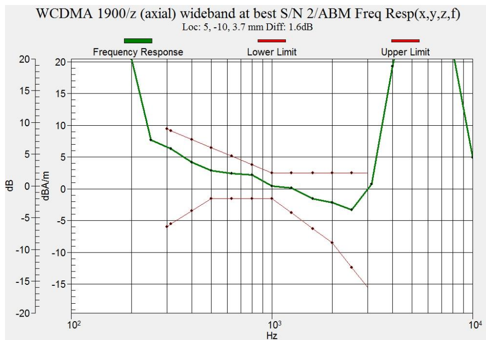
Figure B.18 Frequency Response of WCDMA Band 2 (Google Duo)
