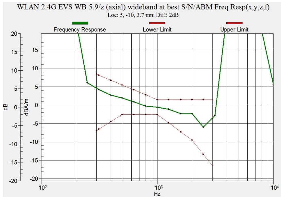
Figure B.13 Frequency Response of WLAN 2.4GHz
