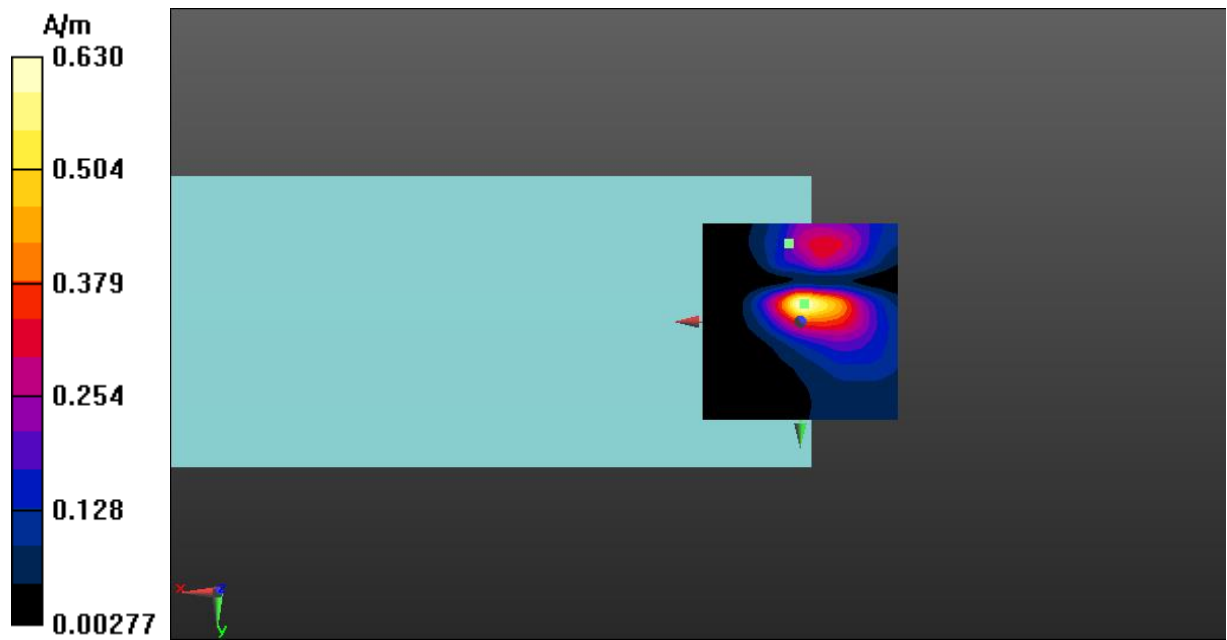
Fig A.20 T-Coil WLAN 2.4GHz-Y
