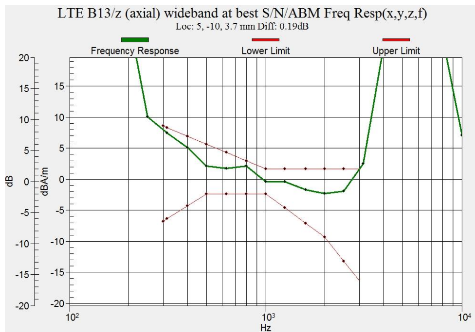
Figure B.19 Frequency Response of LTE Band 13 (Google Duo)
