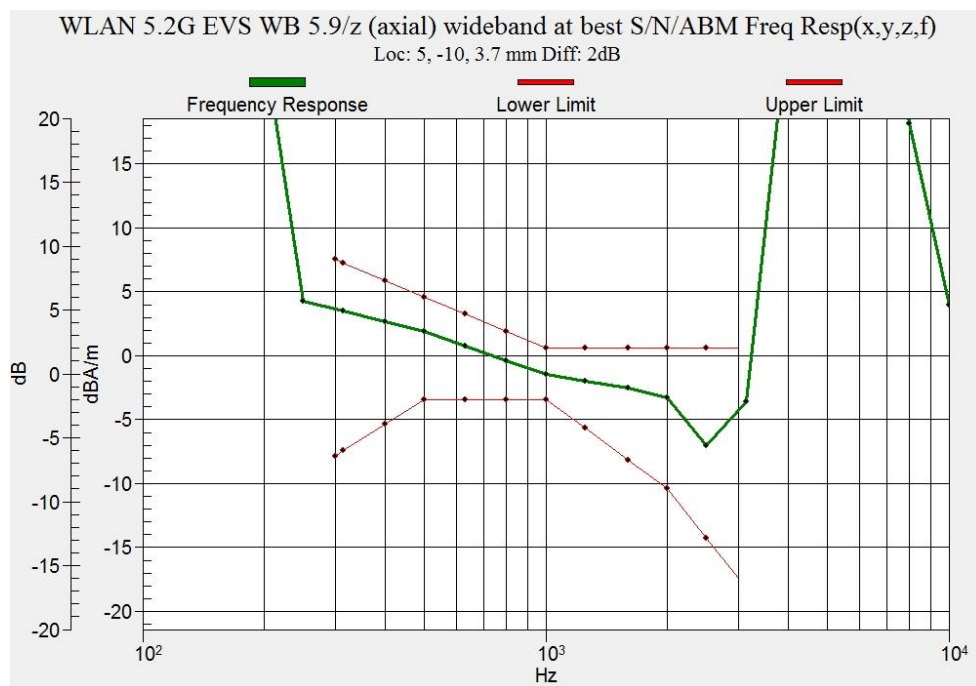
Figure B.14 Frequency Response of WLAN 5.2GHz
