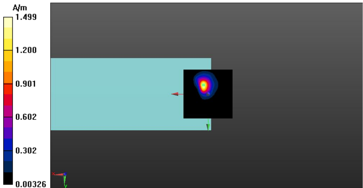
Fig A.21 T-Coil WLAN 5.5GHz-Z
