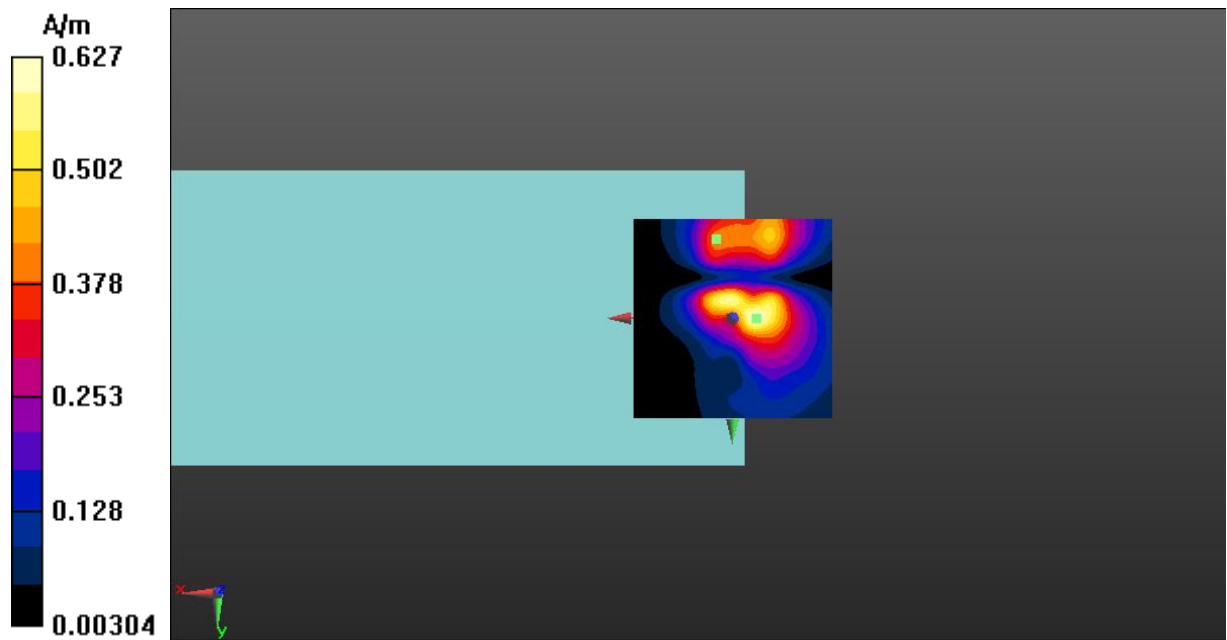
Fig A.21 T-Coil WLAN 5.5GHz-Y
