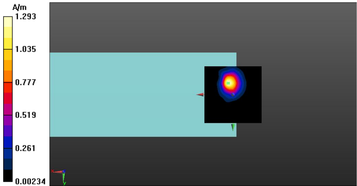
Fig A.16 T-Coil WLAN 5.5GHz-Z
