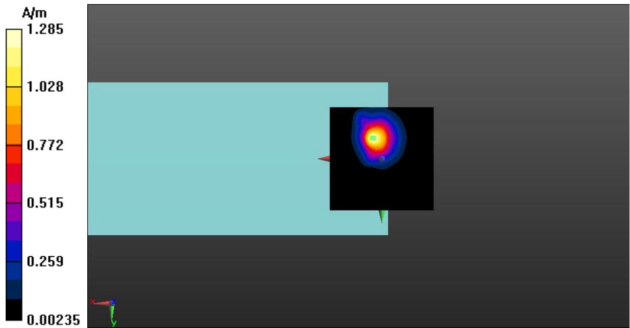
Fig A.14 T-Coil WLAN 5.2GHz-Z
