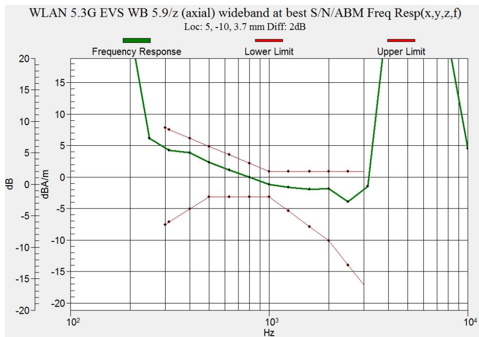
Figure B.15 Frequency Response of WLAN 5.3GHz
