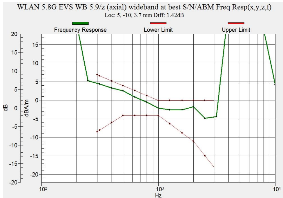
Figure B.17 Frequency Response of WLAN 5.8GHz
