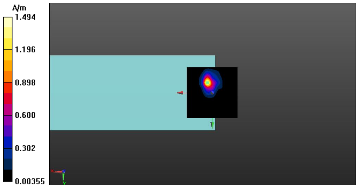
Fig A.19 T-Coil LTE-Band 13-Z
