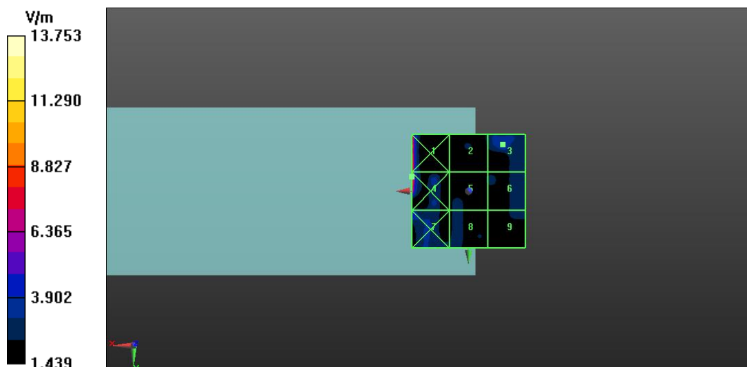
Fig A.9 HAC RF E-Field WLAN 2.4GHz
