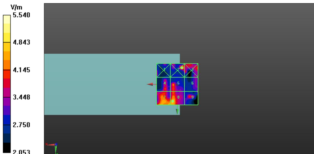
Fig A.7 HAC RF E-Field WLAN 2.4GHz
