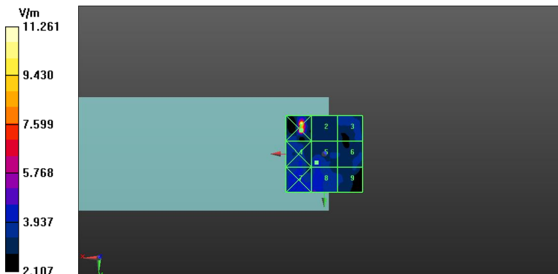
Fig A.8 HAC RF E-Field WLAN 2.4GHz
