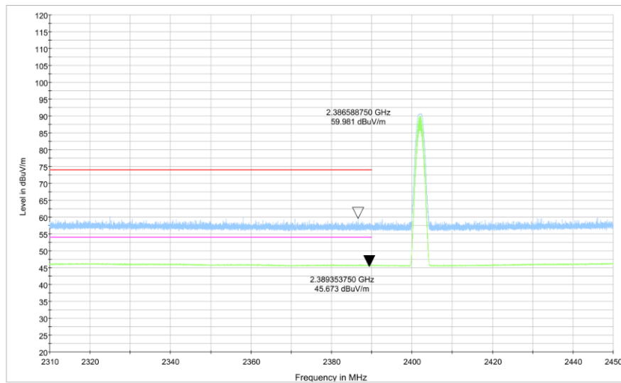
Fig.3. Frequency Band Edges: GFSK, 2402 MHz, Hopping Off, 2.31 GHz – 2.45GHz
