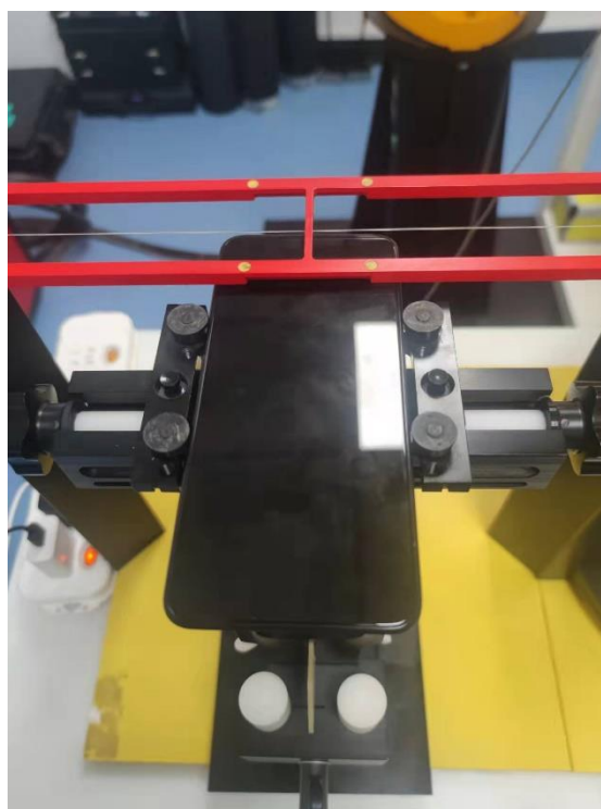
Picture 2: EUT Positioning for RF/T-coil
