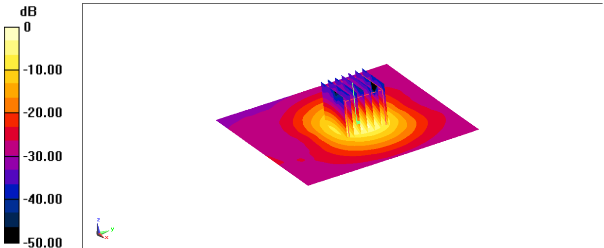
Fig.B.16 validation 5600 MHz 100mW
