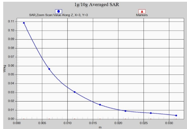
Fig. 1-26 Z-Scan at power reference point (LTE Band41PC2)
