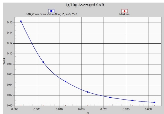
Fig. 1-27 Z-Scan at power reference point (LTE Band41PC2)
