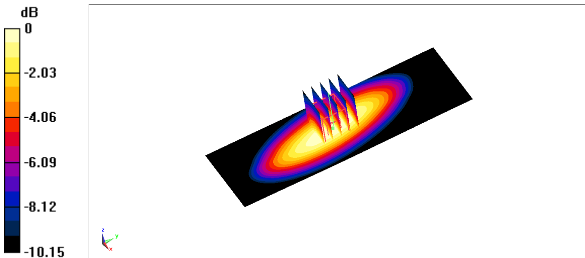
Fig.B.1 validation 750 MHz 250mW
