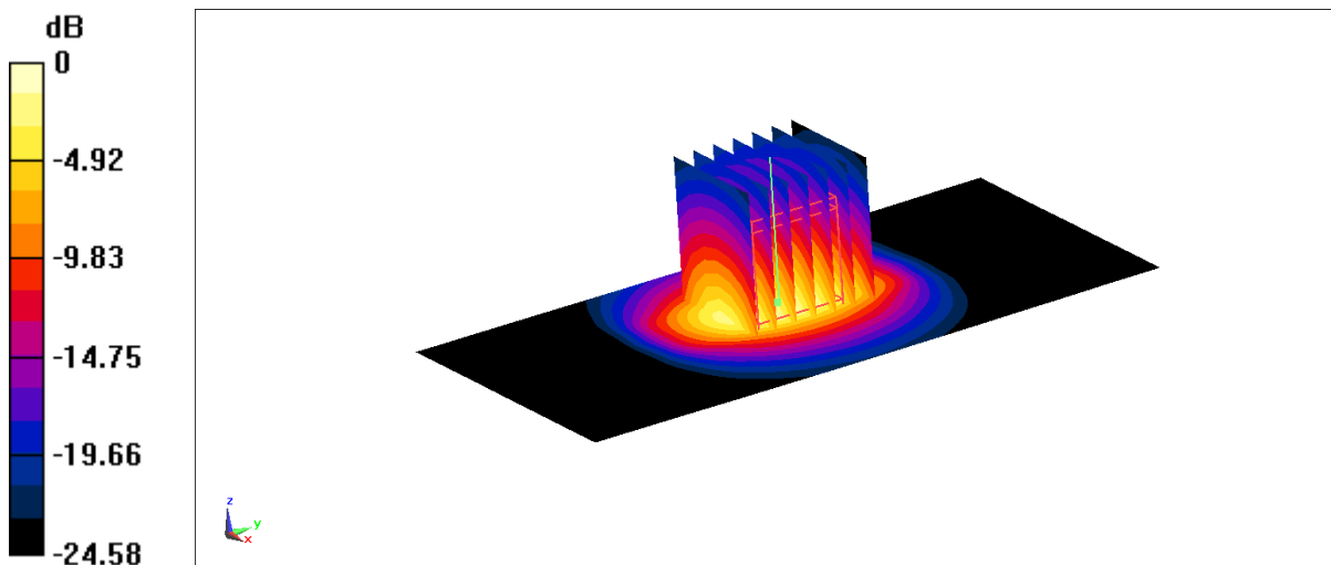
Fig.B.13 validation 2600 MHz 250mW
