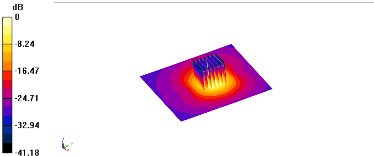
Fig.B.15 validation 5250 MHz 100mW
