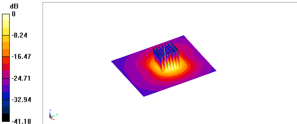
Fig.B.14 validation 5250 MHz 100mW
