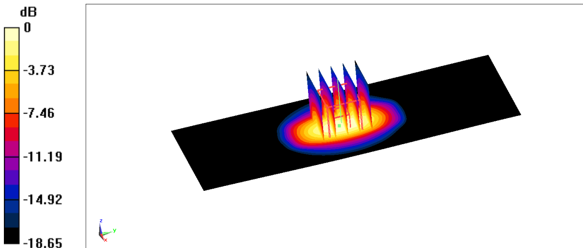
Fig.B.9 validation 1900 MHz 250mW
