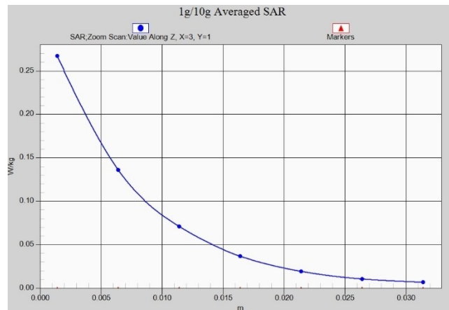
Fig. 1-28 Z-Scan at power reference point (LTE Band41PC2)
