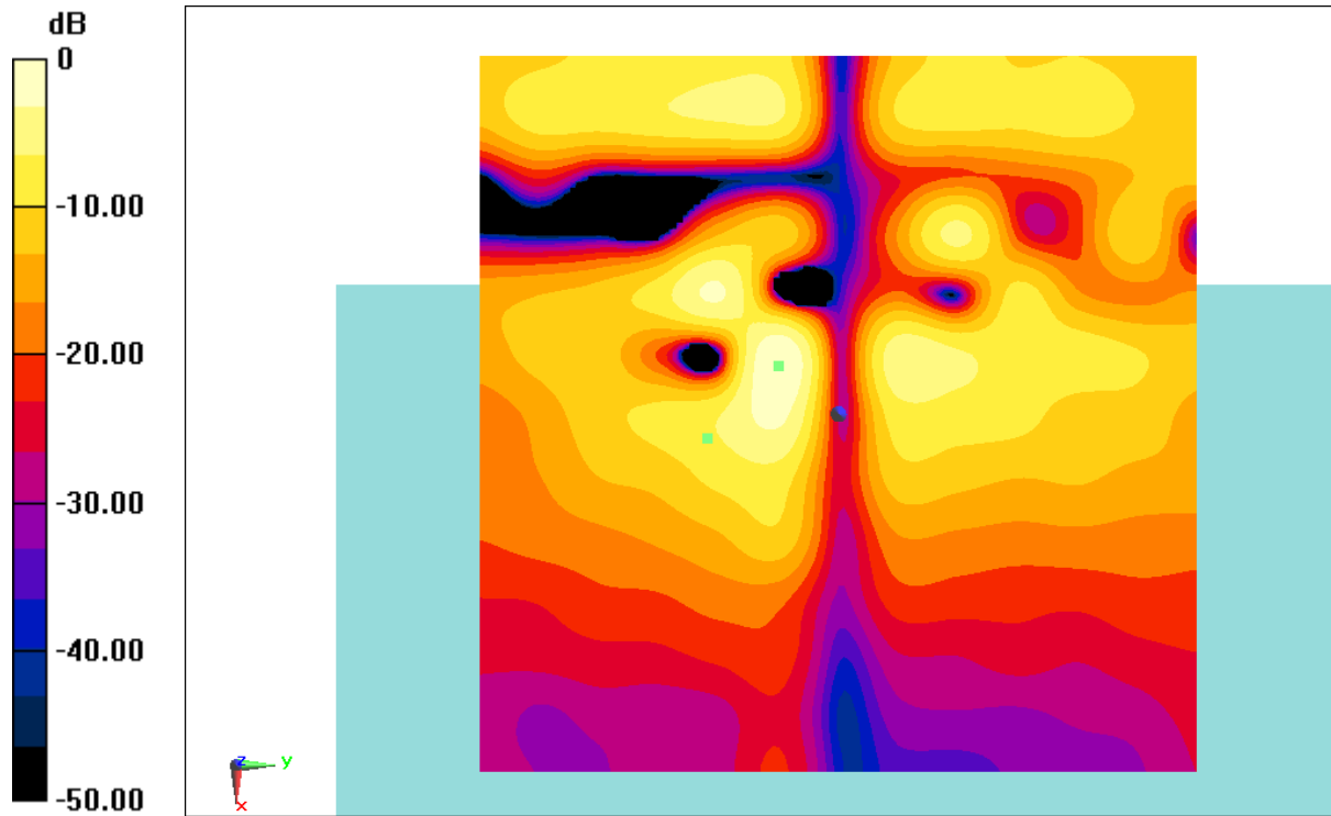
Fig B.17 T-Coil WiFi-2.4G
