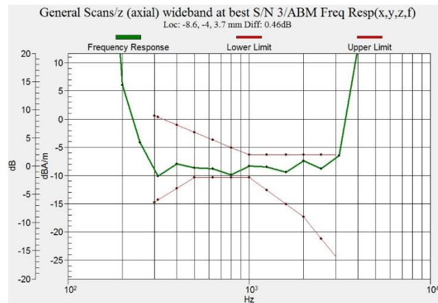
Figure C.7 Frequency Response of LTE B66 - OTT VoIP
