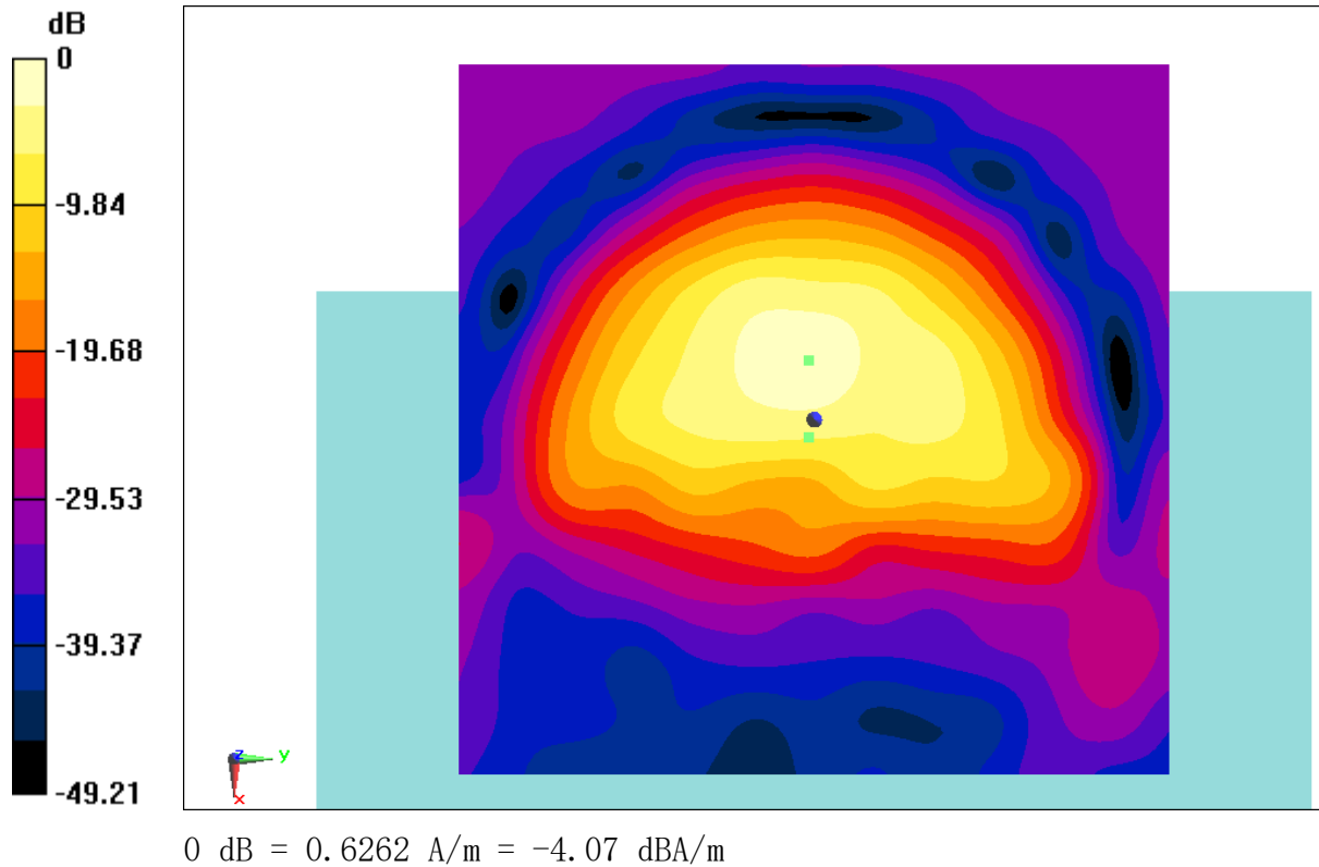
Fig B.10 T-Coil WiFi-2.4G
