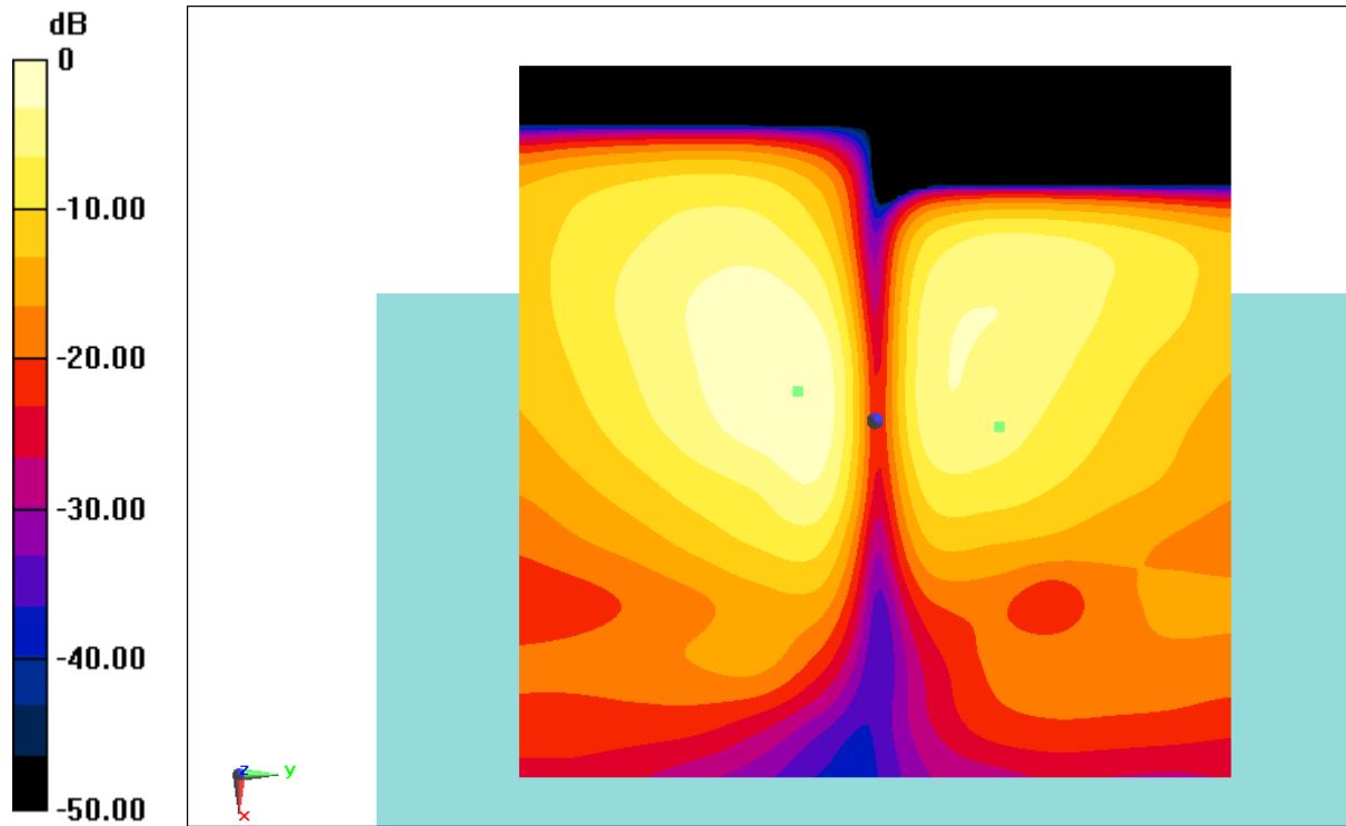
Fig B.5 T-Coil LTE B13
