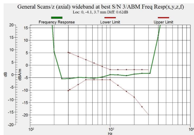
Figure C.6 Frequency Response of WCDMA1900 - OTT VoIP
