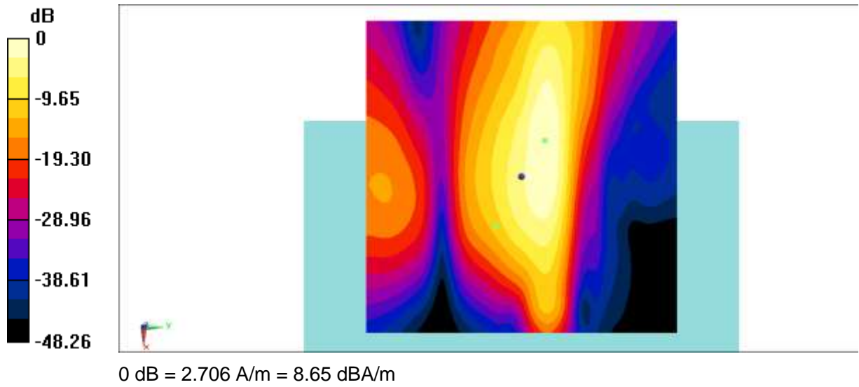
Fig B.1 T-Coil GSM 850
