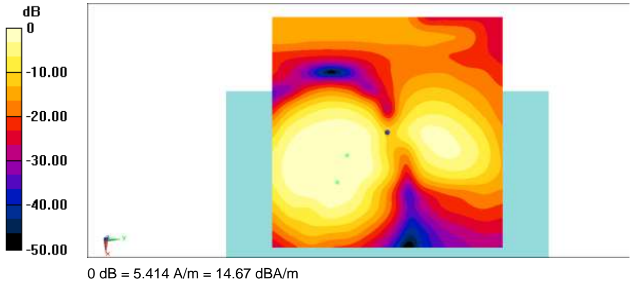
Fig B.4 T-Coil LTE B2
