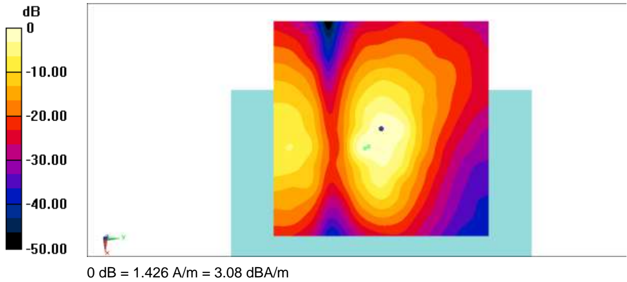
Fig B.7 T-Coil LTE B66
