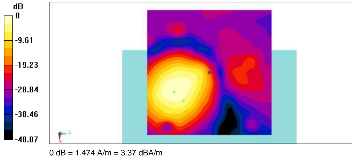
Fig B.8 T-Coil LTE B66
