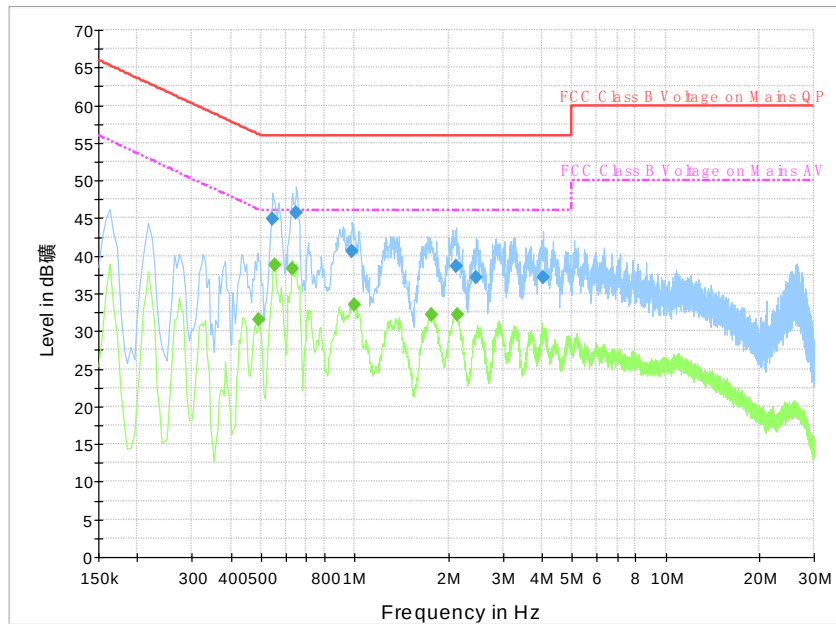
Fig.101. AC Powerline Conducted Emission-Iidle
