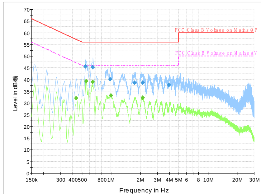
Fig.100. AC Powerline Conducted Emission- bluetooth
