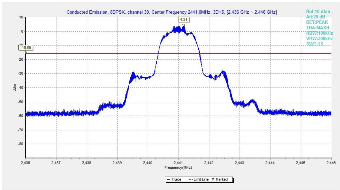
Fig.54. Conducted spurious emission: 8DPSK, Channel 39, 2441MHz
