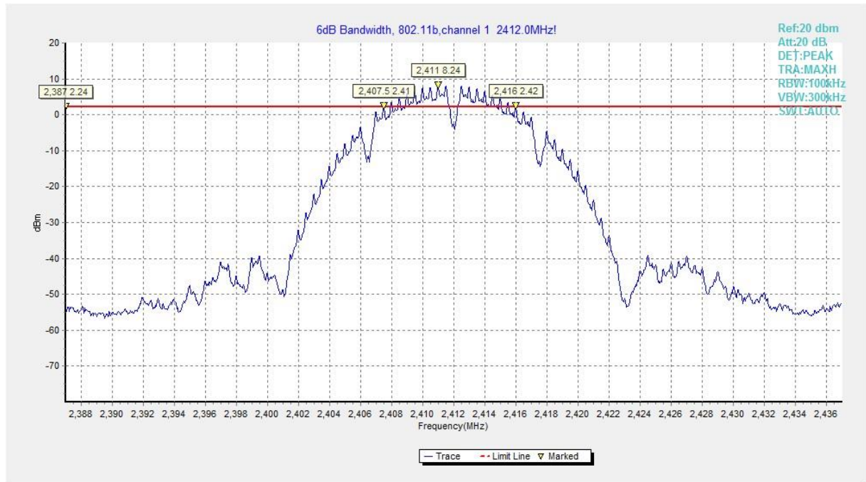
Fig.13. Occupied 6dB Bandwidth(802.11b,Ch 1)
