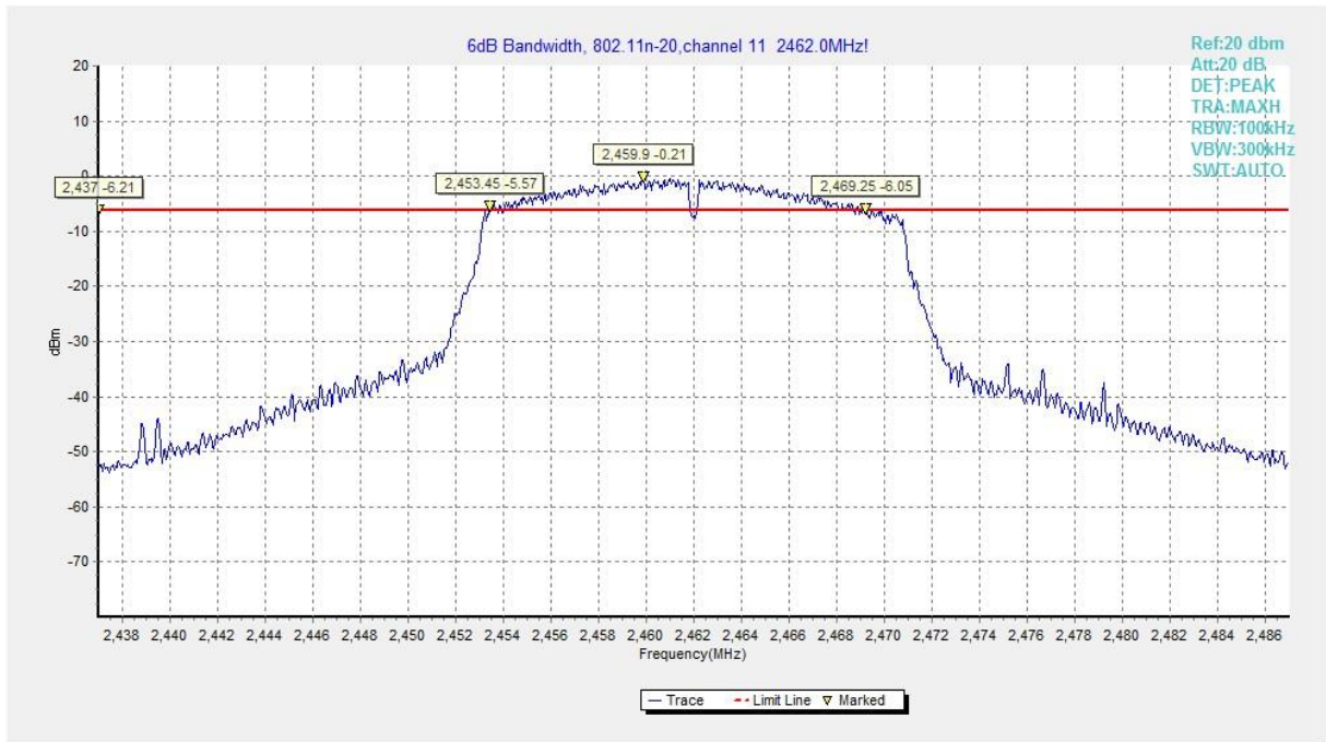
Fig.21. Occupied 6dB Bandwidth (802.11n-HT20, Ch 11)
