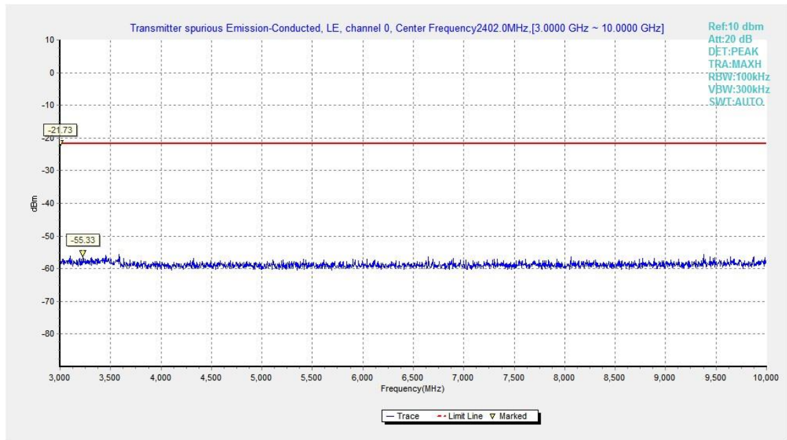
Fig.8. Transmitter Spurious Emission - Conducted: GFSK, 2402 MHz,3GHz - 10GHz
