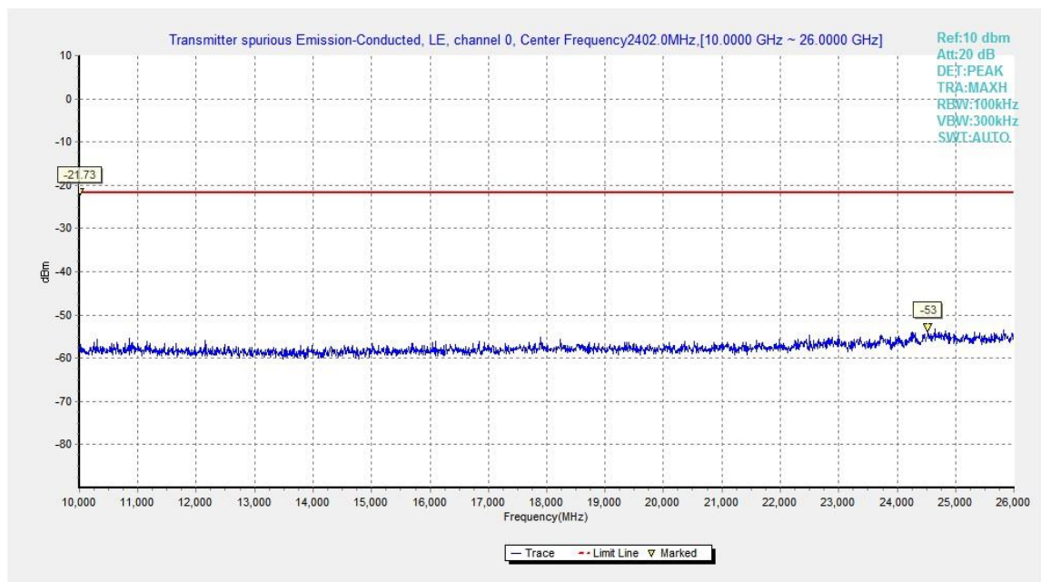
Fig.9. Transmitter Spurious Emission - Conducted: GFSK, 2402 MHz,10GHz - 26GHz
