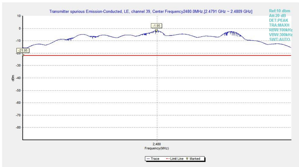
Fig.15. Transmitter Spurious Emission - Conducted: GFSK, 2480 MHz
