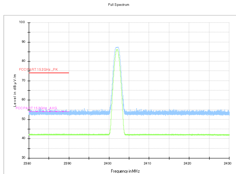
Fig.3. Frequency Band Edges: GFSK, GFSK, Channel 0, 2.38GHz – 2.43GHz
