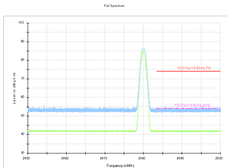
Fig.4. Frequency Band Edges: GFSK, Channel 39, 2.45 GHz - 2.50GHz
