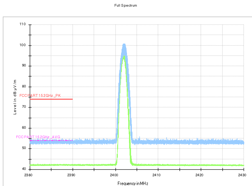
Fig.15. Frequency Band Edges: \pi/4 DQPSK, Channel 0, 2.38GHz – 2.43GHz
