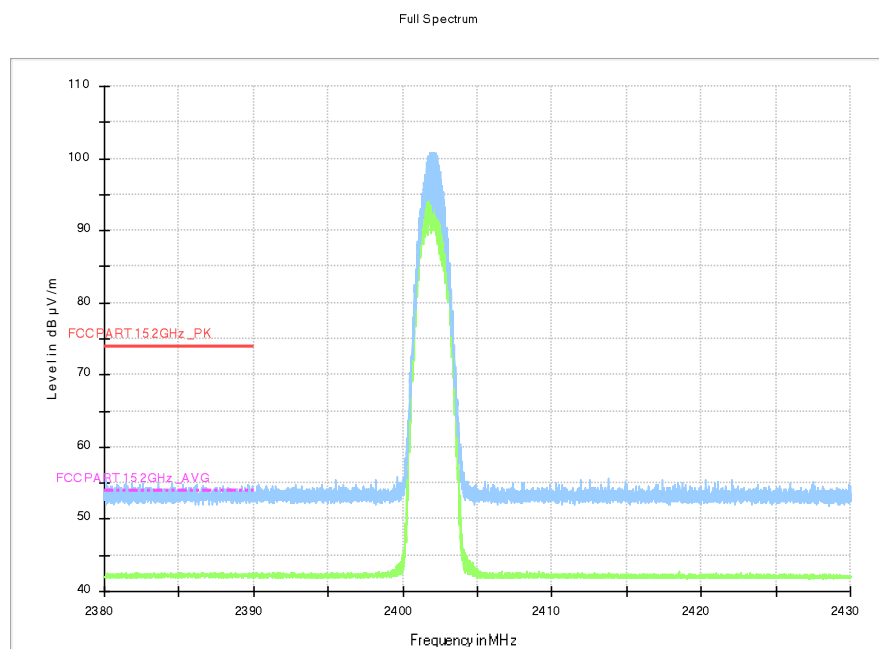
Fig.17. Frequency Band Edges: 8DPSK, Channel 0, 2.38GHz – 2.43GHz
