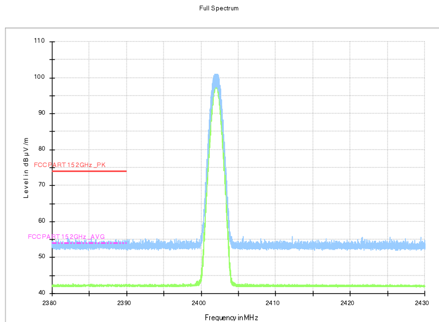
Fig.13. Frequency Band Edges: GFSK, Channel 0, 2.38GHz – 2.43GHz
