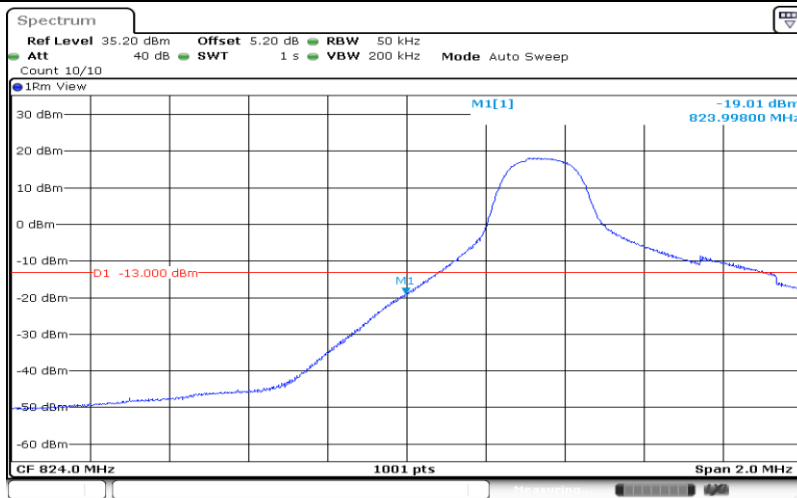
Band5-5MHz-QPSK-20425-25RB#0
