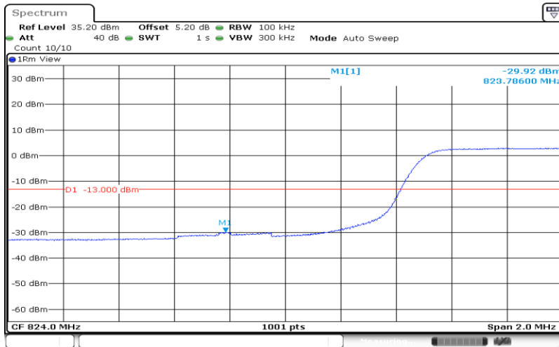
Band5-10MHz-16QAM-20450-50RB#0
