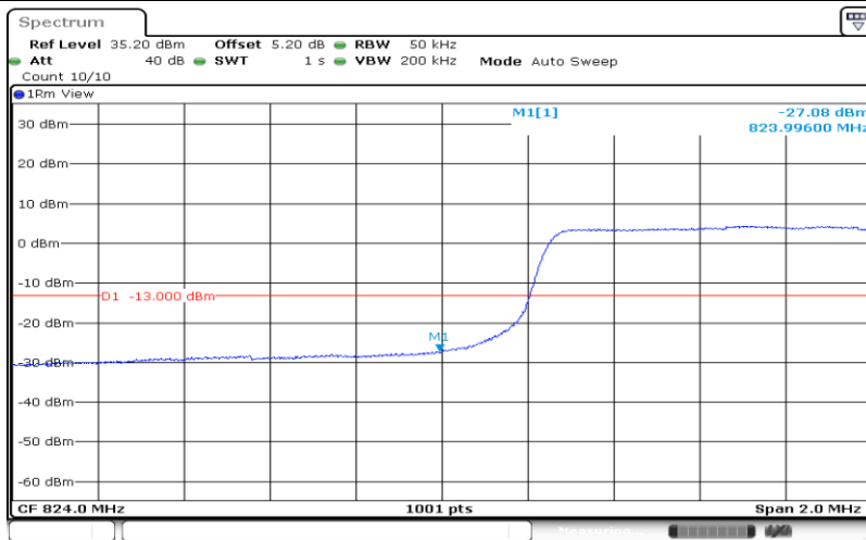
Band5-5MHz-QPSK-20425-25RB#0
