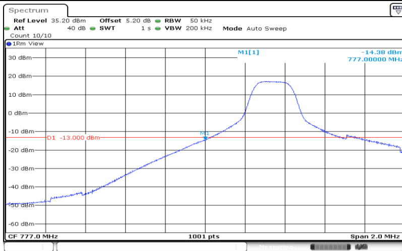
Band13-5MHz-16QAM-23205-25RB#0
