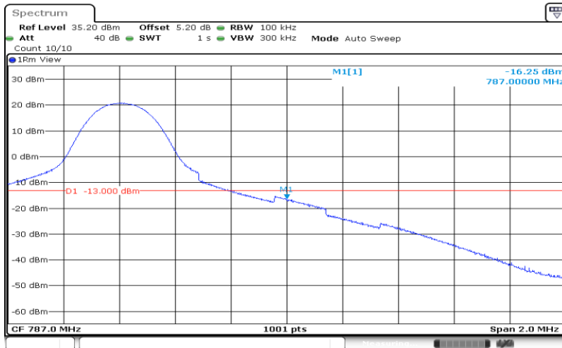
Band13-10MHz-QPSK-23230_Right-1RB#49
