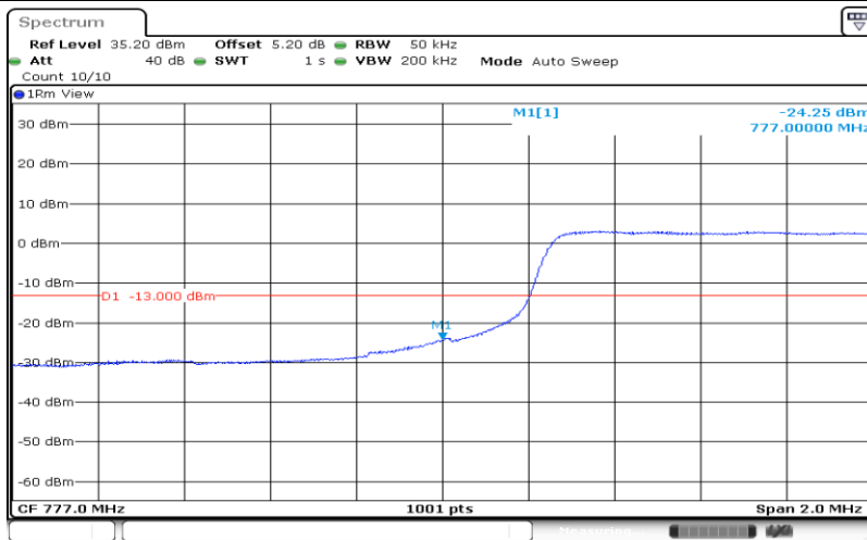
Band13-5MHz-16QAM-23205-25RB#0
