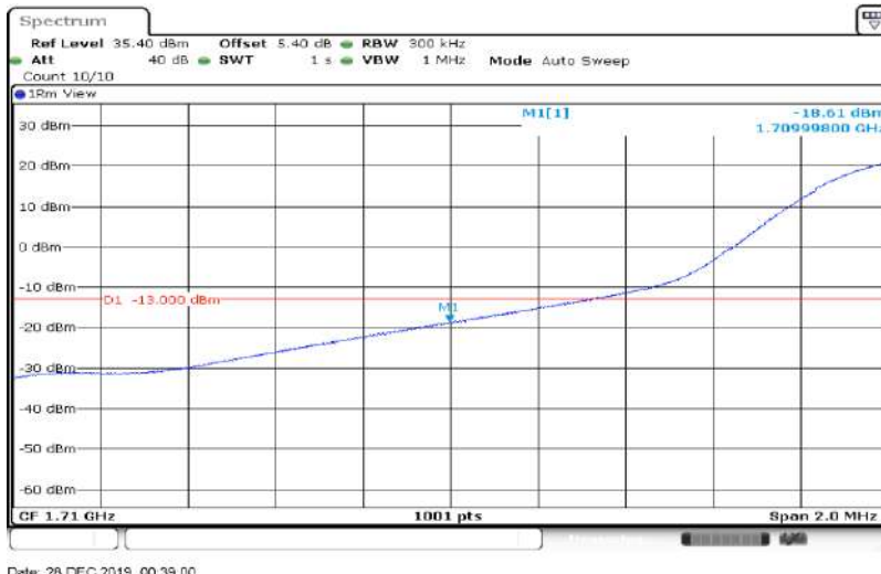
Band66-20MHz-16QAM-132072-100RB#0
