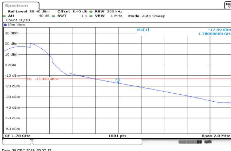
Band66-15MHz-QPSK-132597-75RB#0
