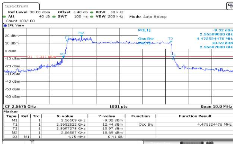
Band7-5MHz-16QAM-20775-25RB#0-4.476
