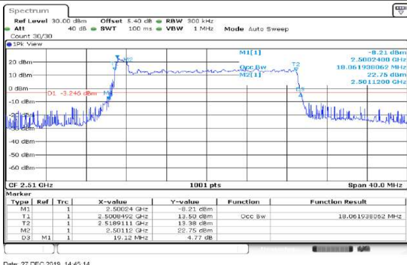
Band7-20MHz-QPSK-21100-100RB#0-18.062
