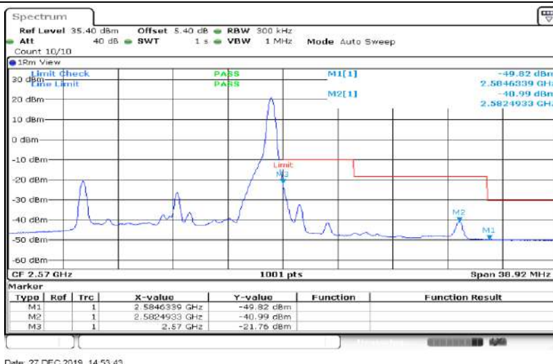
Band7-15MHz-16QAM-21375-75RB#0
