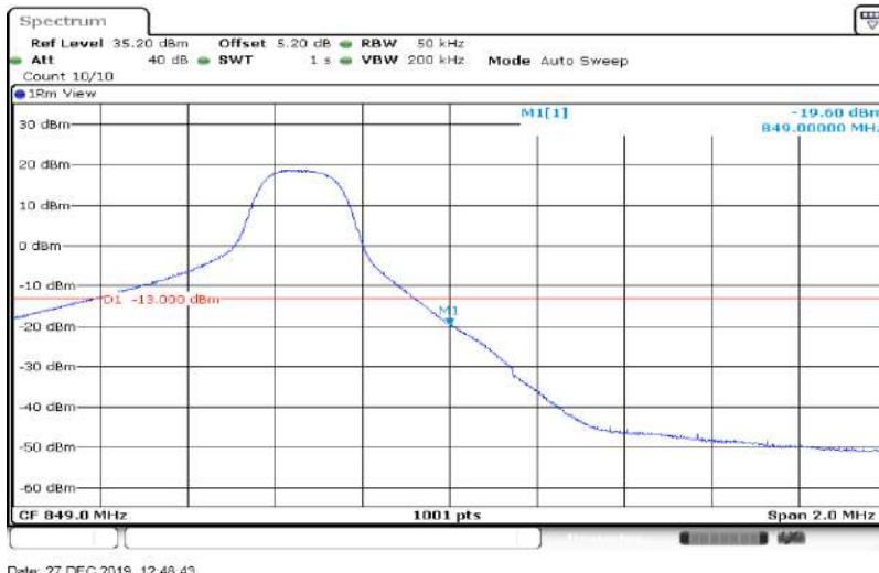
Band5-5MHz-QPSK-20625-25RB#0
