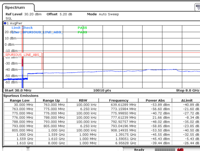
Band13-10MHz-QPSK-23230-1RB#0-Range1
