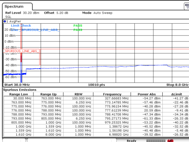
Band13-10MHz-16QAM-23230-1RB#0-Range1
