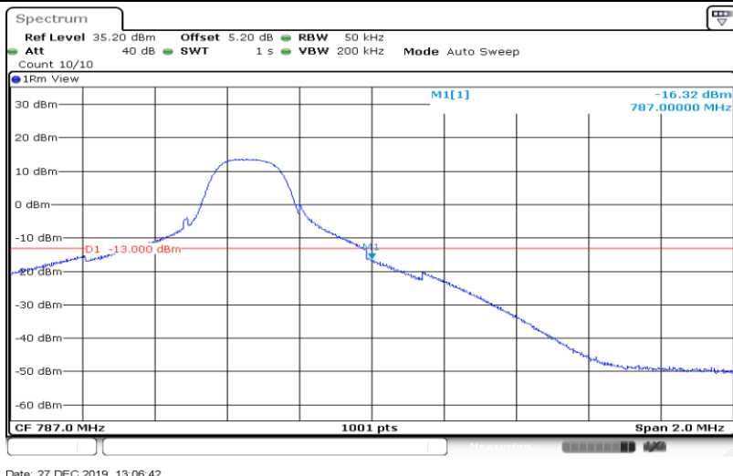
Band13-5MHz-QPSK-23255-25RB#0
