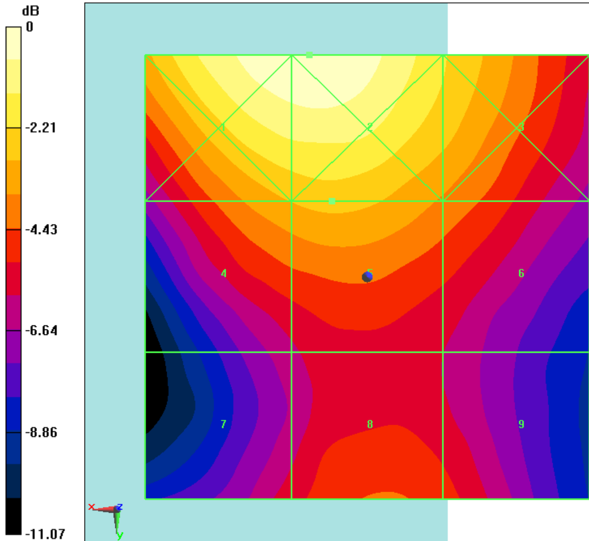
Fig B.6 HAC RF E-Field GSM 1900 Low
