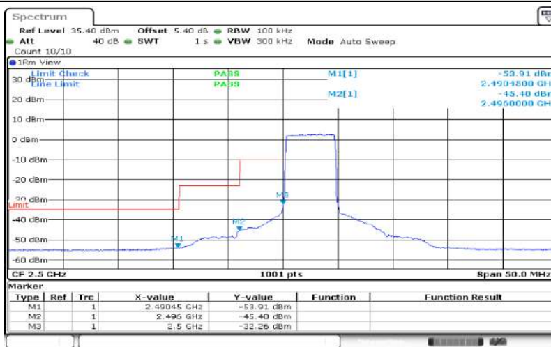
Band7-5MHz-QPSK-20775-25RB#0
