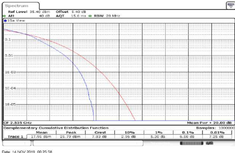
Band7-20MHz-16QAM-21350-100RB#0
