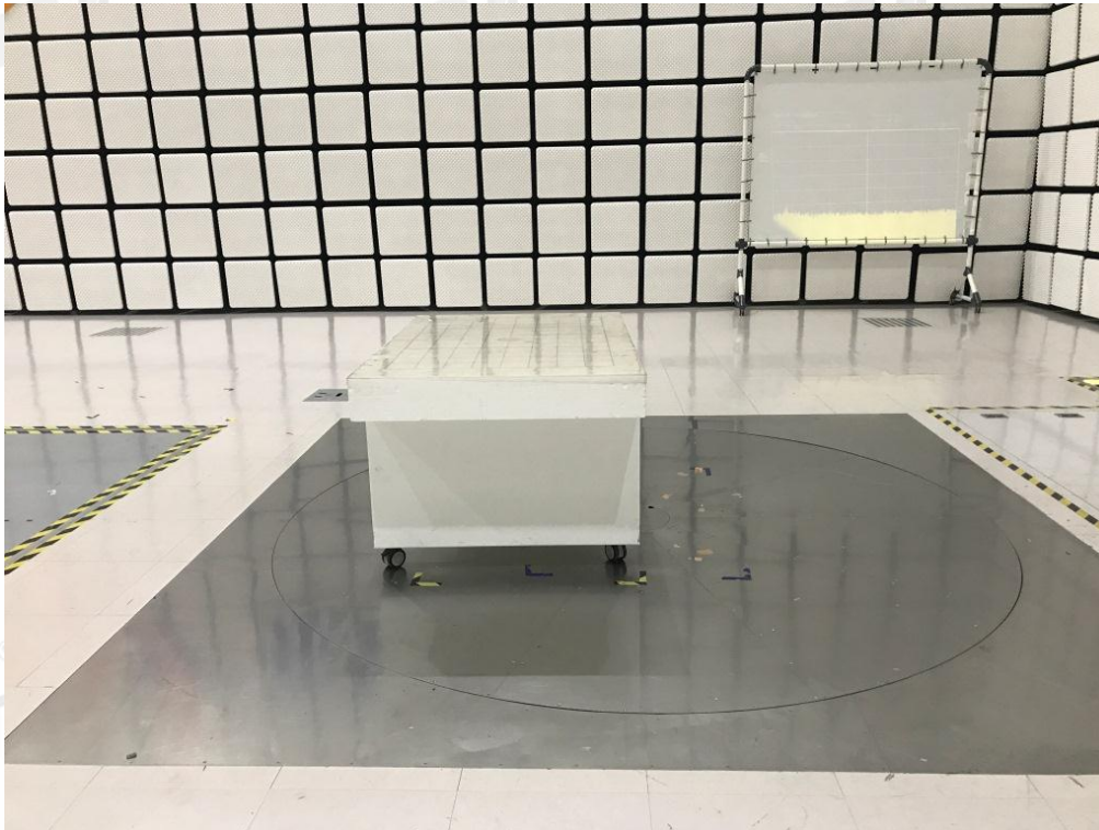
Turn Table Position for below 1GHz
