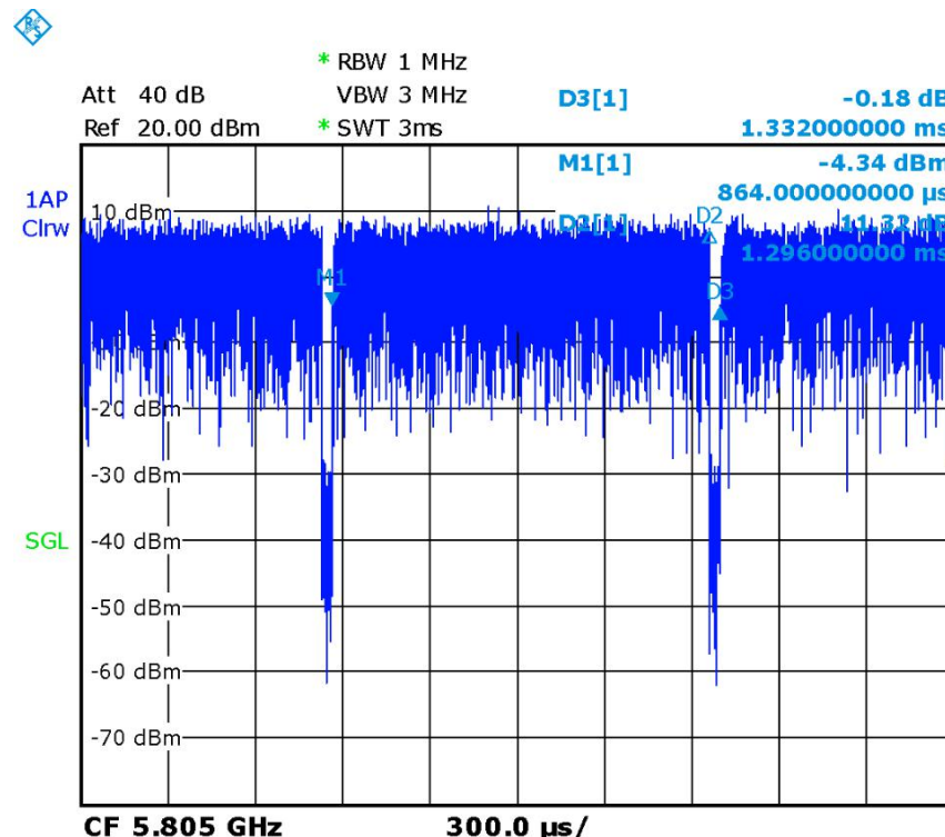
Picture 14.2 The plot of duty factor for UNII-3
