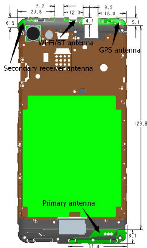
Picture 12.1 Antenna Locations
