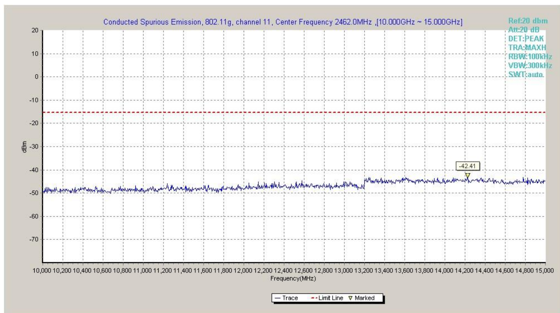
Fig.A.6.1.22 Transmitter Spurious Emission - Conducted (802.11g, Ch11, 10 GHz-15 GHz)
