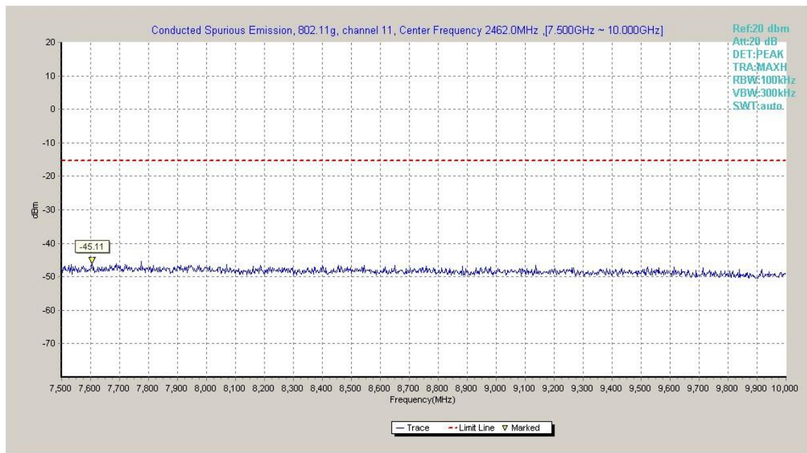
Fig.A.6.1.21 Transmitter Spurious Emission - Conducted (802.11g, Ch11, 7.5 GHz-10 GHz)
