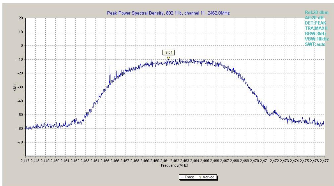
Fig.A.3.3 Power Spectral Density (802.11b, Ch 11)
