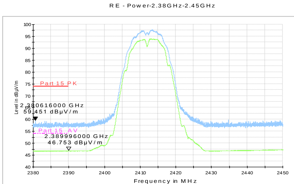
Fig.A.6.2.1 Transmitter Spurious Emission - Radiated (Power): 802.11b, ch1, 2.38 GHz
