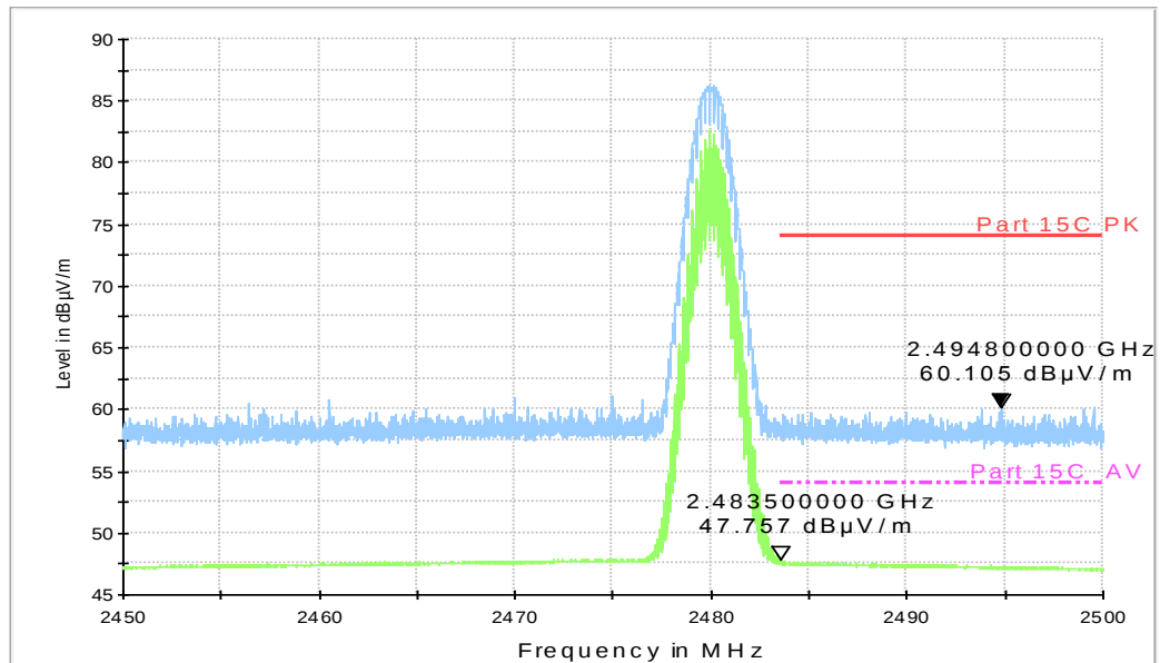
RE - Power-2.45GHz-2.5GHz
