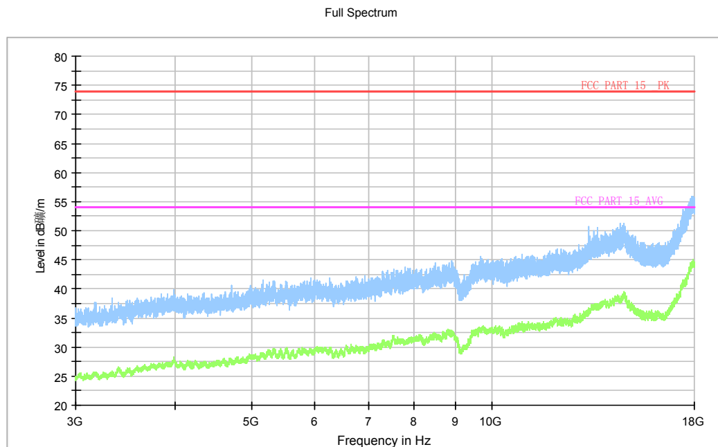
Fig.82. Radiated emission: 8DPSK, Channel 39, 3 GHz - 18 GHz
