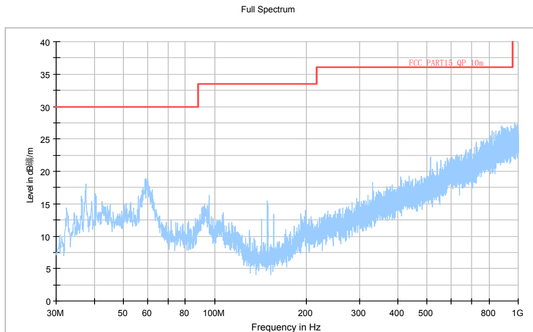
Fig.70. Radiated emission: \pi/4 DQPSK, Channel 39, 30 MHz - 1 GHz
