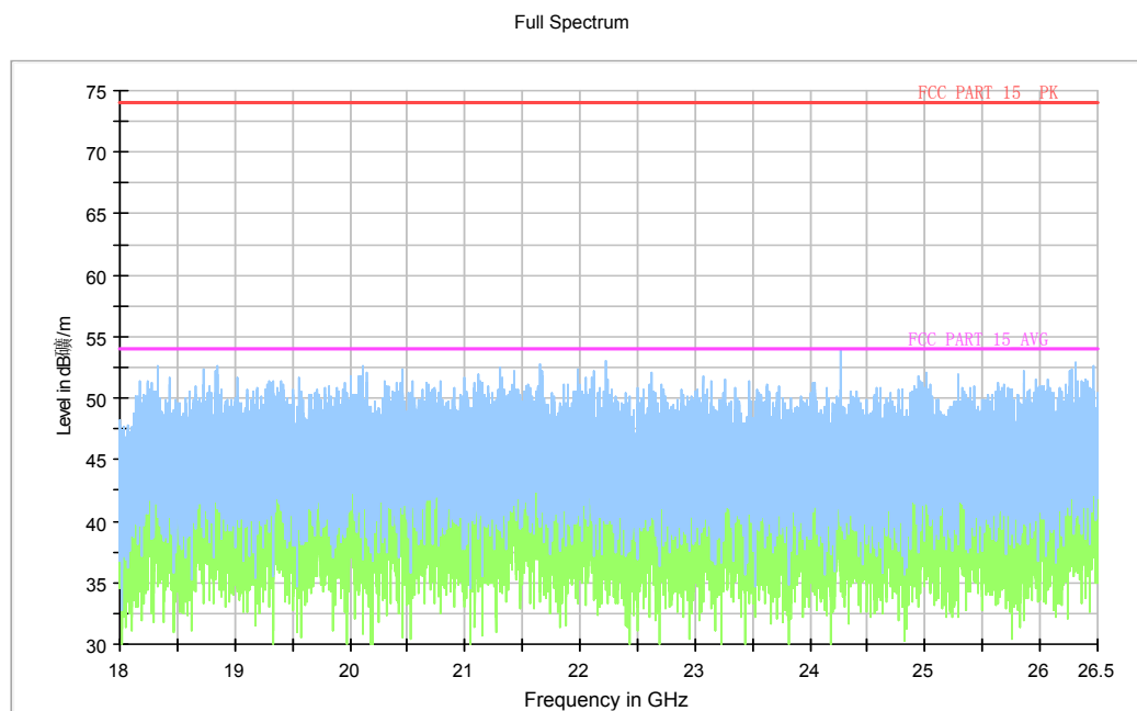
Fig.77. Radiated emission: \pi/4 DQPSK, 18 GHz - 26 GHz
