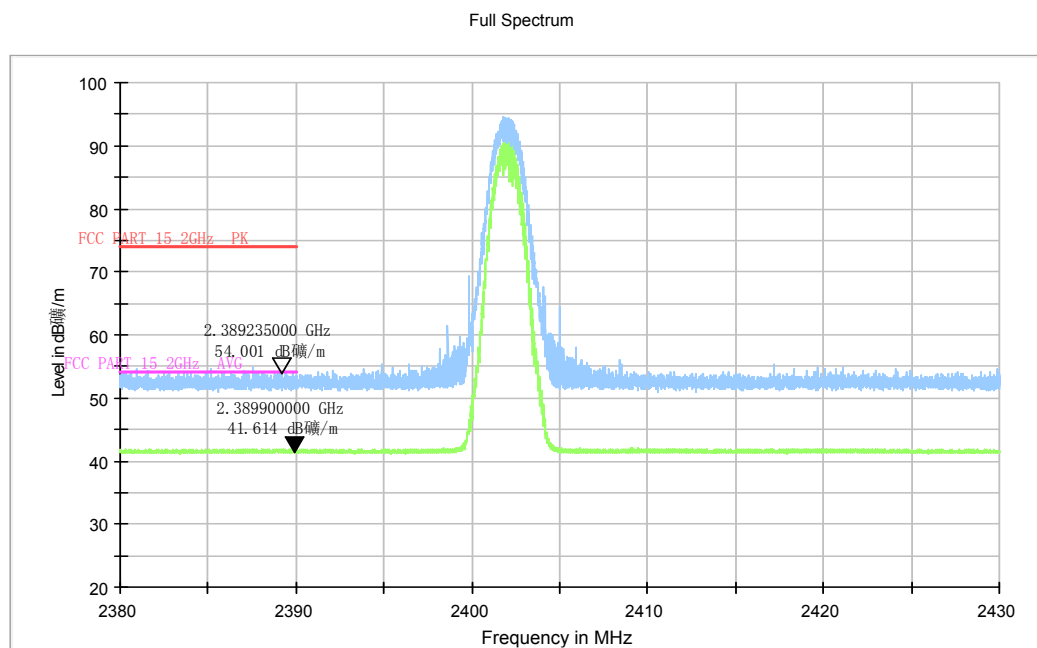
Fig.75. Radiated emission (Power): \pi/4 DQPSK, low channel
