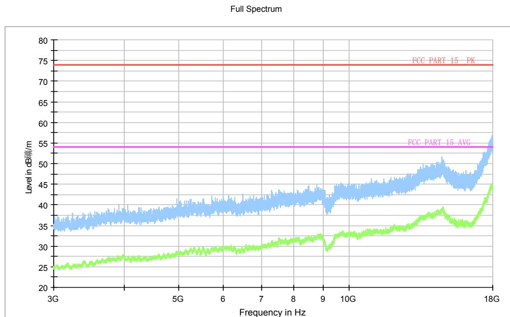
Fig.84. Radiated emission: 8DPSK, Channel 78, 3 GHz - 18 GHz
