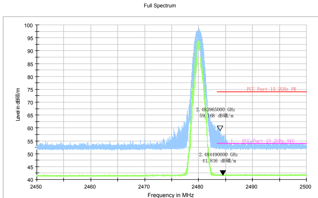
Fig.86. Radiated emission (Power): 8DPSK, high channel
