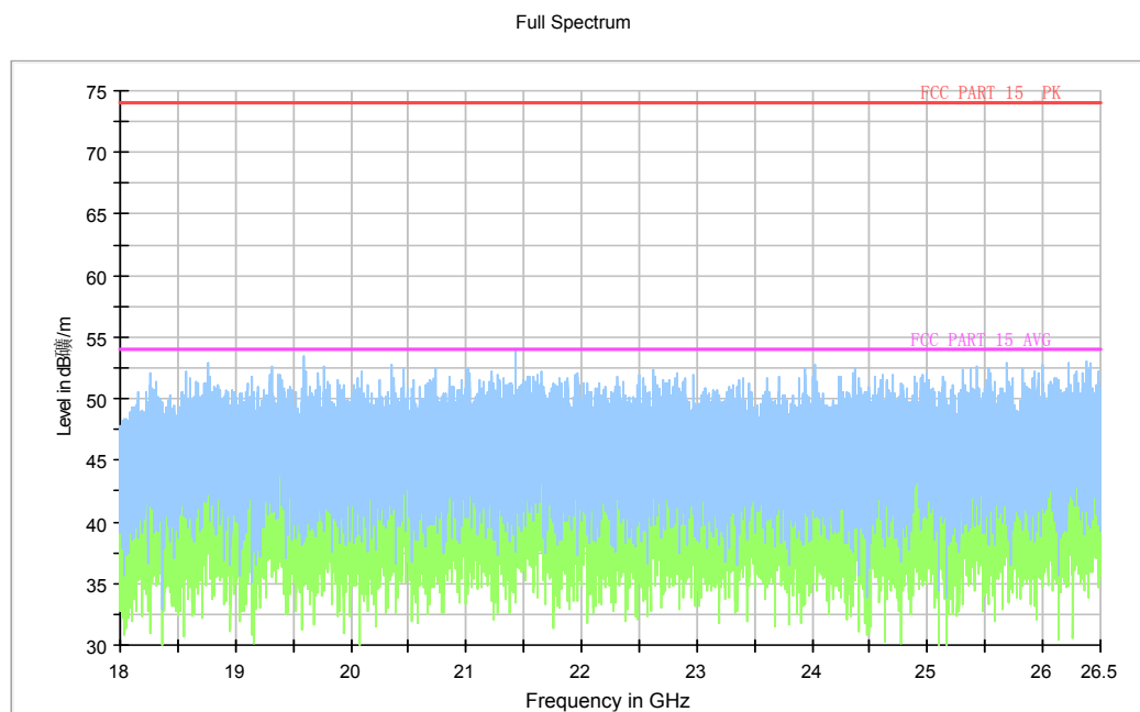
Fig.87. Radiated emission: 8DPSK, 18 GHz - 26 GHz
