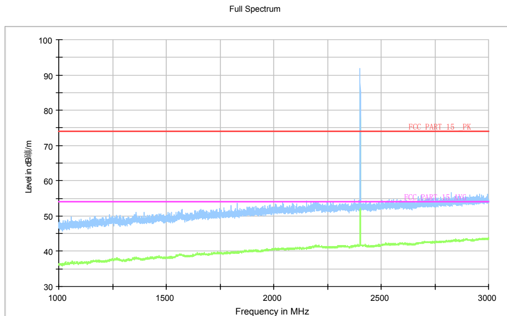
Fig.78. Radiated emission: 8DPSK, Channel 0, 1 GHz - 3 GHz
