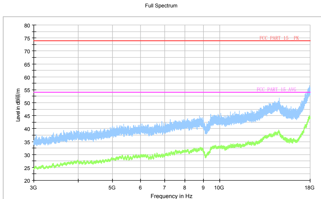
Fig.62. Radiated emission: GFSK, Channel 39, 3 GHz - 18 GHz
