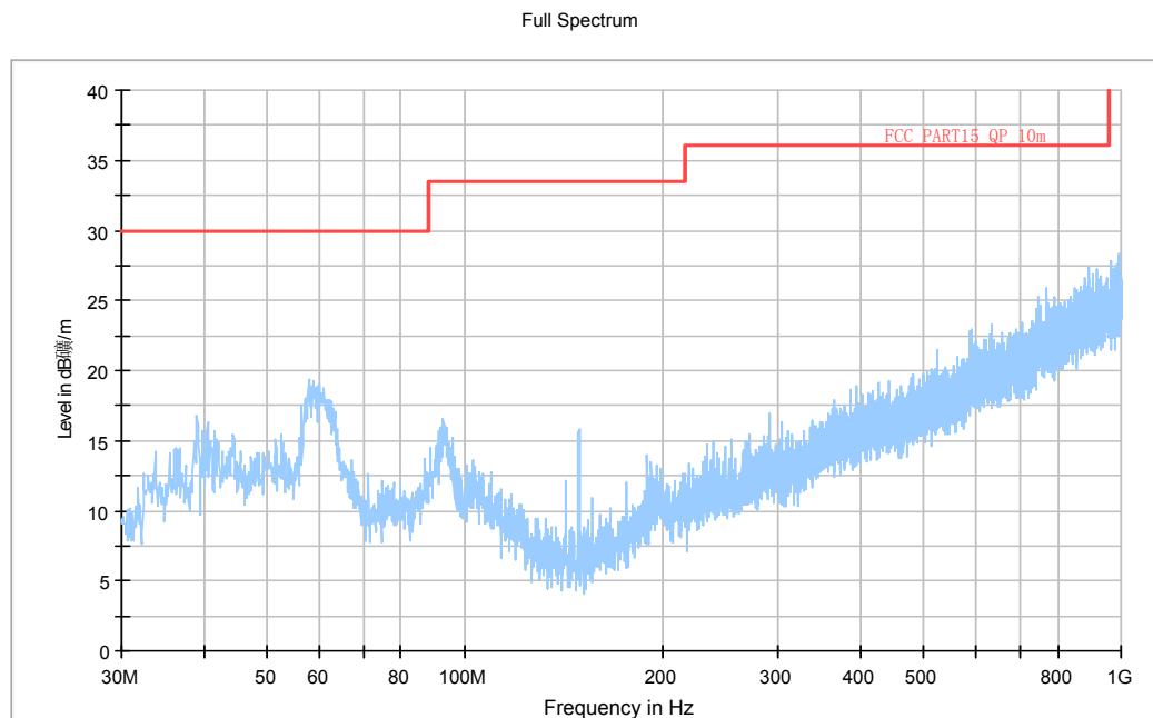
Fig.60. Radiated emission: GFSK, Channel 39, 30 MHz - 1 GHz
