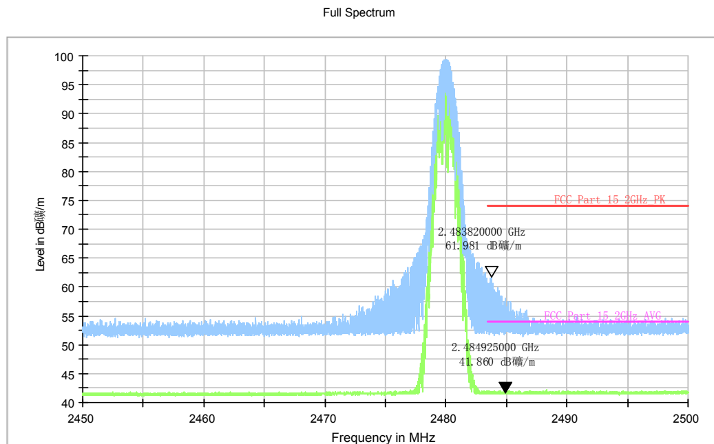
Fig.76. Radiated emission (Power): \pi/4 DQPSK, high channel
