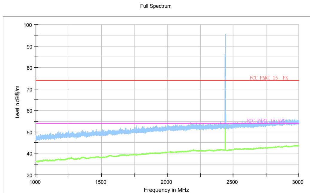
Fig.71. Radiated emission: \pi/4 DQPSK, Channel 39, 1 GHz - 3 GHz
