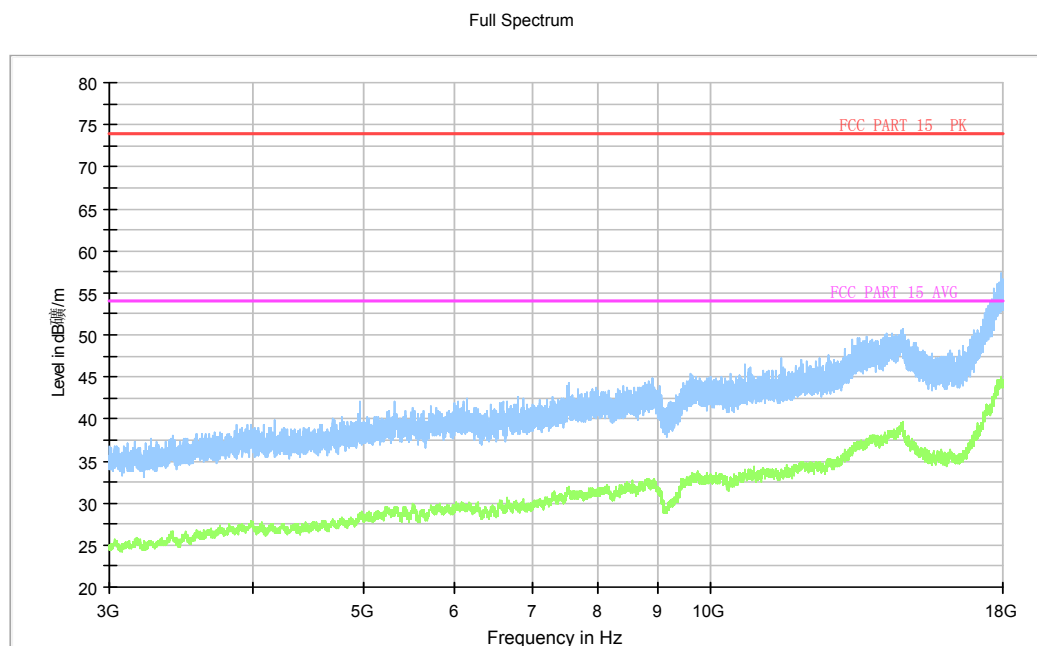
Fig.79. Radiated emission: 8DPSK, Channel 0, 3 GHz - 18 GHz
