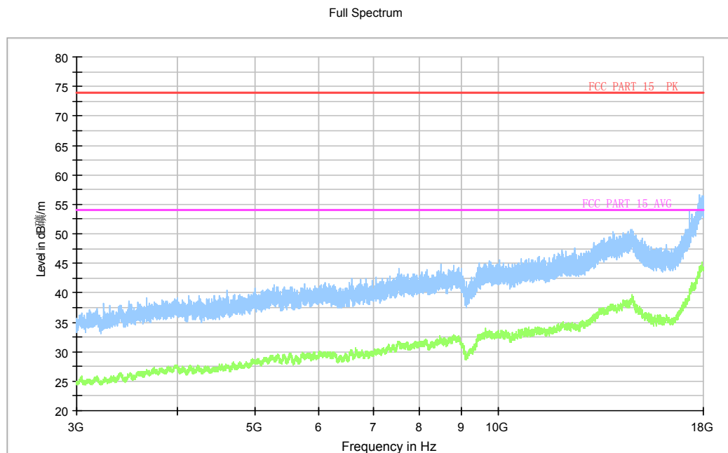
Fig.64. Radiated emission: GFSK, Channel 78, 3 GHz - 18 GHz
