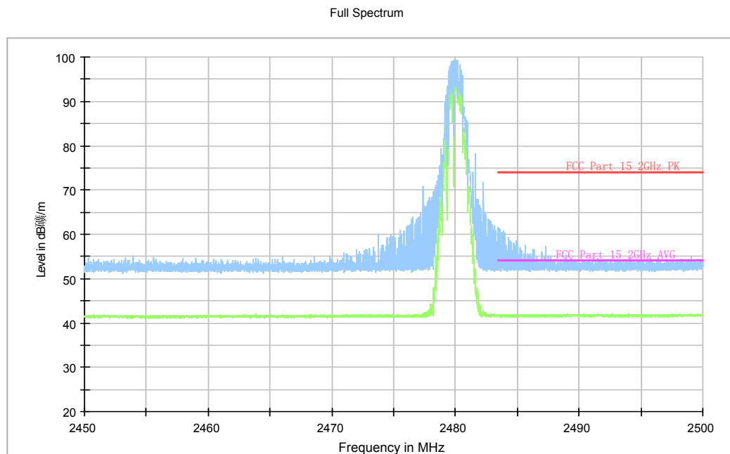
Fig.66. Radiated emission (Power) GFSK, high channel
