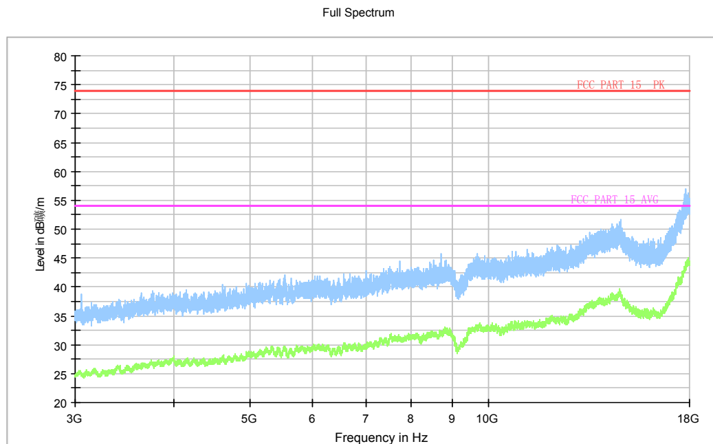
Fig.72. Radiated emission: \pi/4 DQPSK, Channel 39, 3 GHz - 18 GHz
