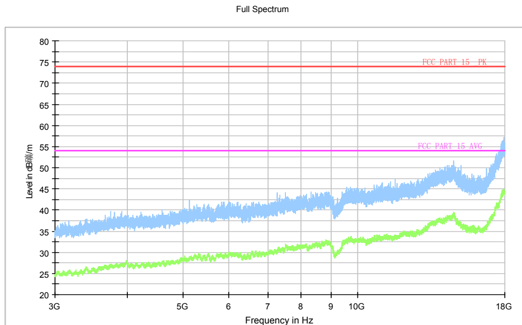
Fig.74. Radiated emission: \pi/4 DQPSK, Channel 78, 3 GHz - 18 GHz
