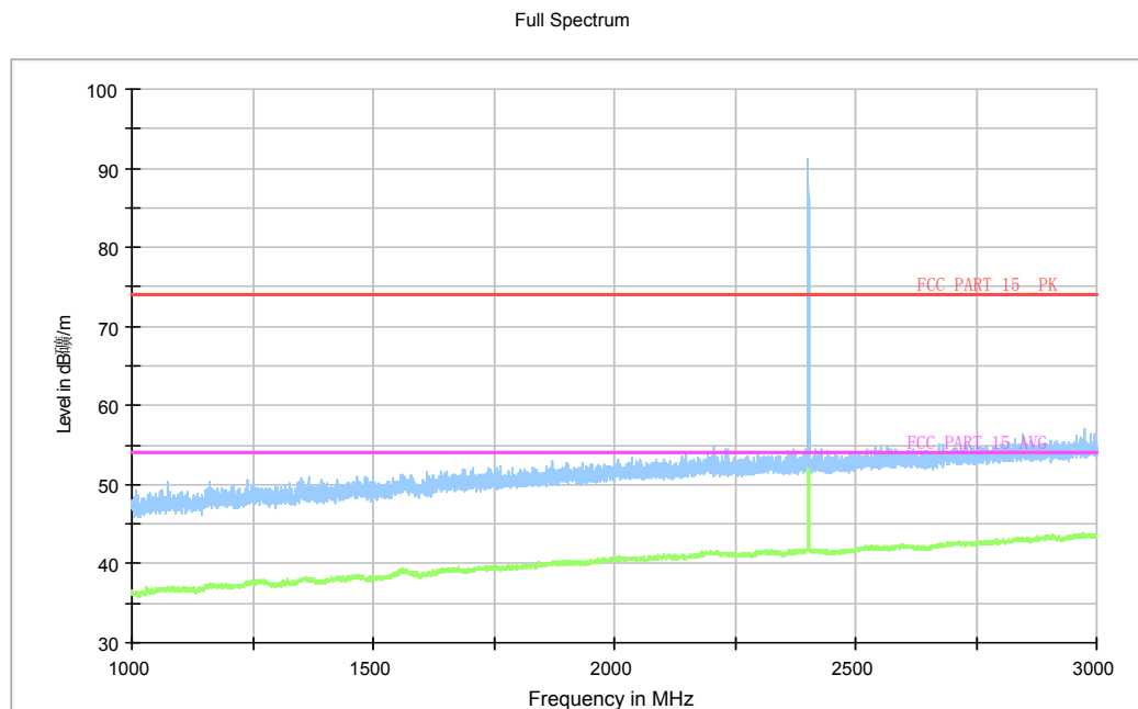
Fig.68. Radiated emission: \pi/4 DQPSK, Channel 0, 1 GHz - 3 GHz
