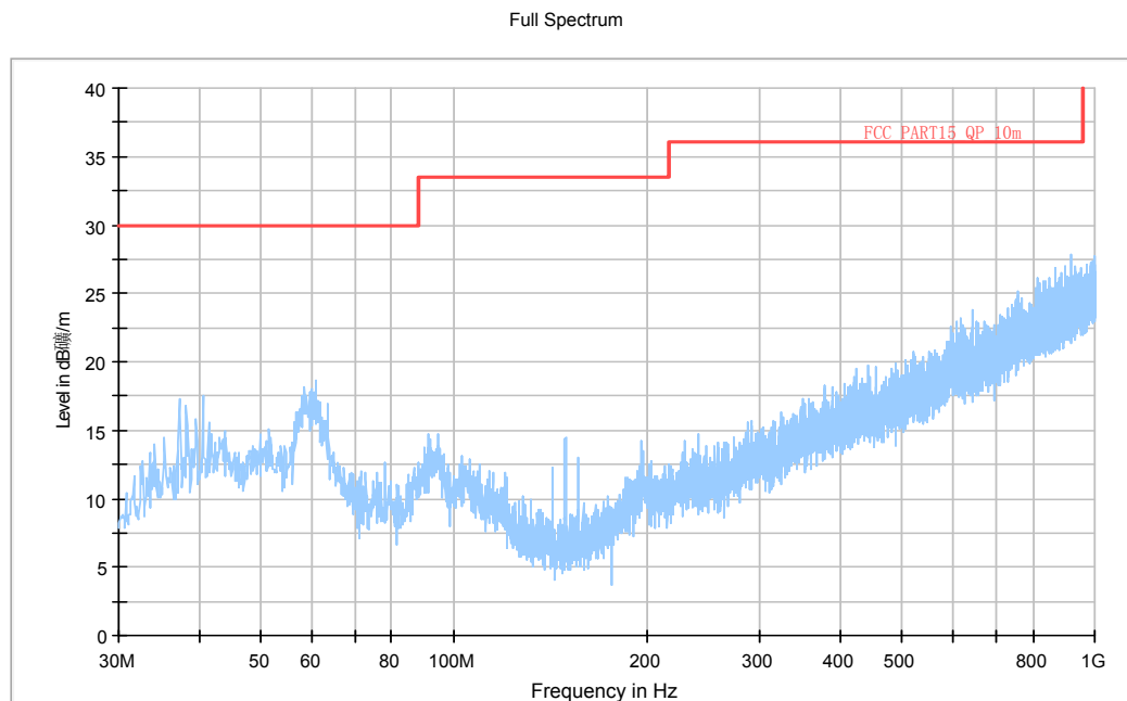
Fig.80. Radiated emission: 8DPSK, Channel 39, 30 MHz - 1 GHz
