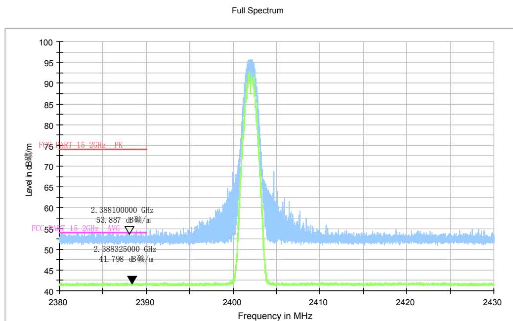
Fig.65. Radiated emission (Power): GFSK, low channel
