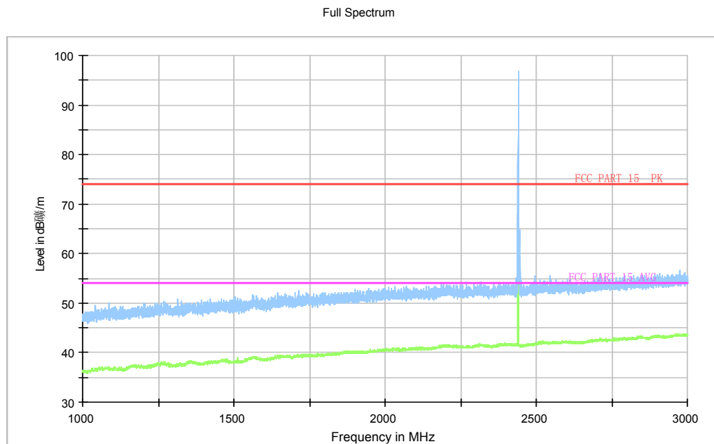
Fig.63. Radiated emission: GFSK, Channel 78, 1 GHz - 3 GHz
