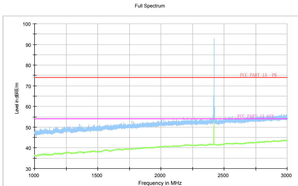
Fig.61. Radiated emission: GFSK, Channel 39, 1 GHz - 3 GHz
