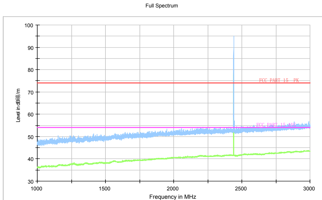
Fig.81. Radiated emission: 8DPSK, Channel 39, 1 GHz - 3 GHz
