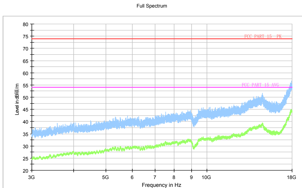
Fig.69. Radiated emission: \pi/4 DQPSK, Channel 0, 3 GHz - 18 GHz
