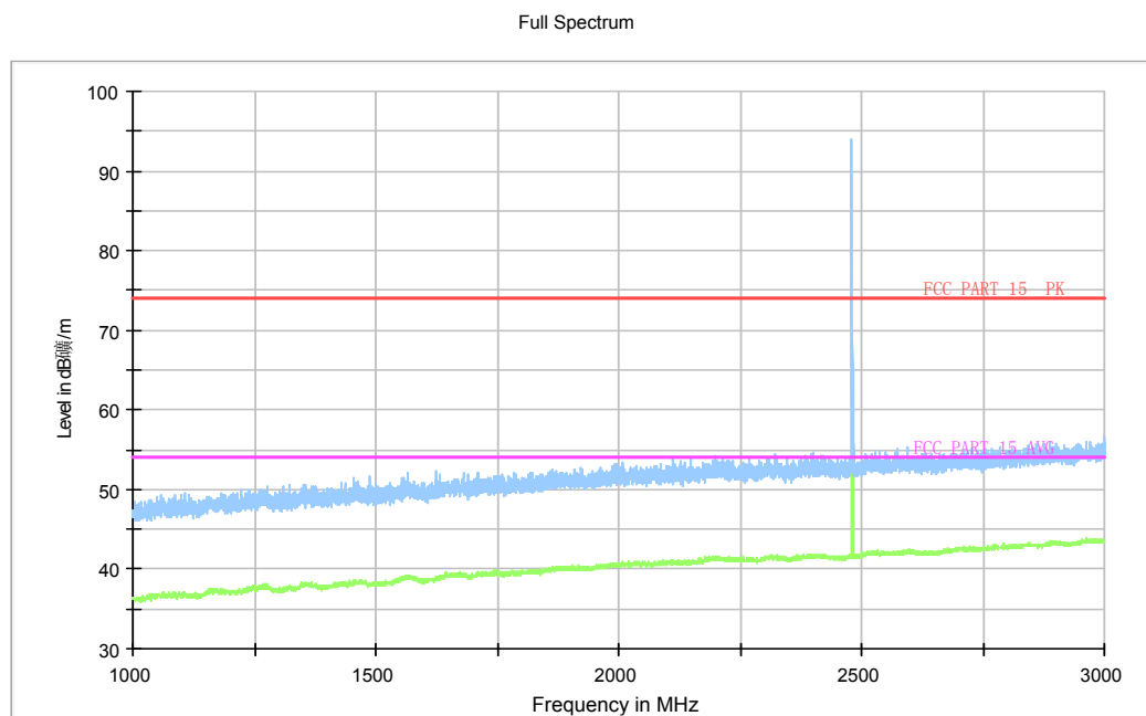
Fig.73. Radiated emission: \pi/4 DQPSK, Channel 78, 1 GHz - 3 GHz
