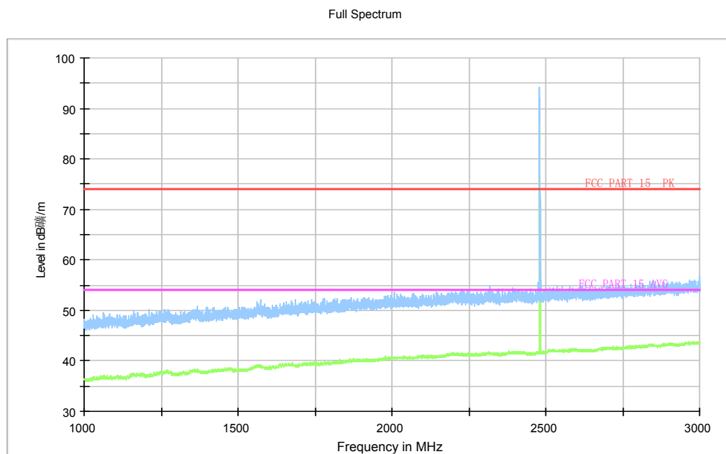
Fig.83. Radiated emission: 8DPSK, Channel 78, 1 GHz - 3 GHz
