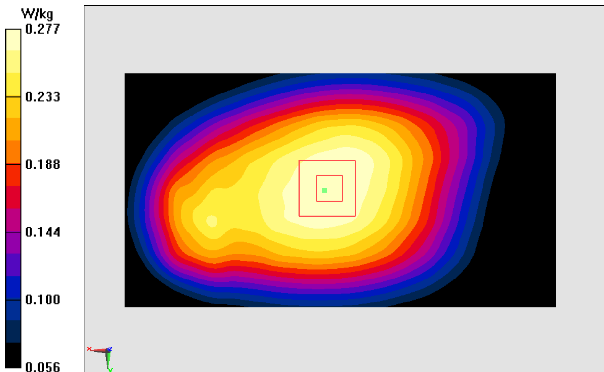
Fig.2 850 MHz
