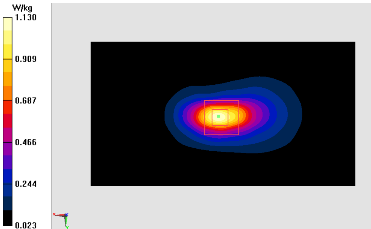
Fig.4 1900 MHz
