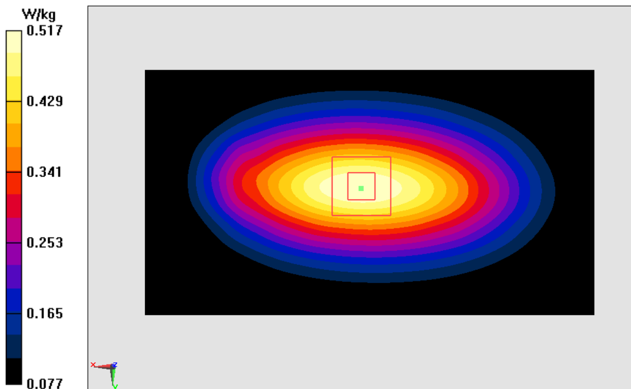
Fig.20 LTE Band12
