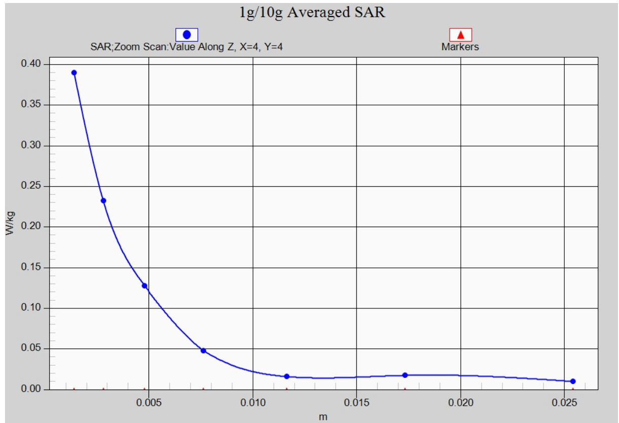
Fig. 24-1 Z-Scan at power reference point (5GHz)
