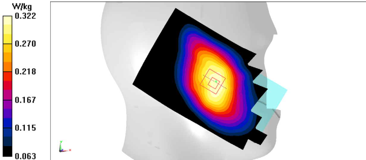
Fig.19 LTE Band12
