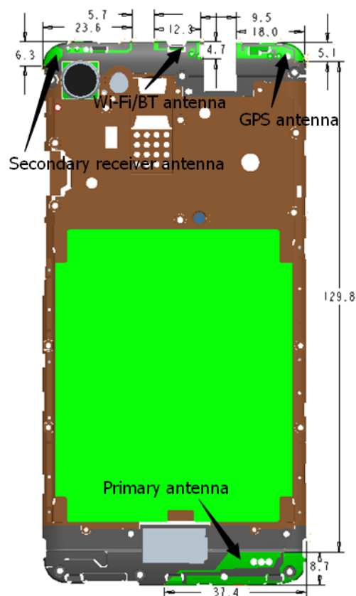
Picture 12.1 Antenna Locations
