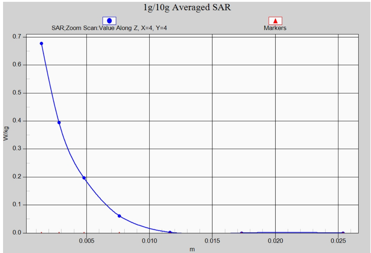
Fig. 23-1 Z-Scan at power reference point (5GHz)
