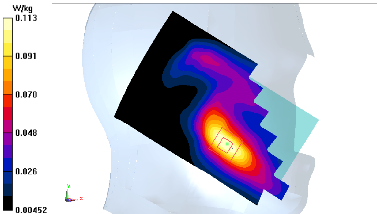
Fig.3 1900 MHz
