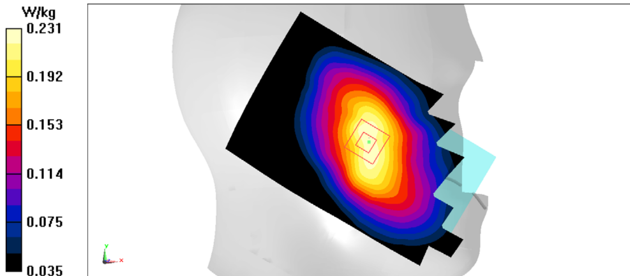
Fig.1 850MHz
