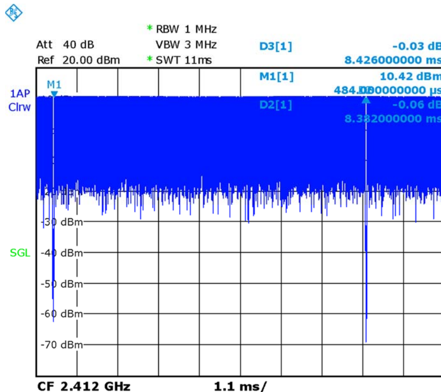
Picture 14.1 Duty factor plot (CH1)
