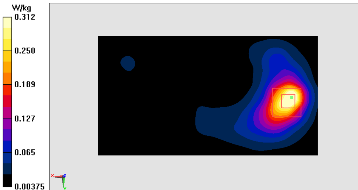
Fig.22 2450 MHz
