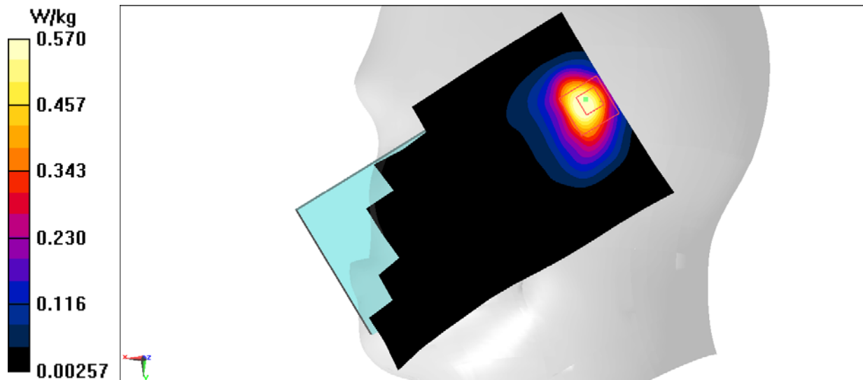
Fig.21 2450 MHz
