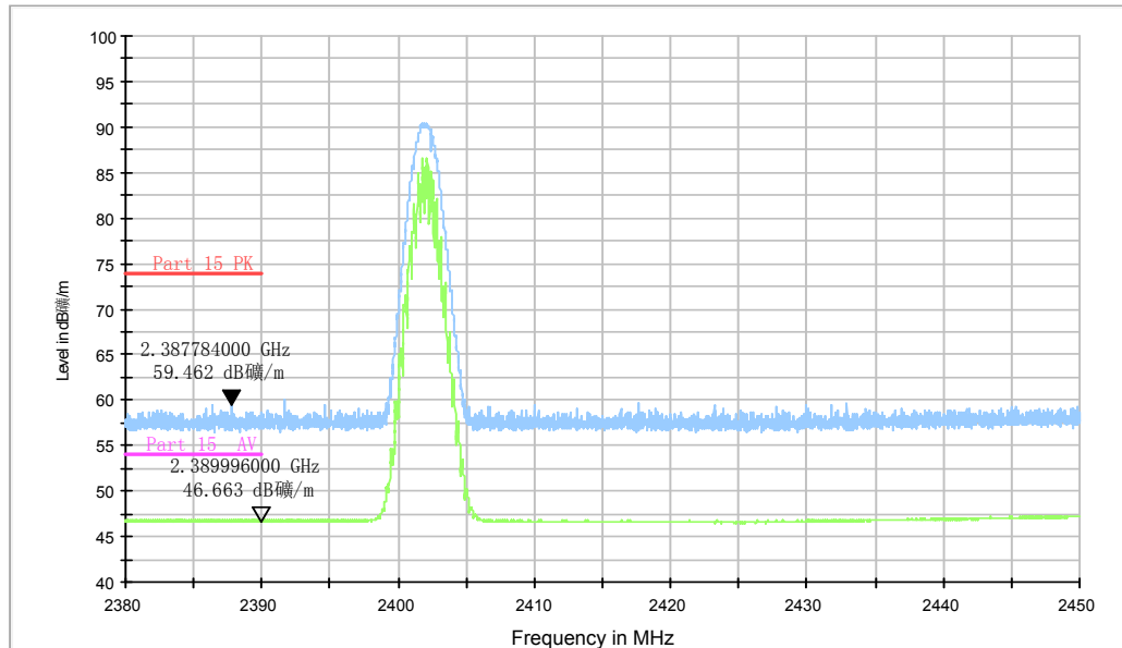
Fig.60. Radiated emission (Power): π/4 DQPSK, low channel
