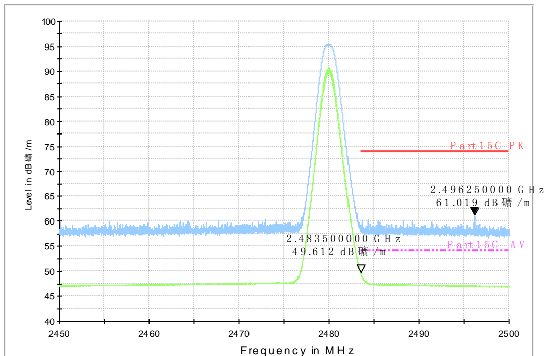
RE - Power-2.45GHz-2.5GHz
