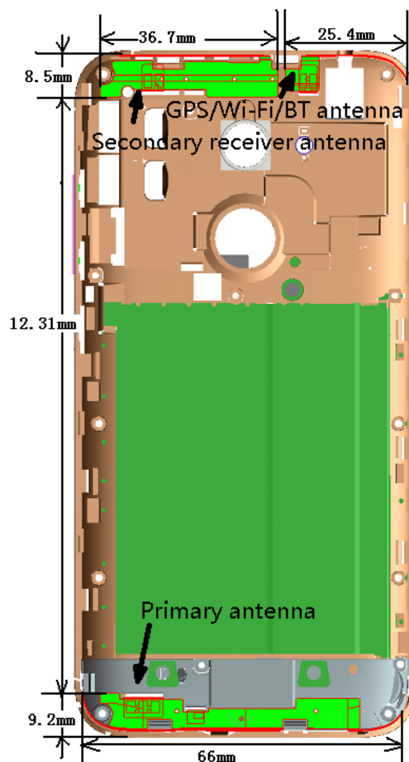
Picture 12.1 Antenna Locations
