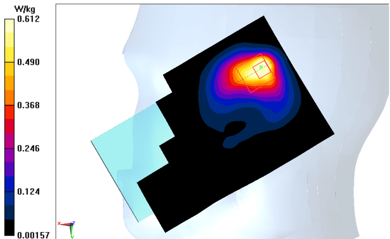
Fig.23 2450 MHz
