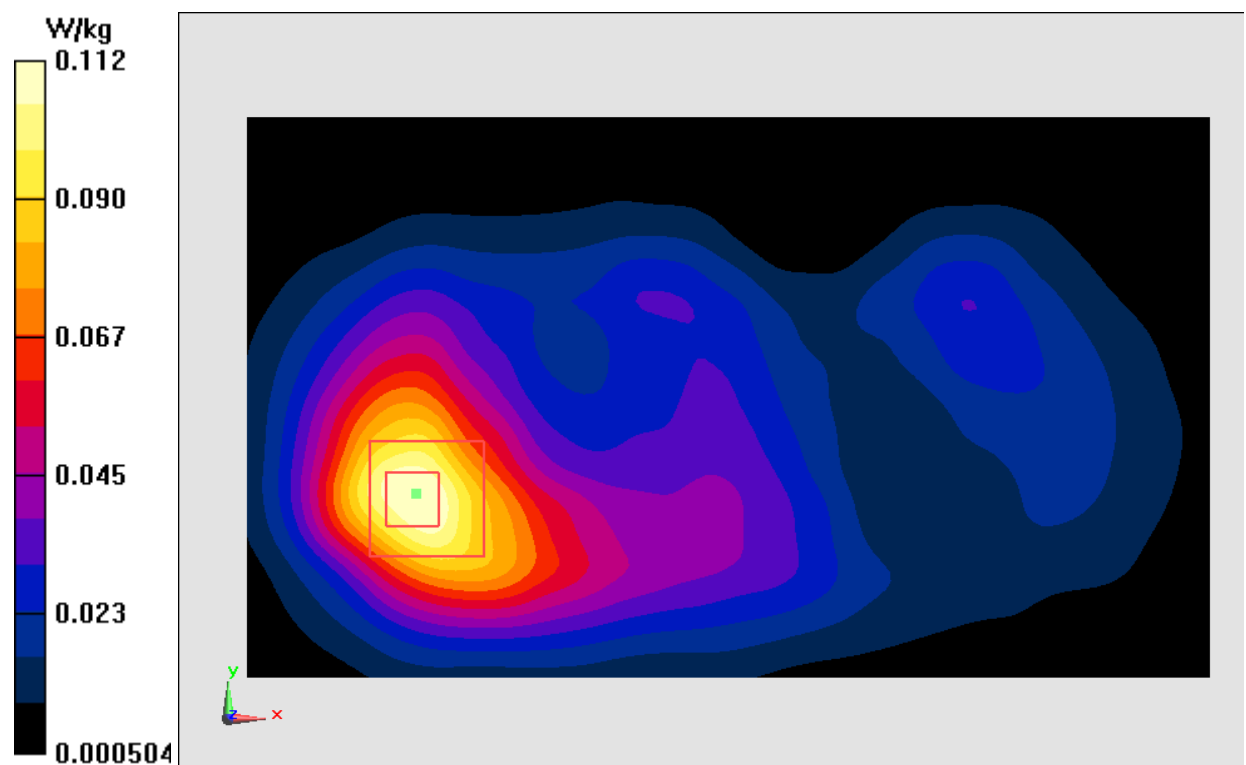
Fig.24 2450 MHz
