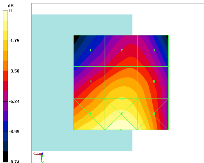
Fig B.1 HAC RF E-Field GSM 850 High
