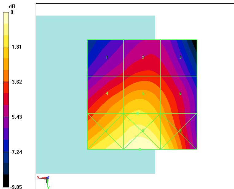
Fig B.2 HAC RF E-Field GSM 850 Middle
