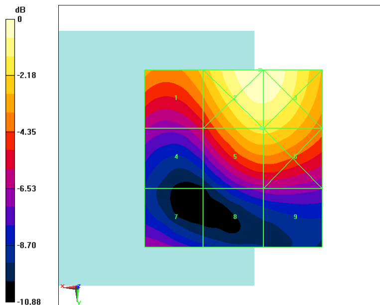
Fig B.5 HAC RF E-Field GSM 1900 Middle
