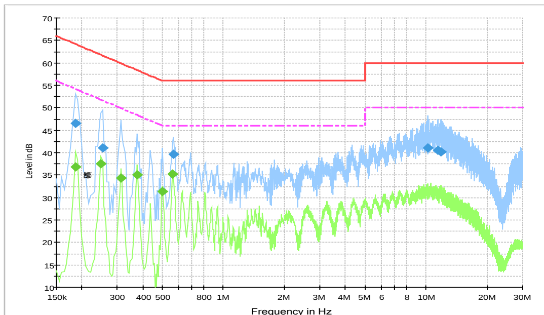
Fig.A.7.4 AC Powerline Conducted Emission-Idle(CBA0058AGAC3)
