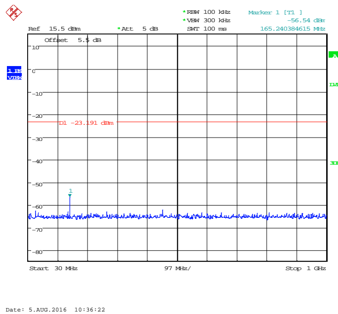
Fig.14. Transmitter Spurious Emission - Conducted: GFSK, 2480 MHz, 30MHz - 1GHz
