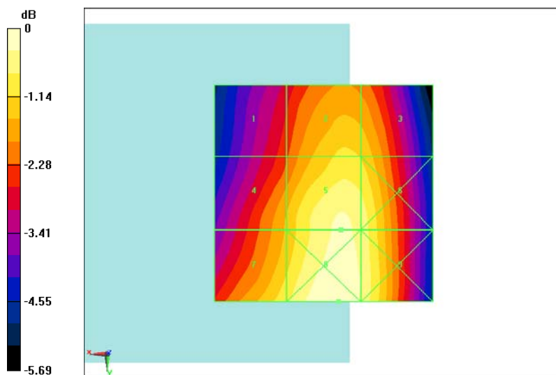
Fig B.2 HAC RF E-Field GSM 850 Middle
