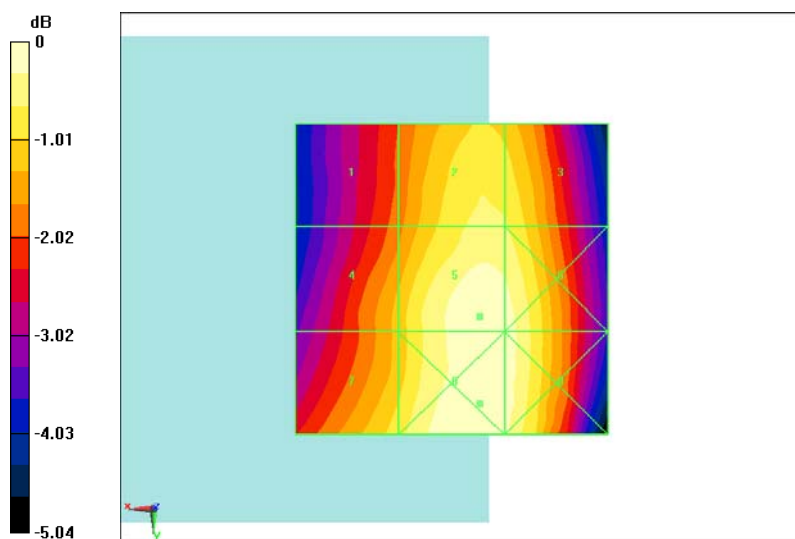
Fig B.1 HAC RF E-Field GSM 850 High
