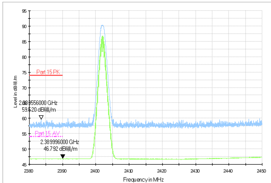
Fig.66. Radiated emission (Power): GFSK, low channel
