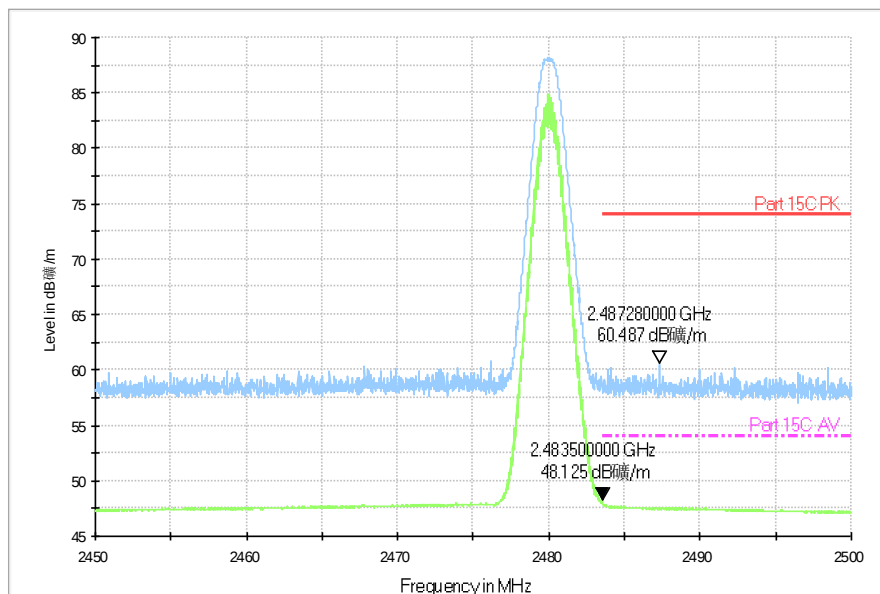
Fig.67. Radiated emission (Power) GFSK, high channel
