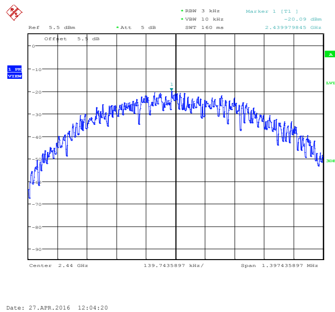
Fig.33. Maximum Power Spectral Density Level Function: GFSK, 2440 MHz
