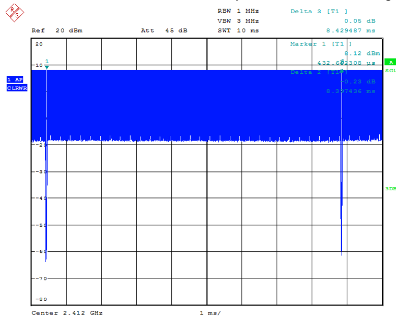
Picture 14.1 The plot of duty factor for WLAN-2.4G
